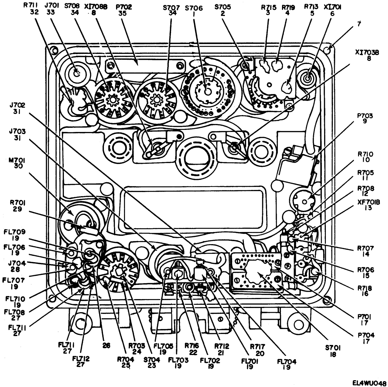
Figure 30. Receiver-Transmitters RT-441/TRC-68 and RT-441A/TRC-68 Front Panel, Rear View.
