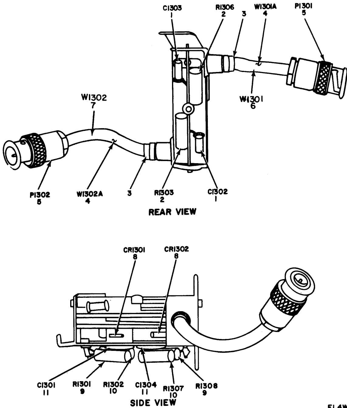
Figure 38. Coupler, Directional.
