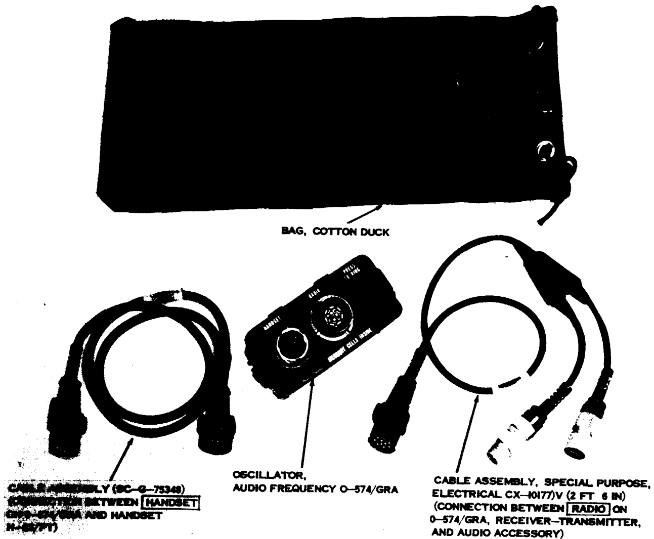
A. OSCILLATOR, AUDIO FREQUENCY 0-574/GRC.
