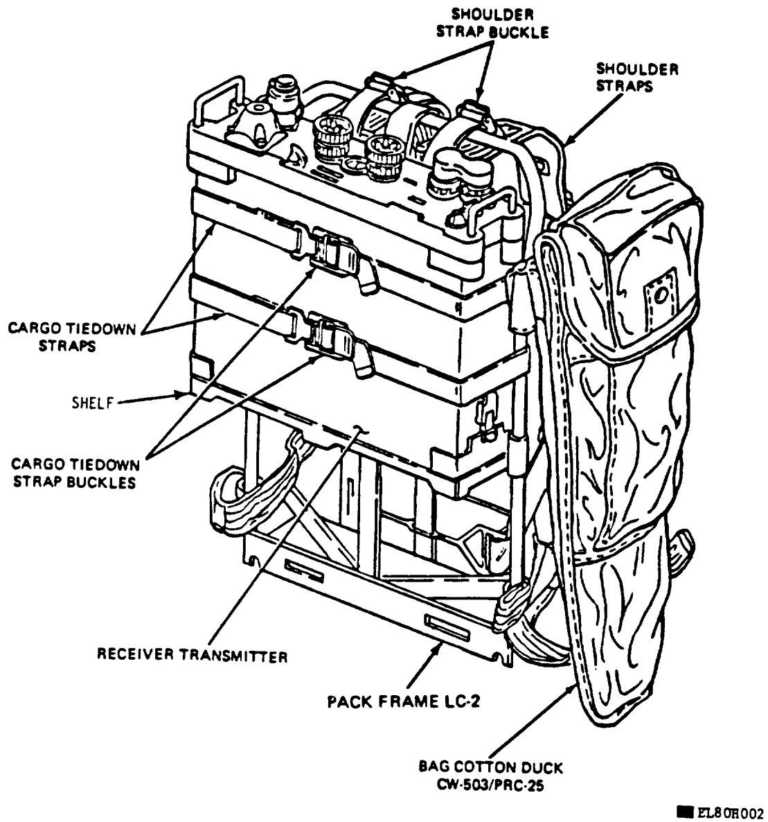
Figure 2-4. Installation of Receiver-Transmitter in LC-2 for man-pack operation.
