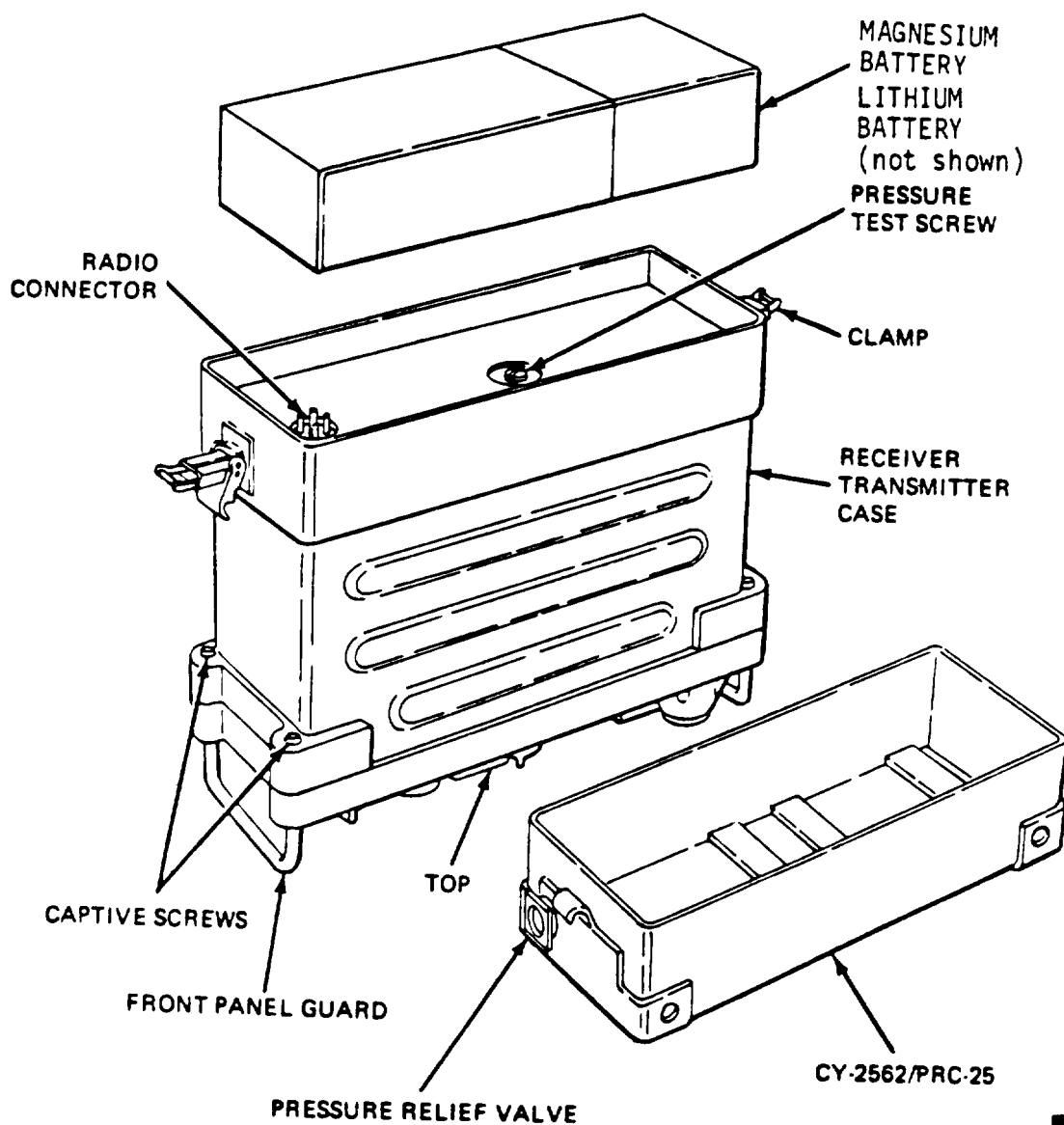
■ Figure 2-6. Installing battery in receiver-transmitter.
