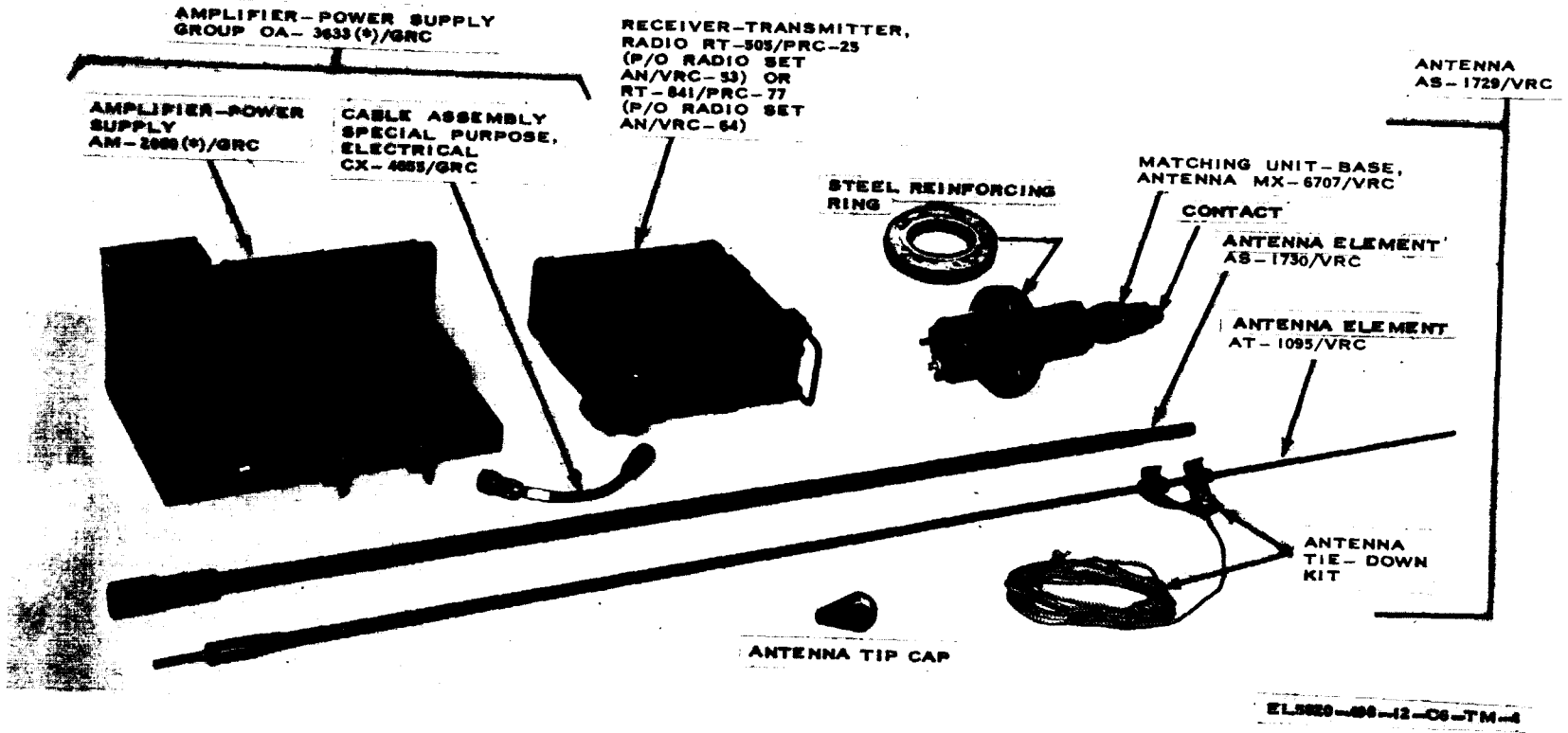
Figure 1-10. Components of AN/VRC-53 and AN/VRC-64.
