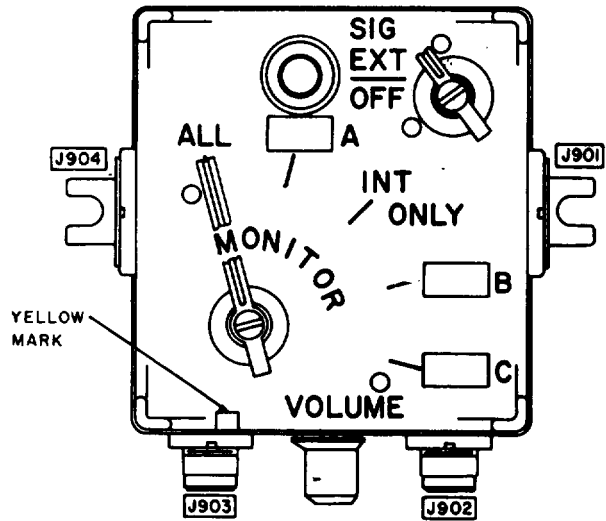
Figure 3-4. Control, Intercommunication Set C-2297/VRC, controls, indicator, and connectors.
