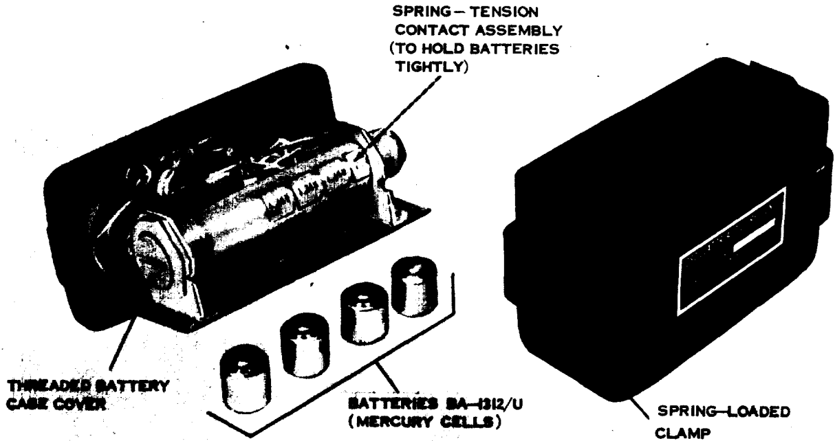
B. OSCILLATOR, AUDIO FREQUENCY 0-574/GRA WITH BATTERIES. (LESS CABLES AND BAG)
