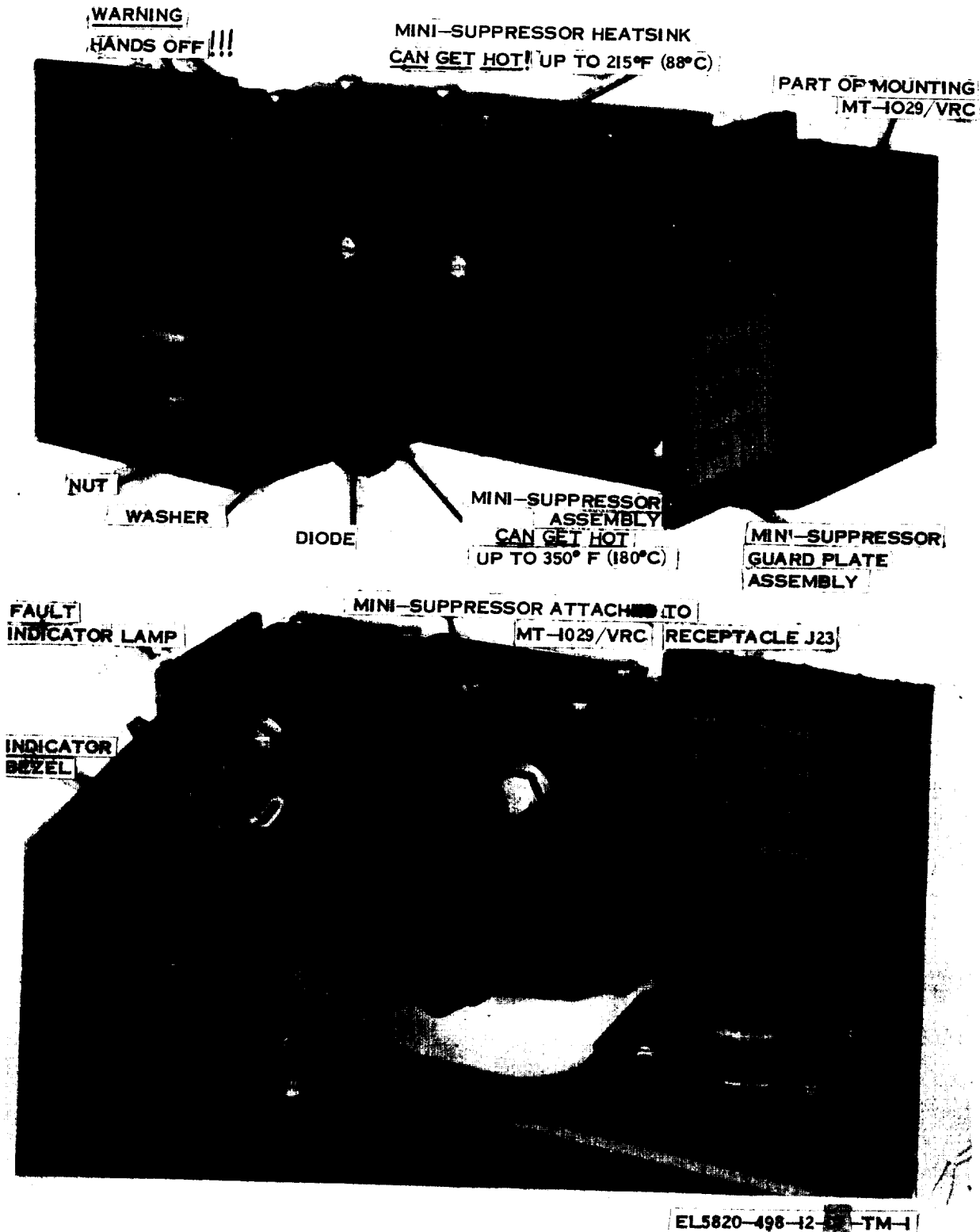
Figure 2-8. Mini-suppressor installed on MT-1029/VRC in some tank installation harnesses.
