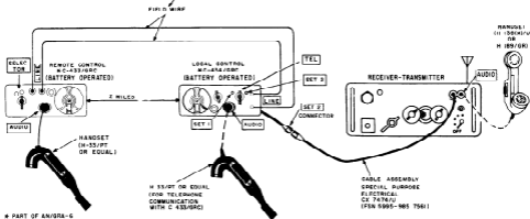
A REMOTE CONTROL CONNECTIONS
