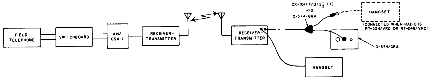
C. AN/GSA-7 AT ONE STATION, O-574/GRA AT OTHER; NO RADIO OPERATOR REQUIRED.
