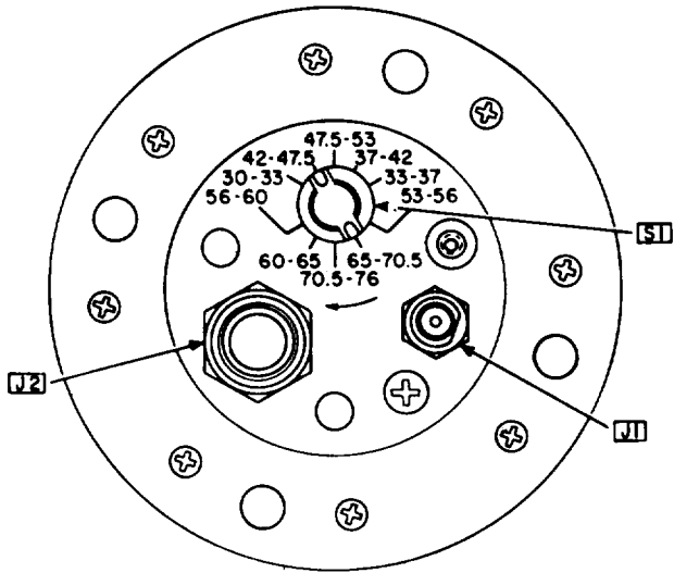
Figure 3-3. Antenna AS-1729/VRC, control and connectors.
