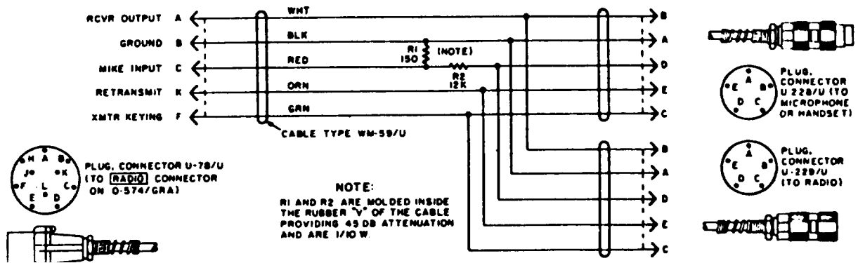
C. CABLE ASSEMBLY SPECIAL PURPOSE ELECTRICAL CX10177/U 12 FT, 6 IN).
