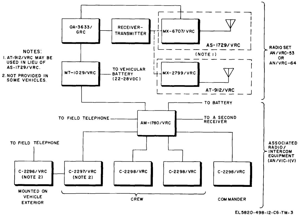
Figure 1-4. Radio Sets AN/VRC-53 and AN/VRC-64 typical configuration with radio/intercom equipment.
