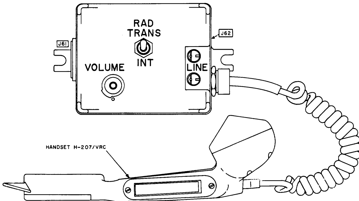
Figure 3-6. Control, Intercommunication Set C-2296/VRC, controls and connectors.
