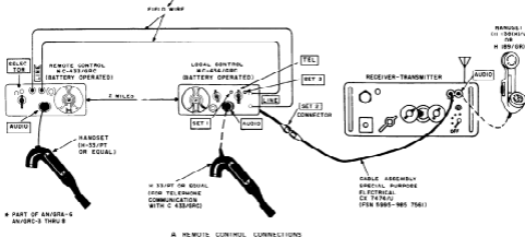
A REMOTE CONTROL CONNECTIONS
