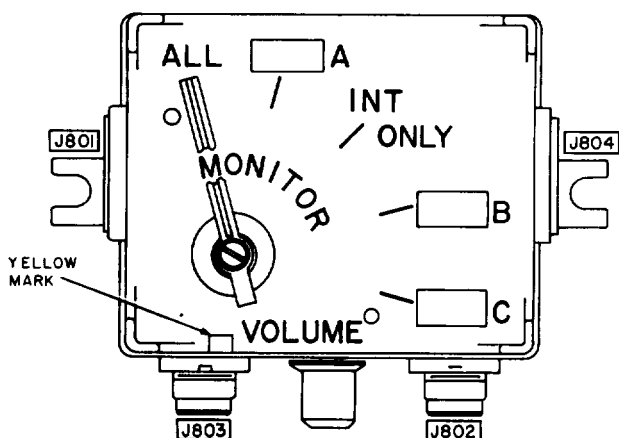
Figure 3-5. Control, Intercommunication Set C-2298/VRC, controls and connectors
