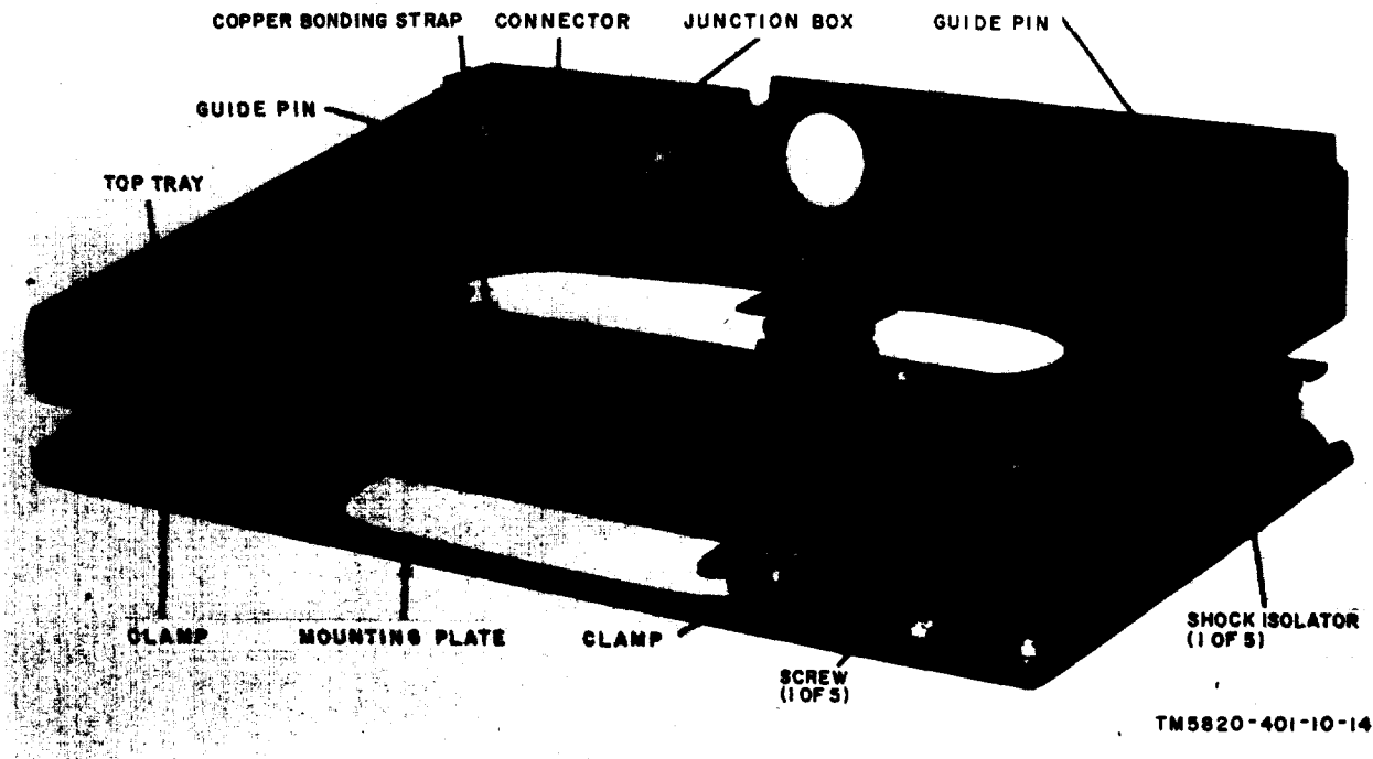
Figure 1-8. Mounting MT-1029/VRC.
