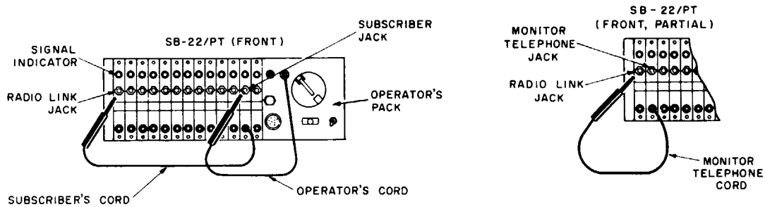
C. CORD CONNECTION FOR MONITOR TELEPHONE (NOTE 2).
