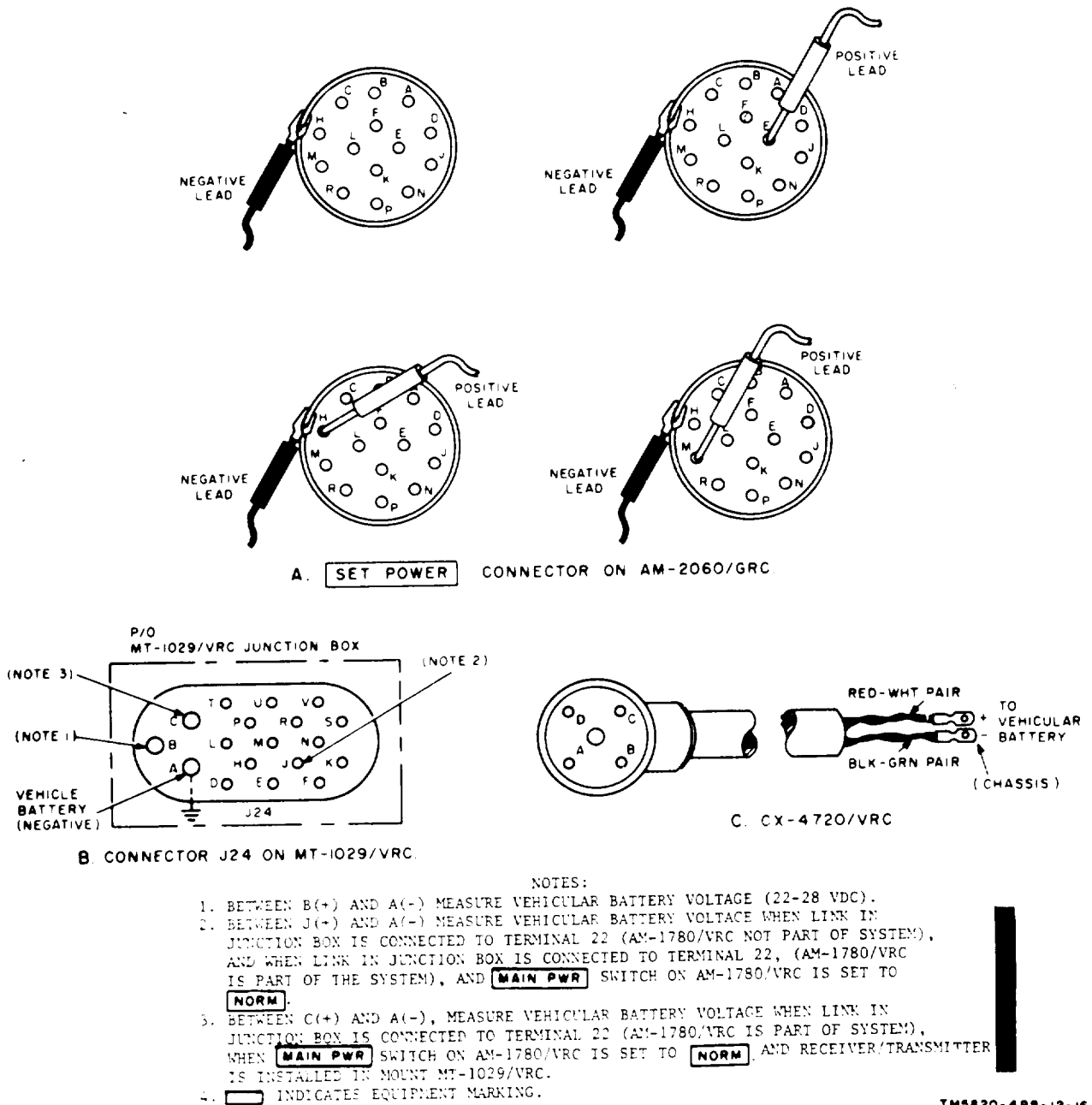
Figure 5-1. Output voltage test points on SET POWER connector on amplifier-power supply, J24 on MT-1029/VRC, and CX-4720/VRC.
