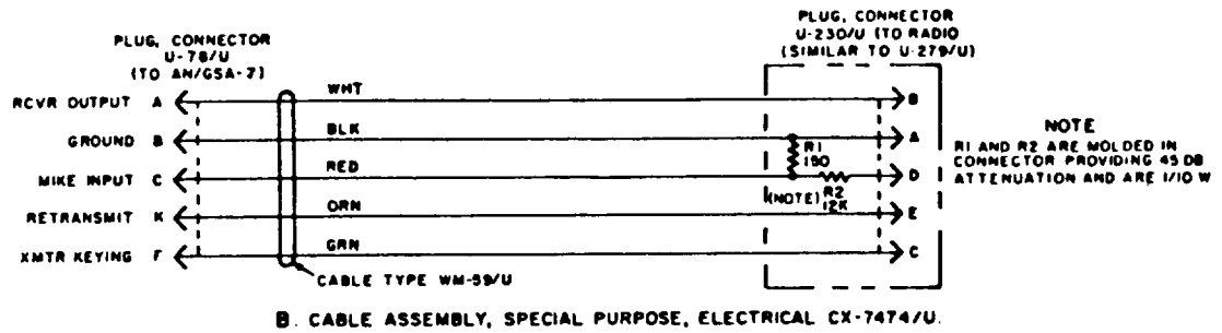
B. CABLE ASSEMBLY, SPECIAL PURPOSE, ELECTRICAL CX-7474/U.
