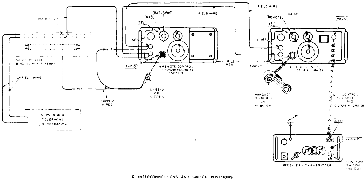
A INTERCONNECTIONS AND SWITCH POSITIONS
