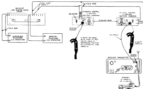
B RWI CONNECTIONS
