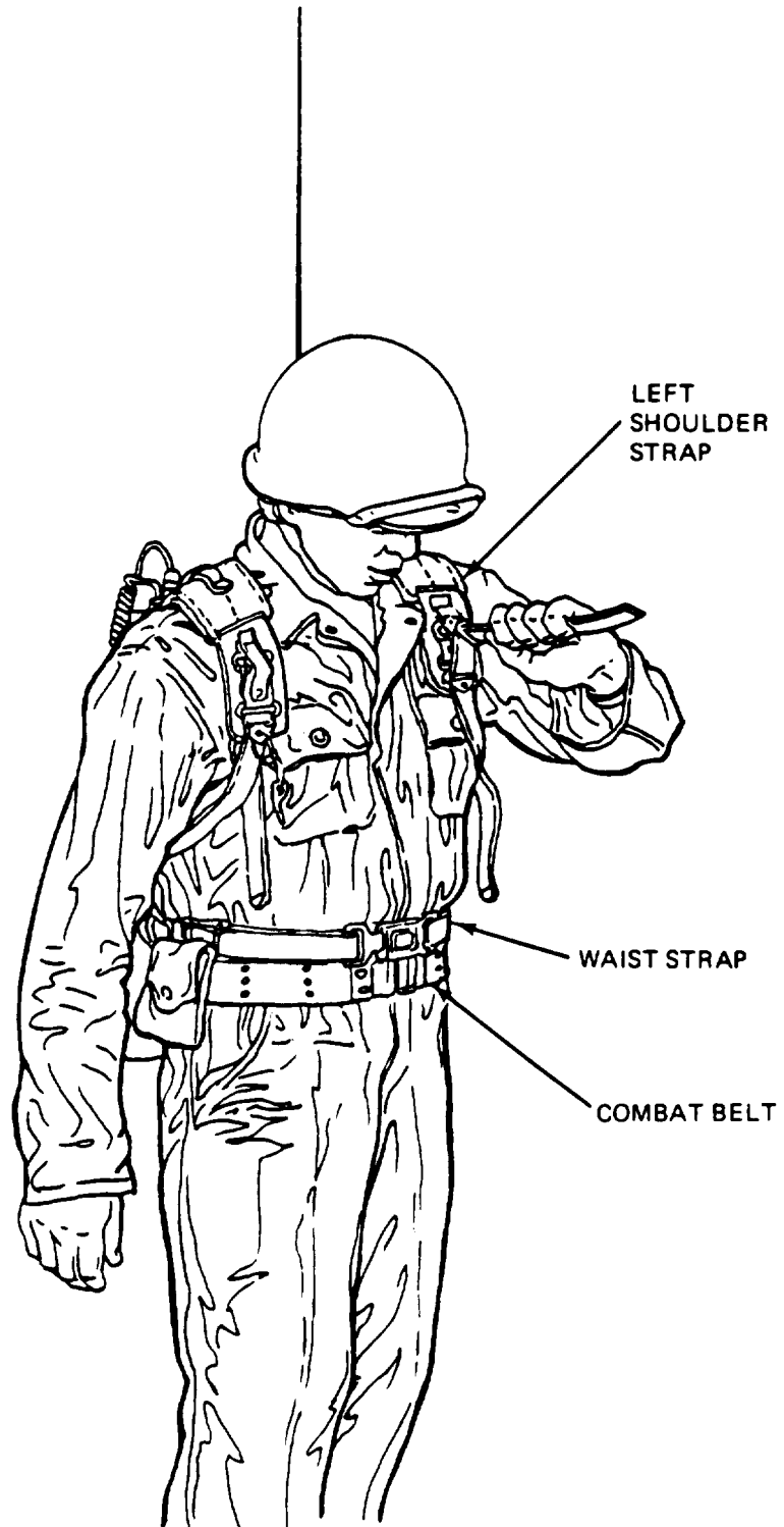
■ Figure 2-5 Strap arrangement of Pack Frame LC-2 for Man-pack Operation.
