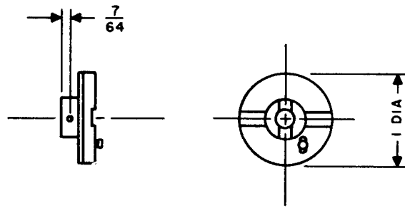
Figure 105. Torque meter adapter.
