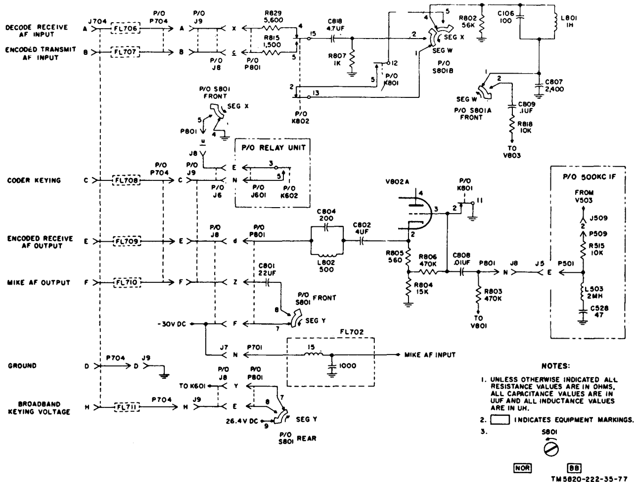
Figure 36. Broadband operation, schematic diagram.
