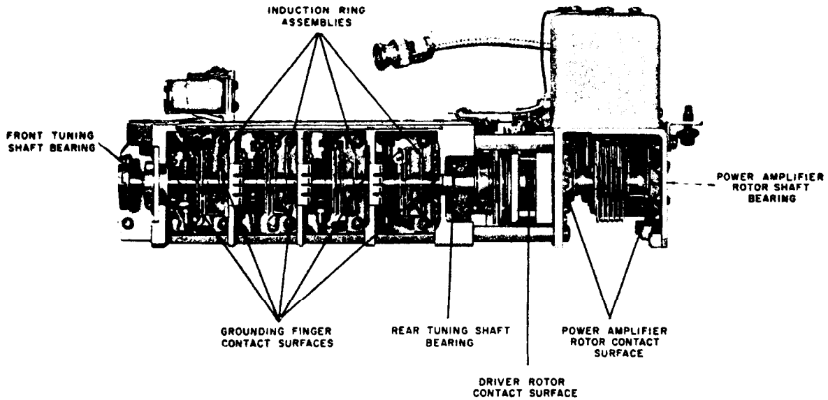
Figure 107. Rf and power amplifier subunit, lubrication points.
