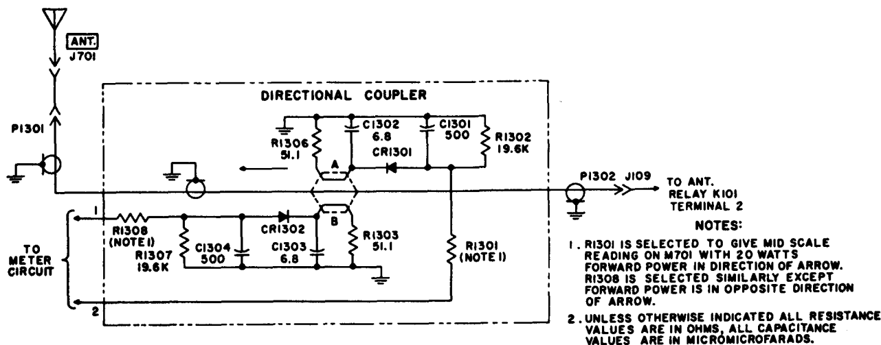
Figure 4. Directional coupler, schematic diagram.
