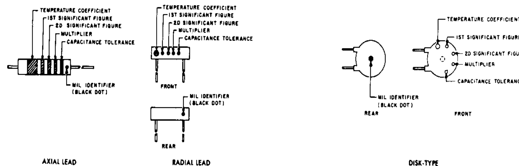
Figure 121. Color code marking for military standard capacitors.
