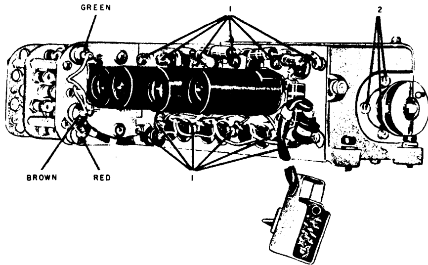
Figure 93. Uhf injection subunit, upper-front view, first oscillator cover plate removed.
