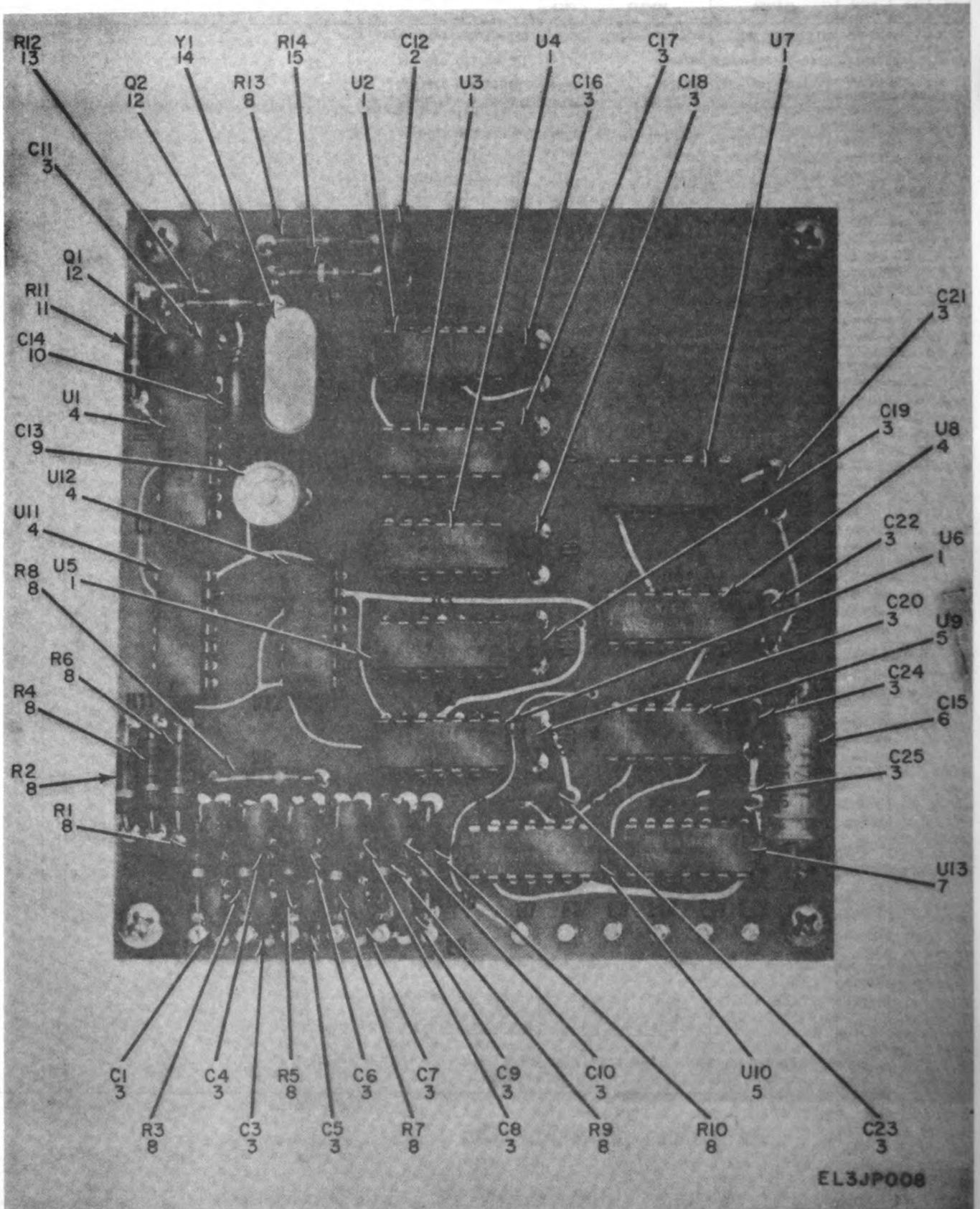
Figure 6. Generator, Signal SG-479C/GRM-50, Time Base A4.
