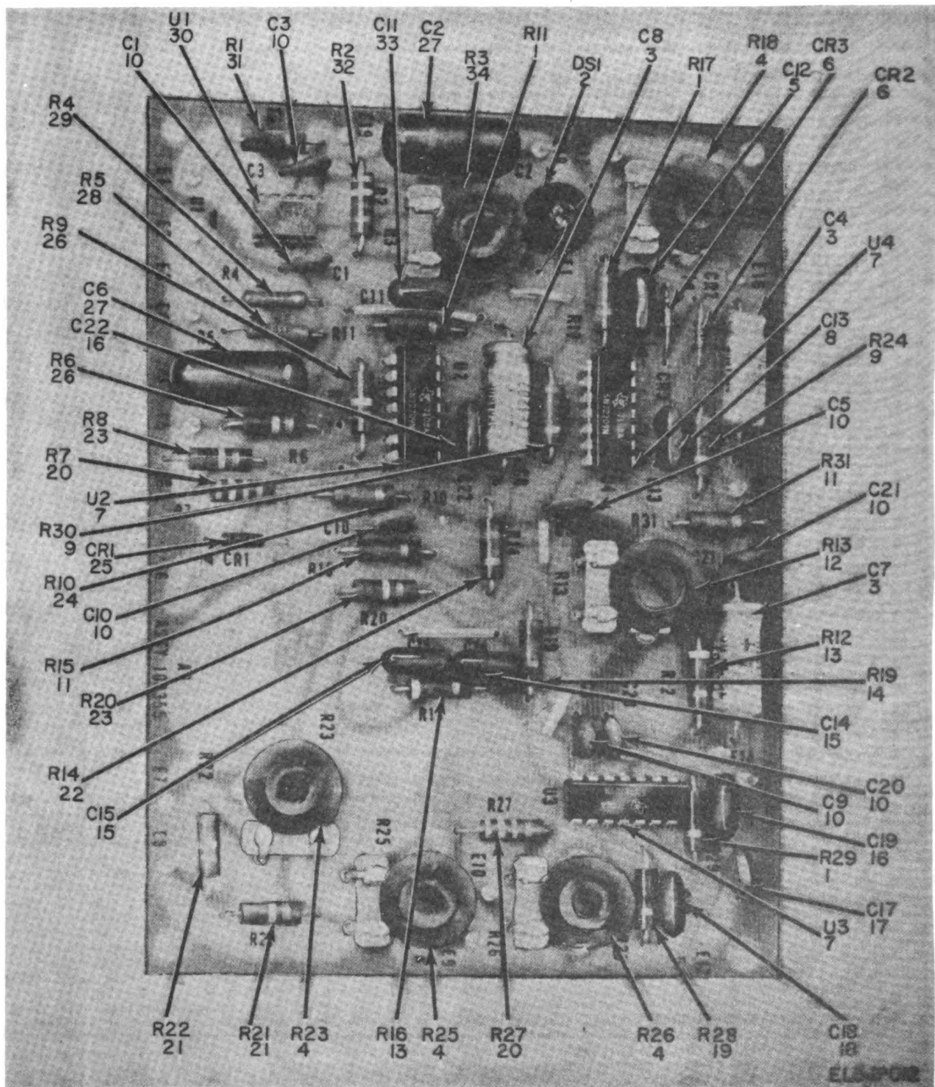
Figure 10. Generator, Signal SG-479C/GRM-50, Audio Level A9.
