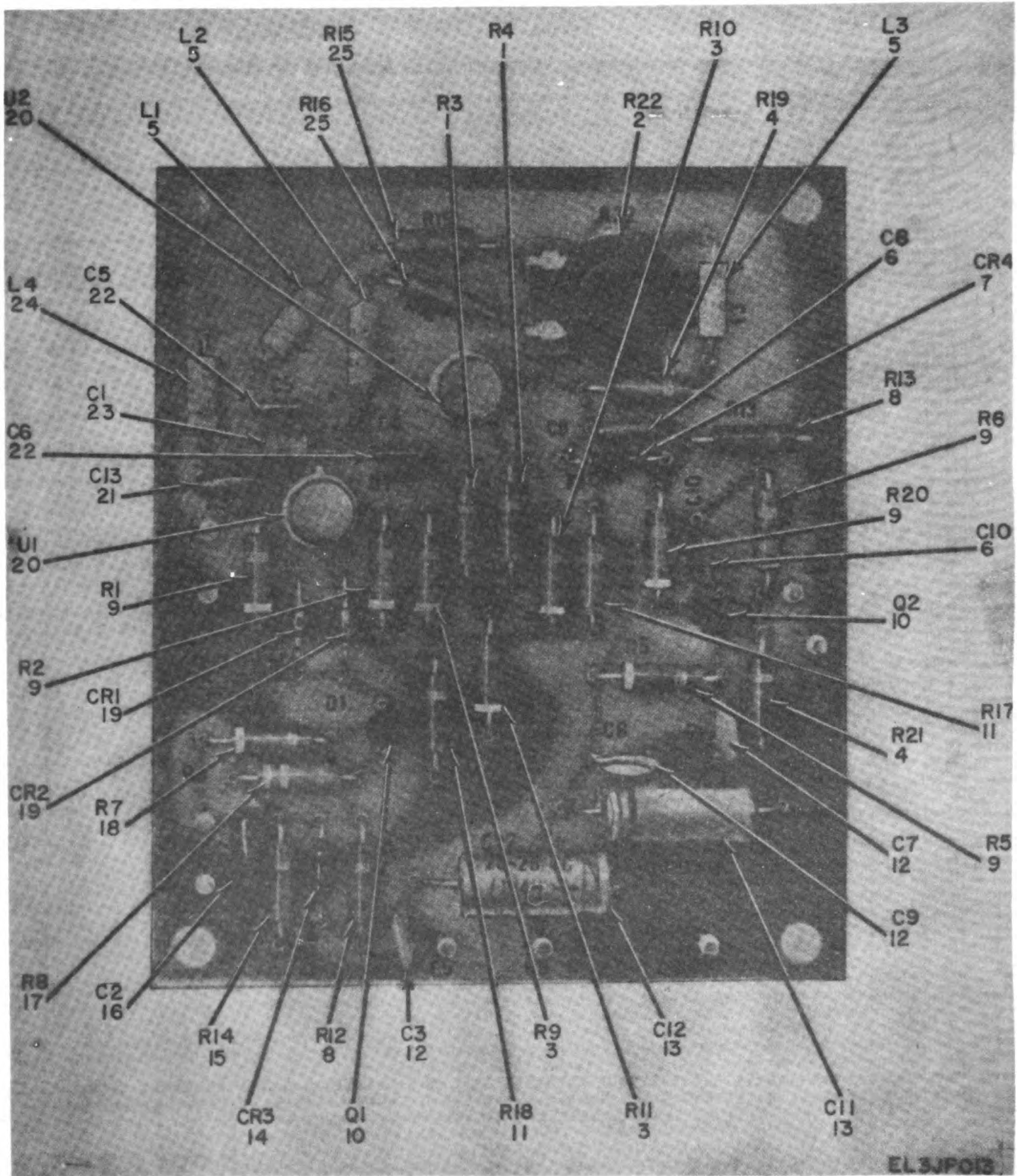
Figure 11. Generator, Signal SG-479C/GRM-50, Modulator A11.
