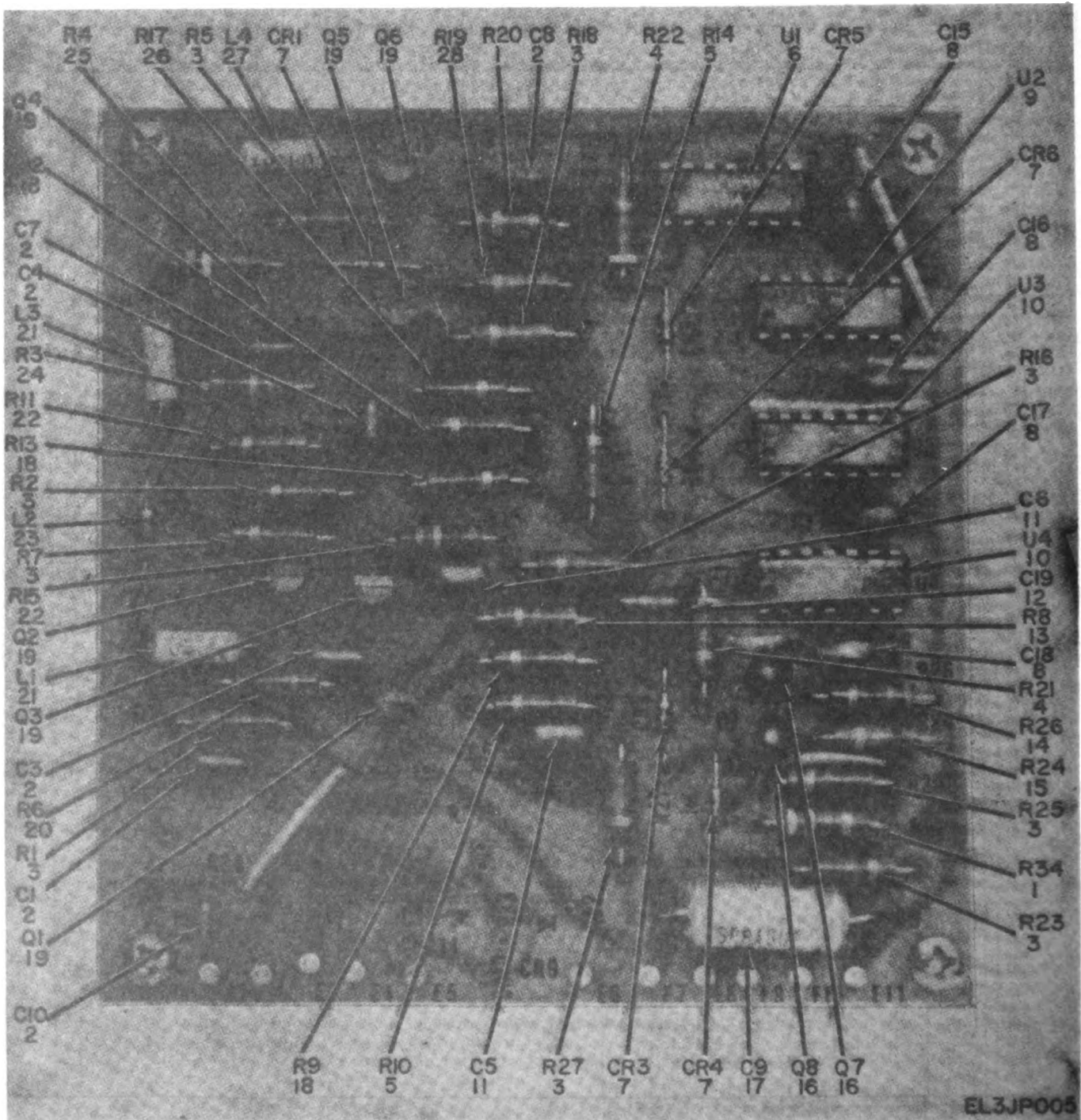
Figure 3. Generator, Signal SG-479C/GRM-50, Prescaler A1.
