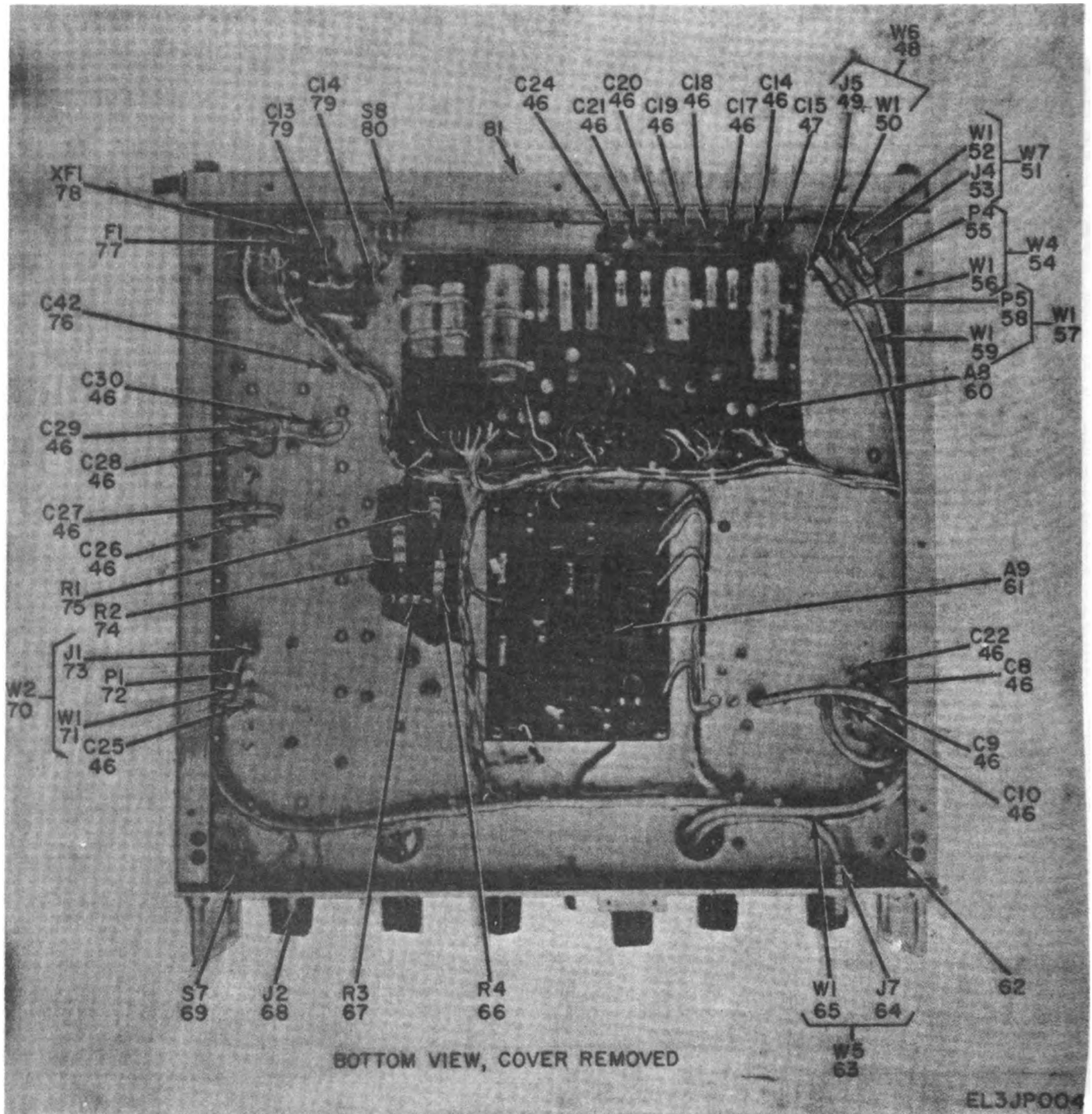
Figure 2. Generator, Signal SG-479C/GRM-50 (Sheet 3 of 3).
