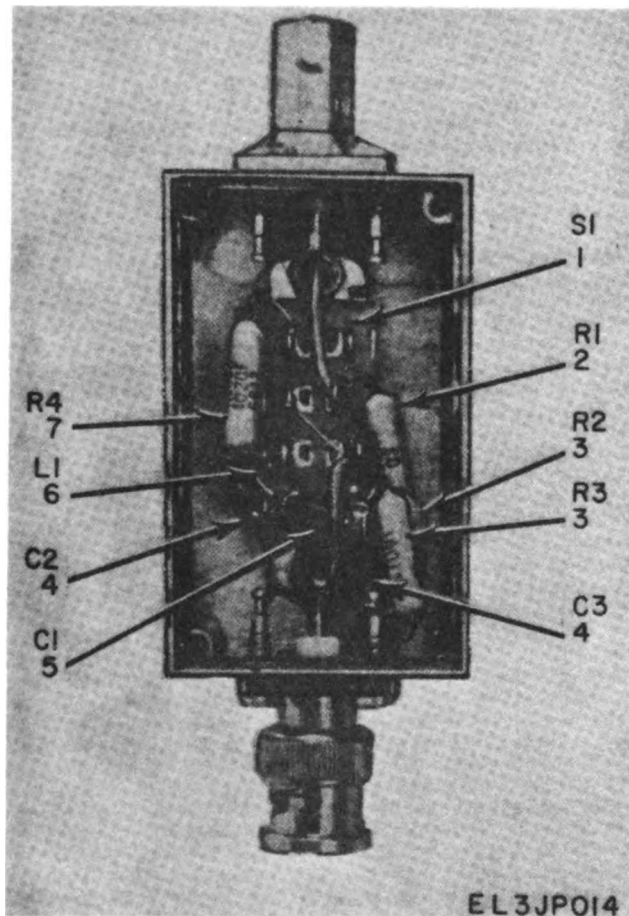
Figure 12. Dummy Load, DA-296A/GRM-50.
