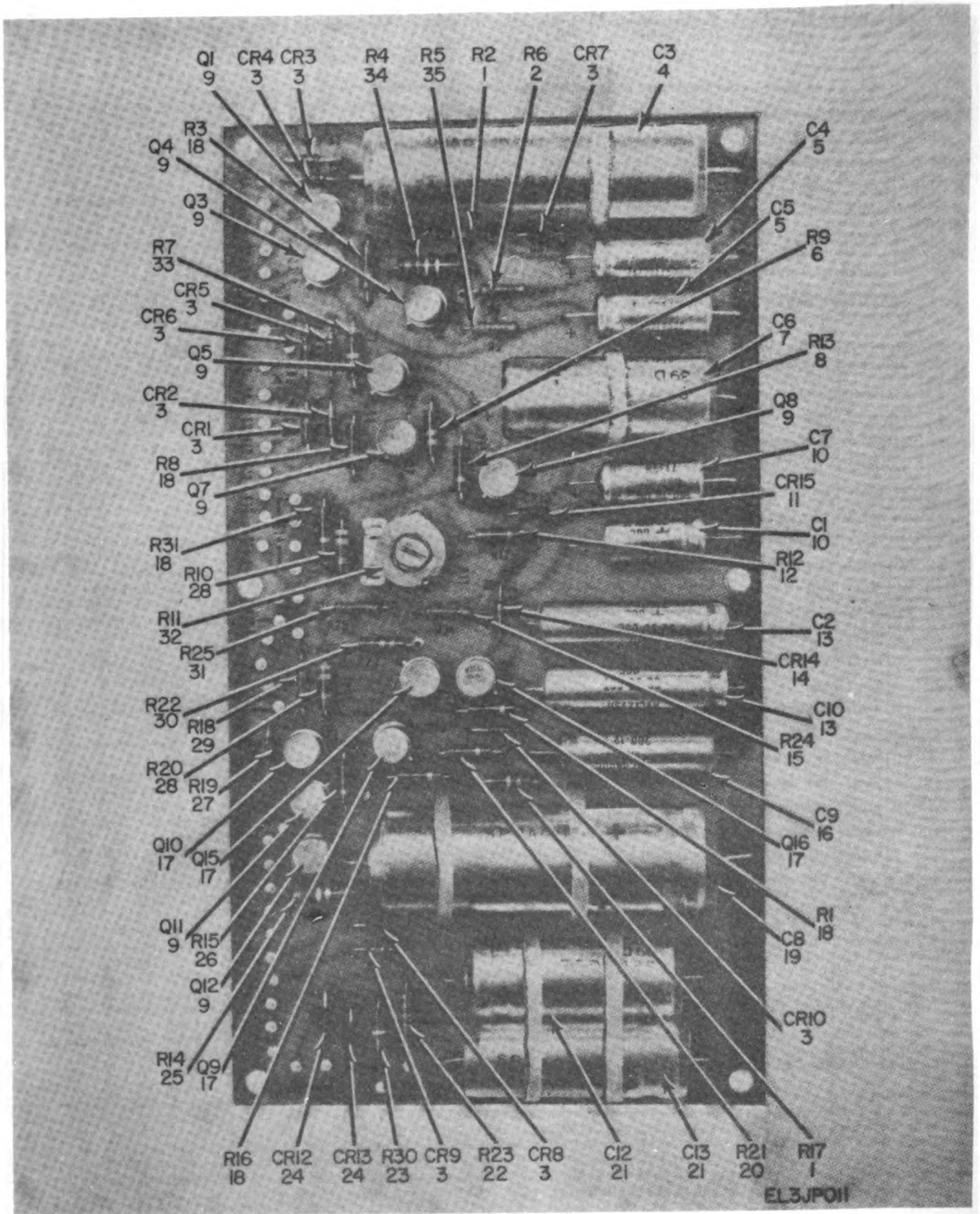
Figure 9. Generator, Signal SG-479C/GRM-50, Power Supply A8.
