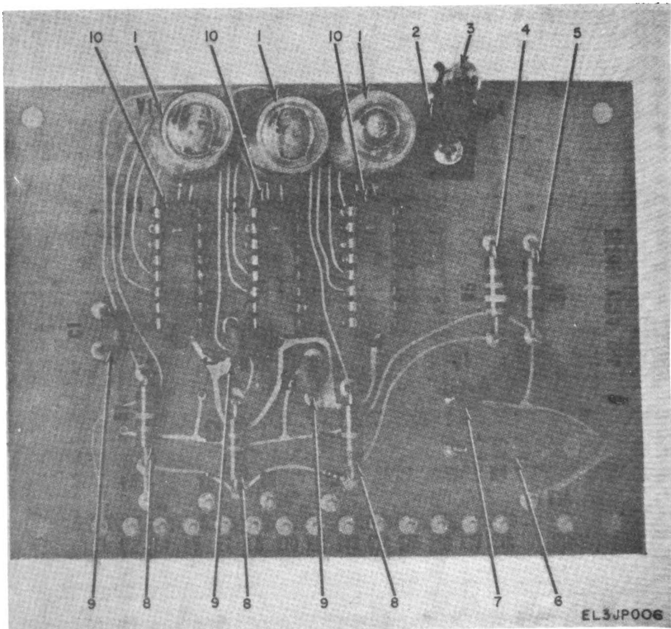
Figure 4. Generator, Signal SG-479C/GRM-50, Display A2.
