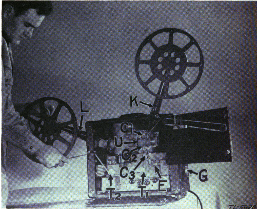
FIGURE 17.—Bell & Howell projector with film threaded.
