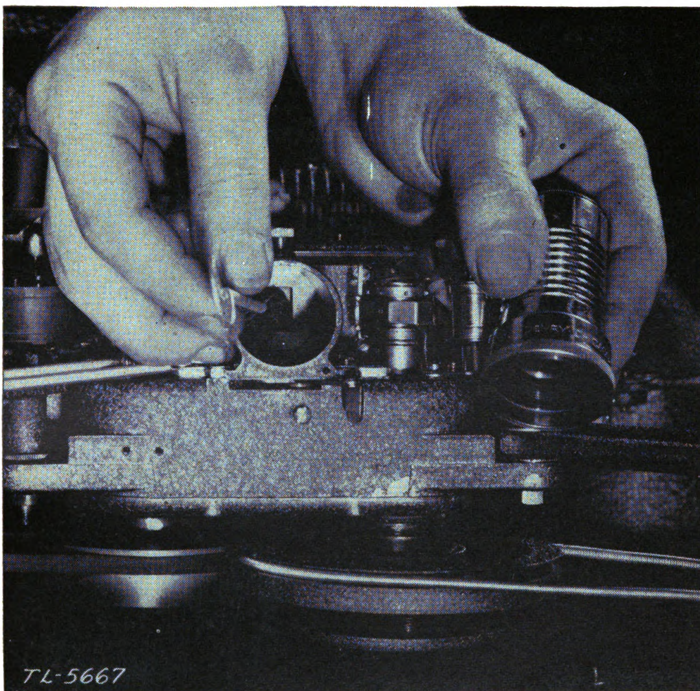
FIGURE 55.—Cleaning the aperture.
