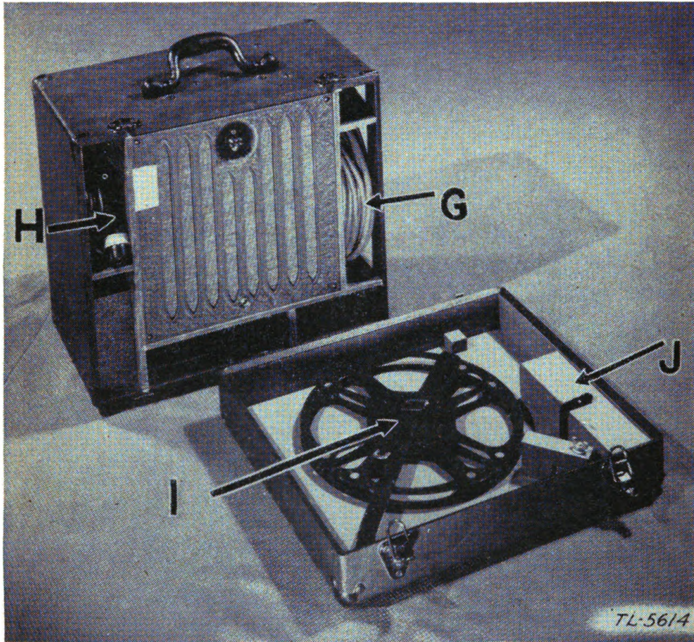
FIGURE 3.—Bell & Howell speaker case open.
