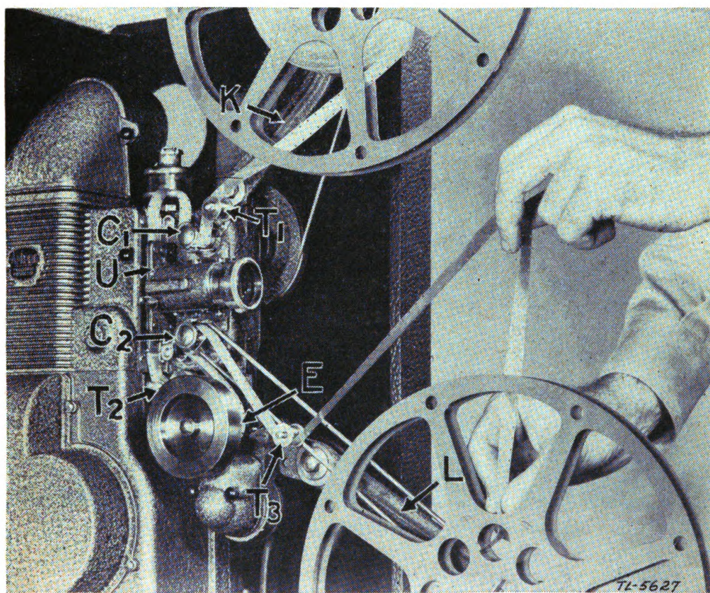
FIGURE 16.—Phonofilm projector with film threaded.
