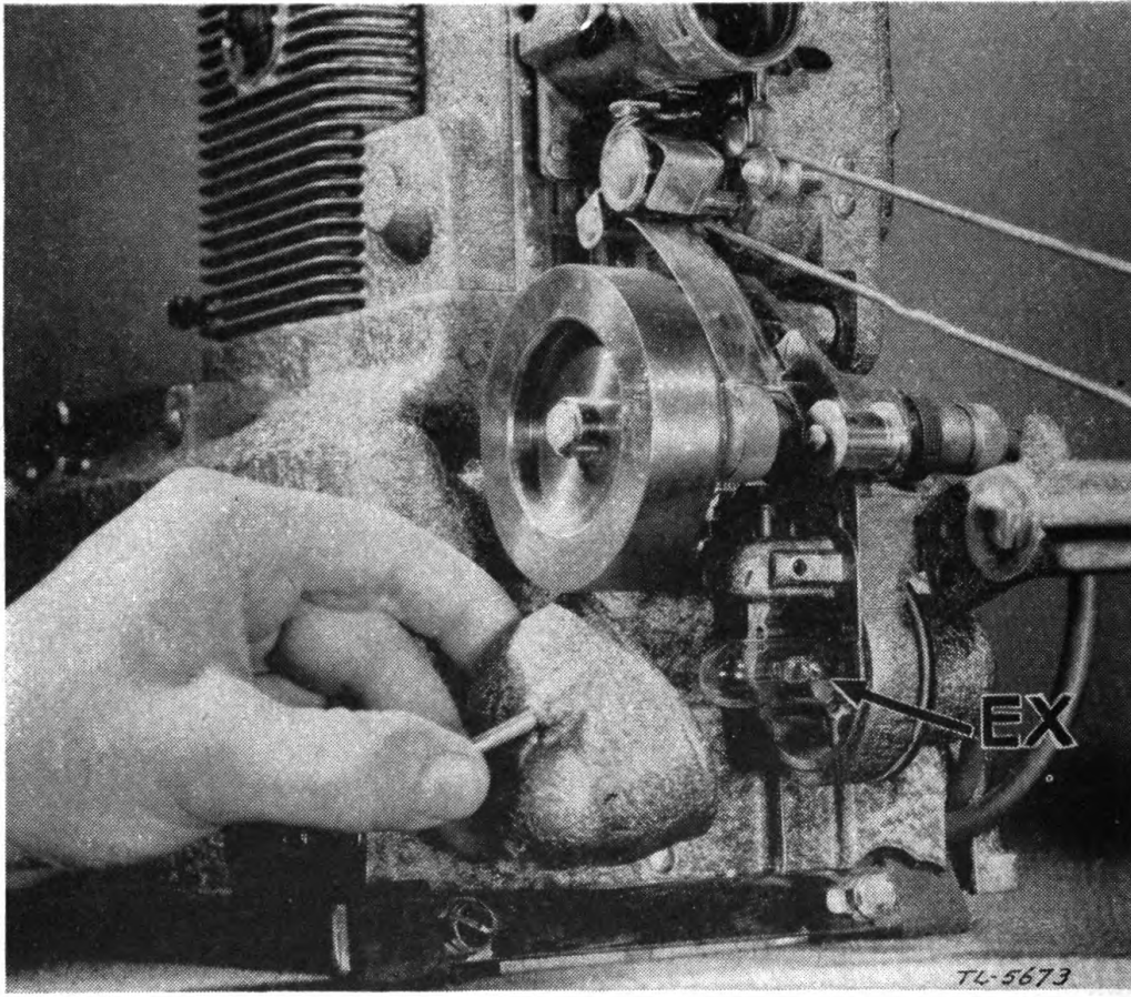
FIGURE 61.—Removing Ampro YA exciter lamp.
