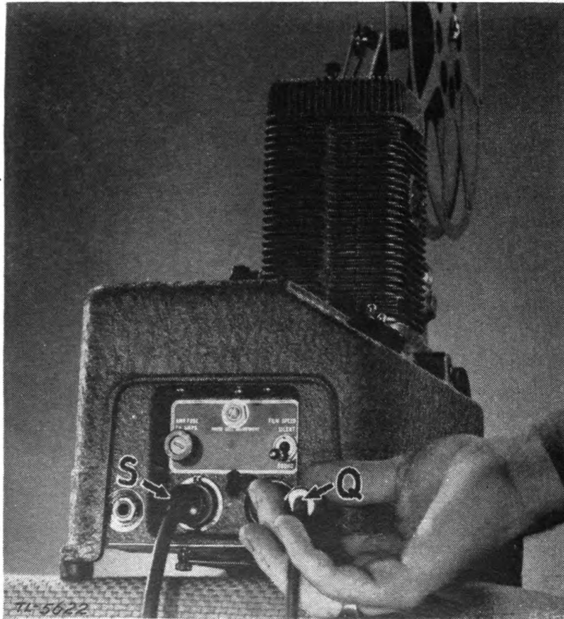
FIGURE 11.—Ampro YA electrical connections.
