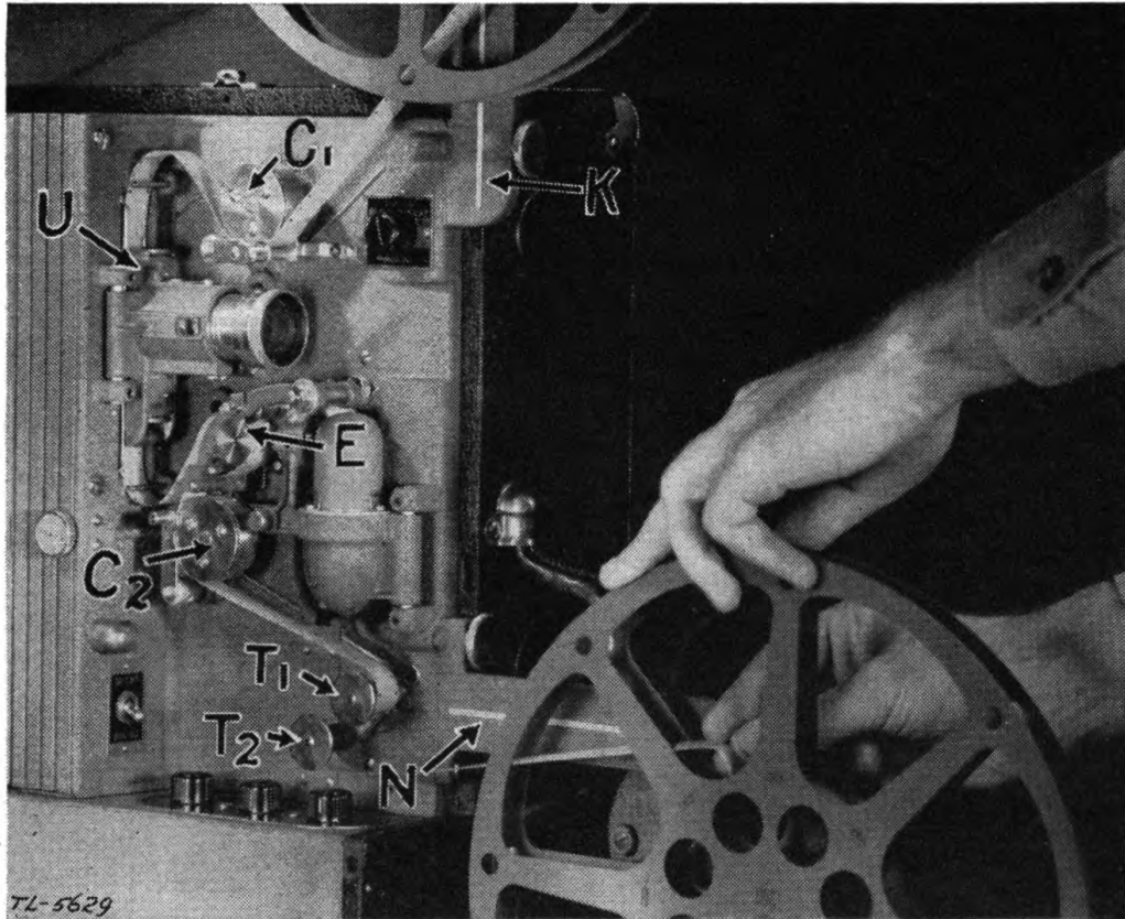
FIGURE 18.—R. C. A. projector with film threaded.
