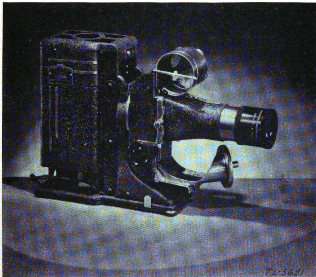
FIGURE 69.—Projector PH-222—assembled.
