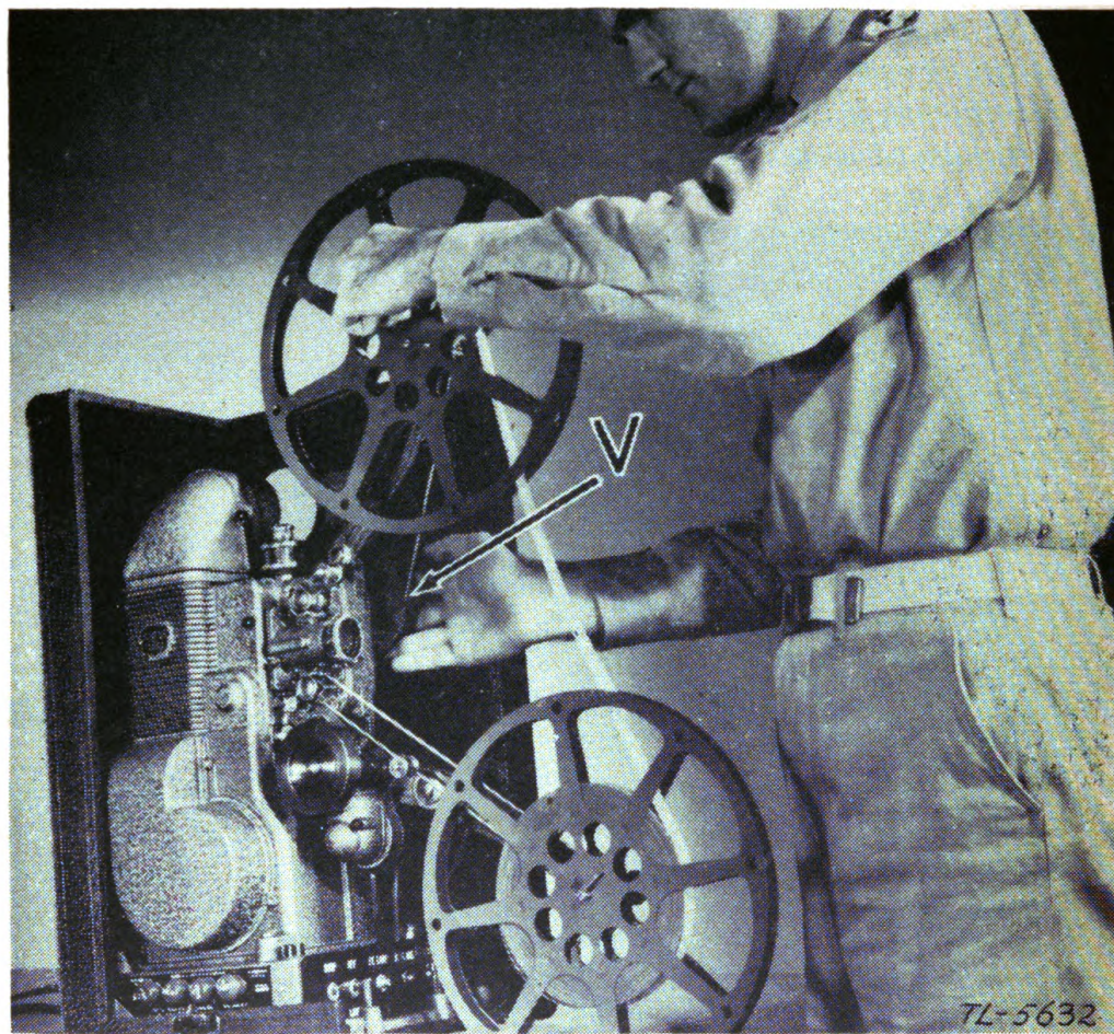
FIGURE 21.—Rewinding Phonofilm projector.
