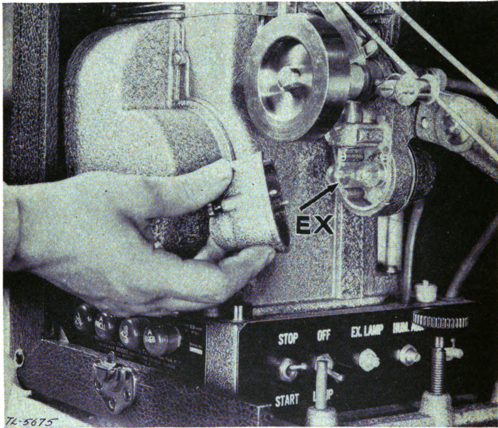
FIGURE 63.—Removing Phonofilm exciter lamp.
