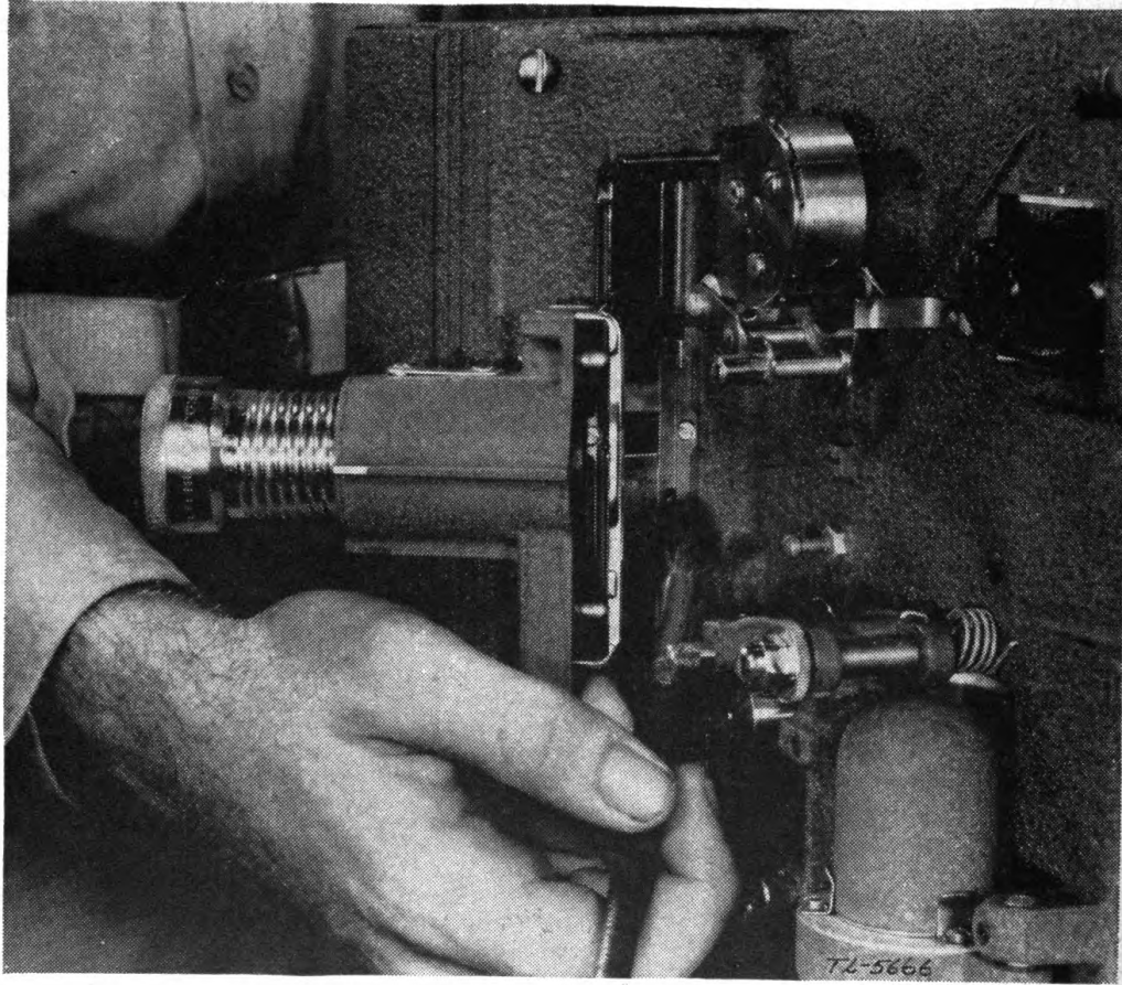
FIGURE 54.—Cleaning the film gate.
