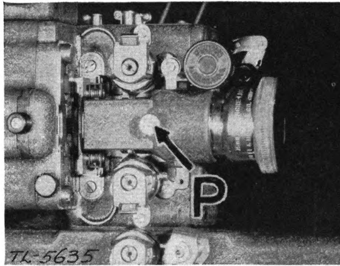
FIGURE 24.—Lens setscrew.
