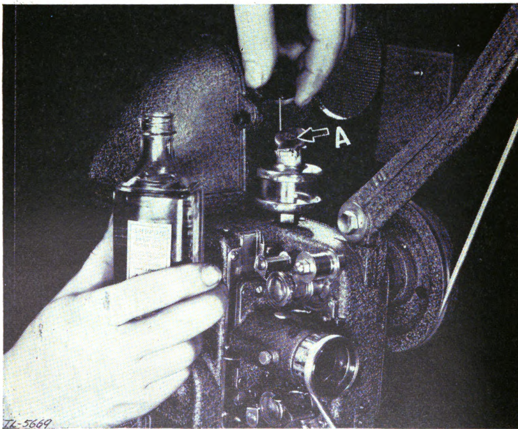
FIGURE 57.—Oiling system of Phonofilm projector.
