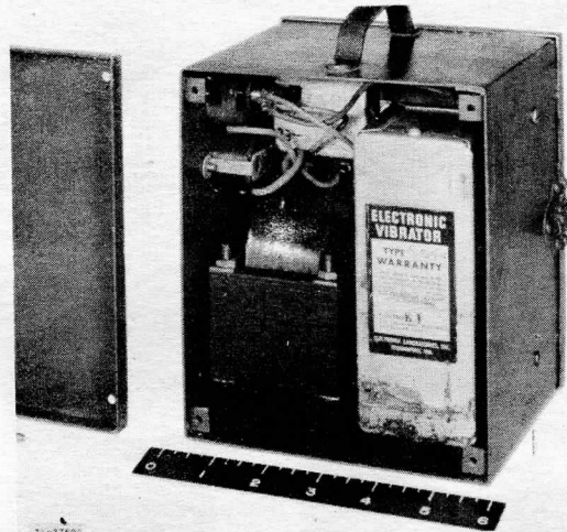
CONVERTER M-222 (RINGING) WITH COVERS REMOVED
