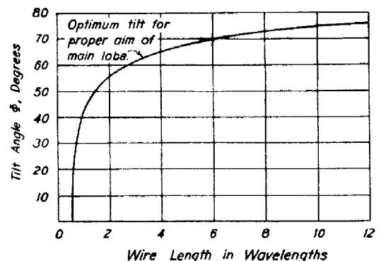
Fig. 2 - OPTIMUM TILT ANGLE FOR RHOMBIC ANTENNA
