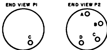
Figure 5-1. Headset-Microphone H-161/U, wiring diagram.
