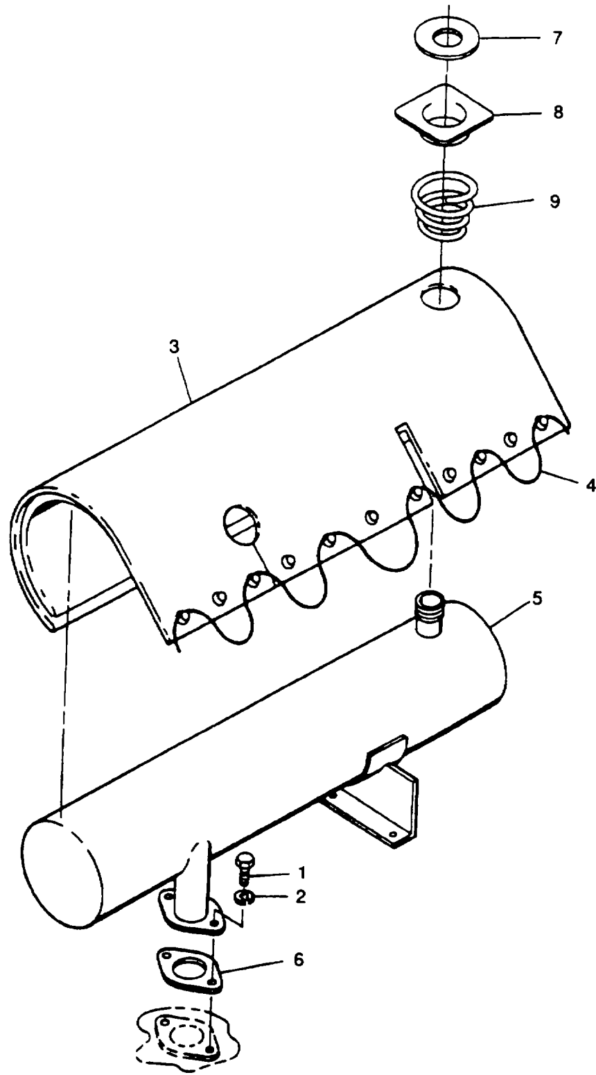
Figure 14. Muffler Assembly
