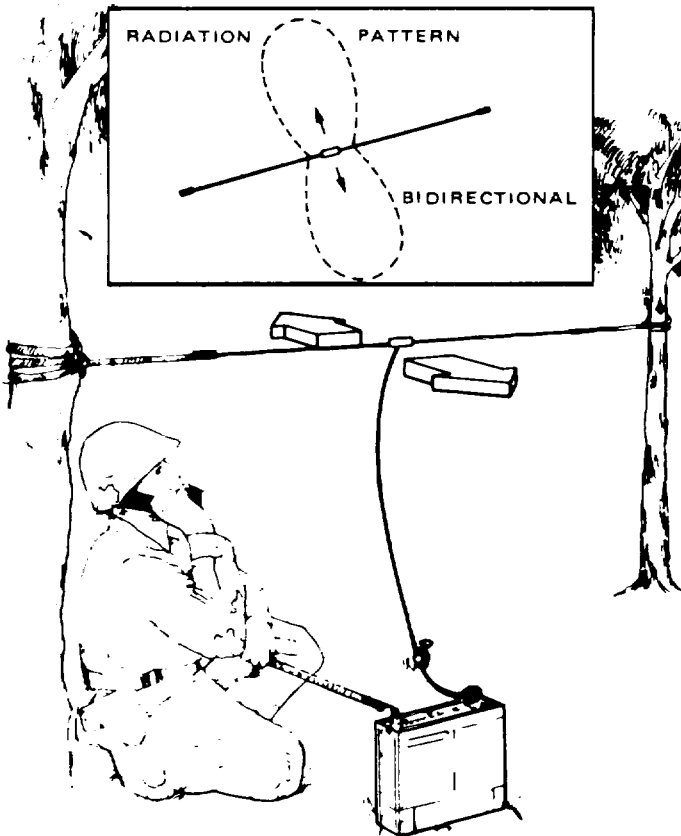
C. HALF-WAVE DIPOLE
