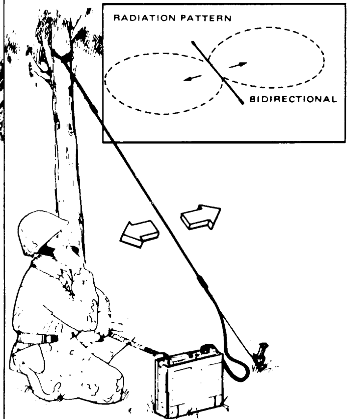
D. QUARTER-WAVE SLANT WIRE
