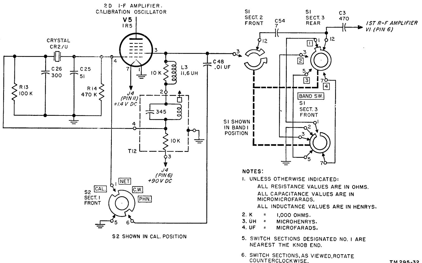
Figure 31. Radio Receiver R-174/URR, calibration oscillator, functional schematic.
