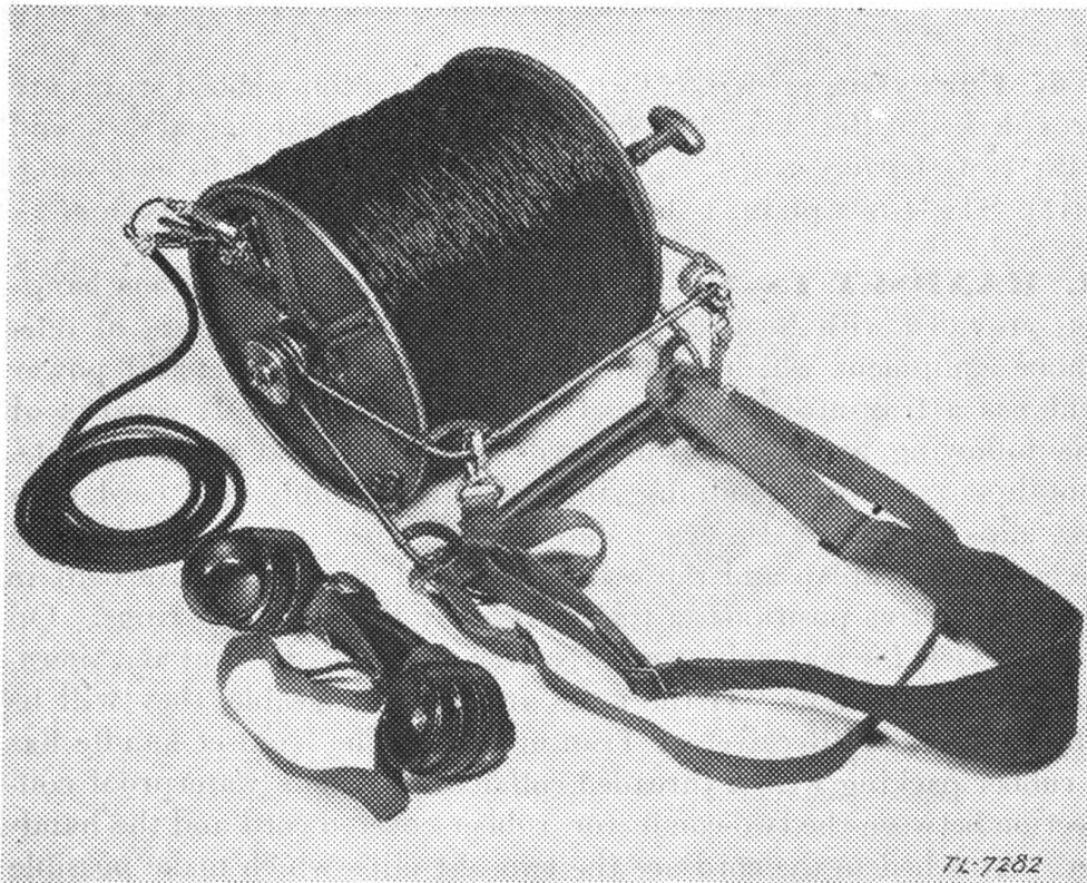
Figure 1. Reel Equipment CE-11.
