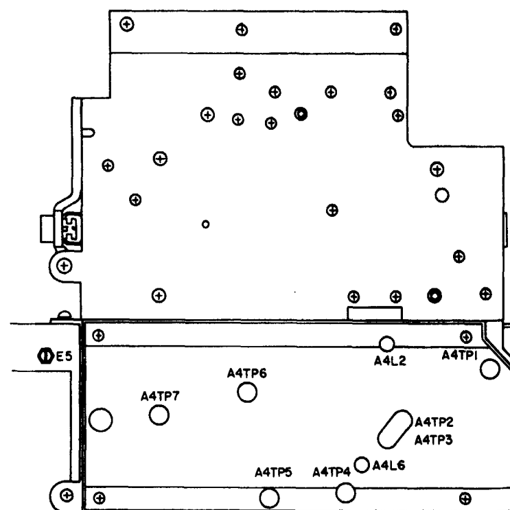
BOTTOM VIEW
