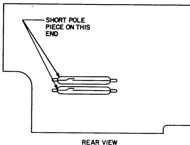
Figure 7-11. Calibration oscillator, A1A1A2A6A1, parts location.
