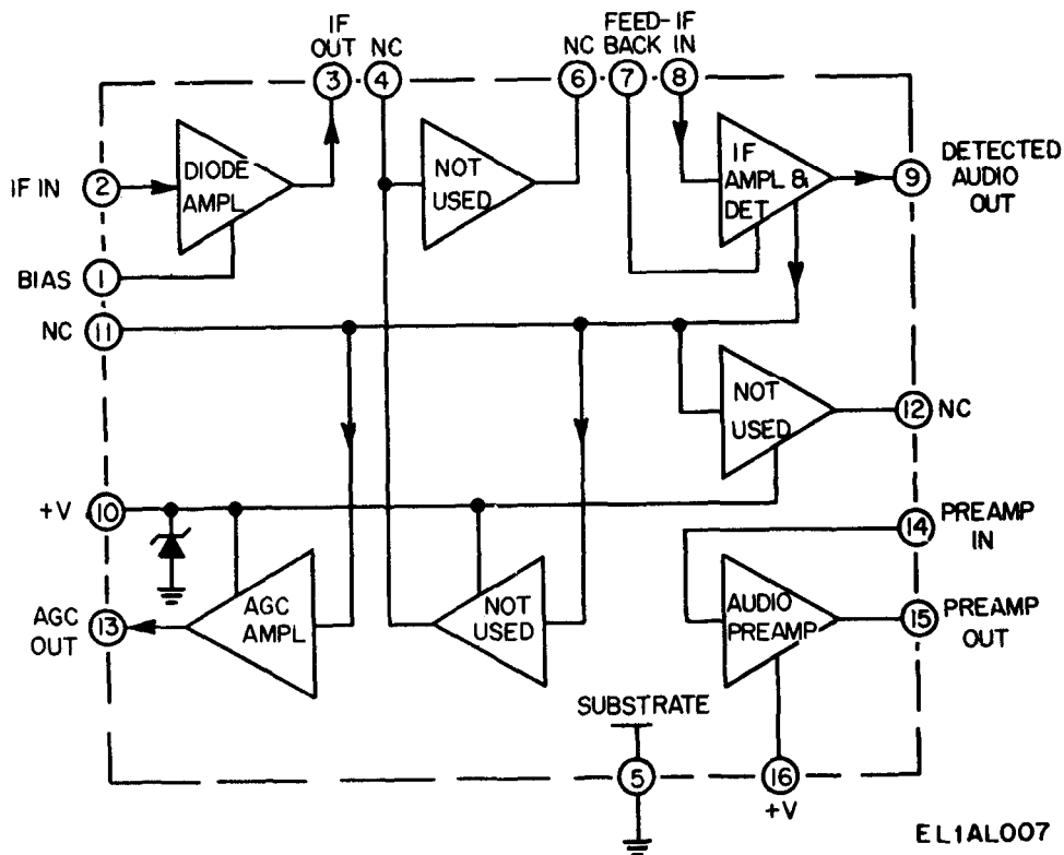
Figure 5-1. Block diagram, AM receiver subsystem integrated circuit.
