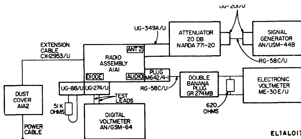
Figure 6-9. IF amplifier gain adjustment connections.
