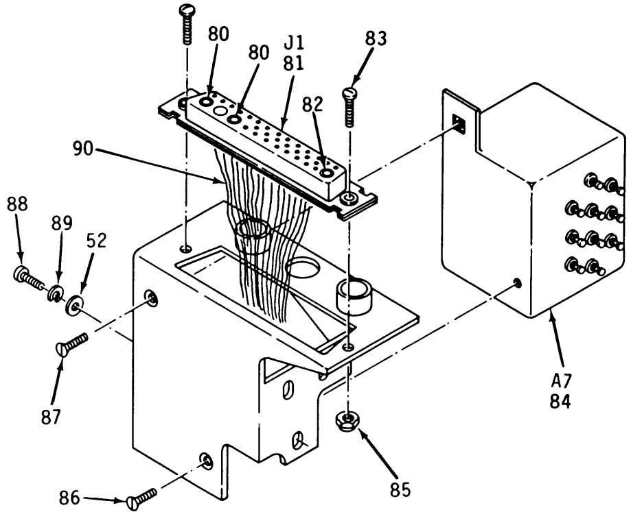
PARTIAL REAR VIEW LOWER LEFT CORNER
