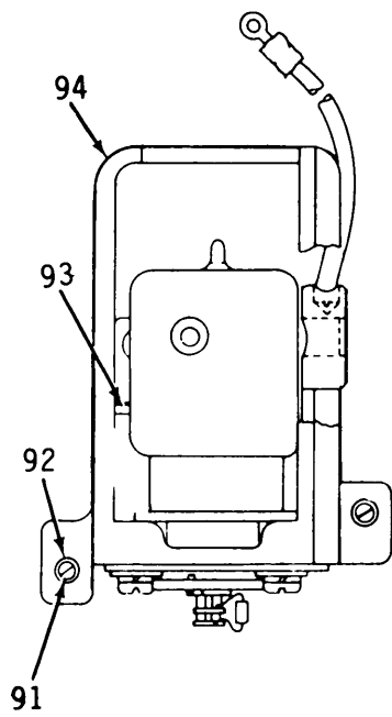
PARTIAL REAR VIEW LOWER RIGHT CORNER
