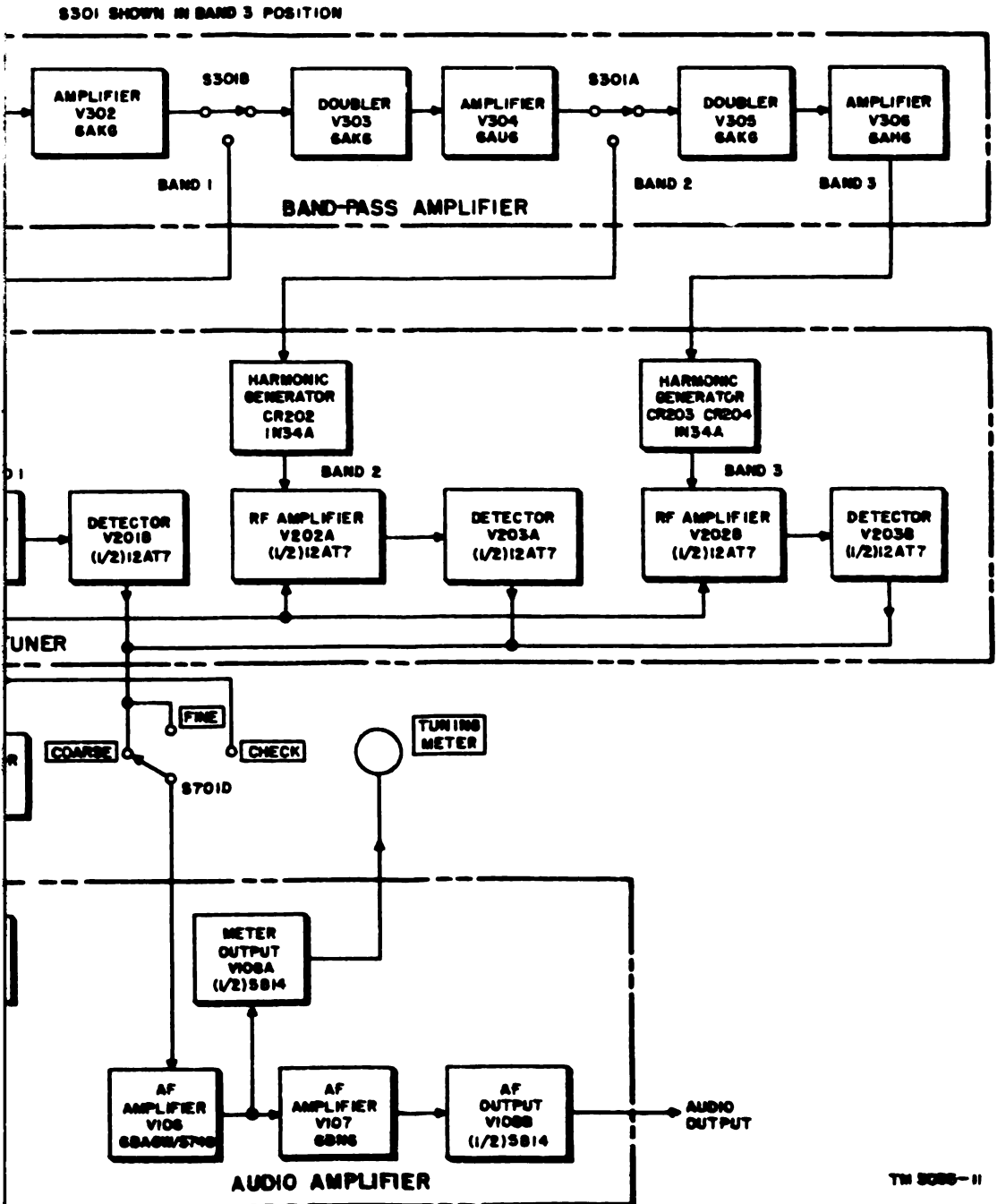
R-5/U, block diagram.
