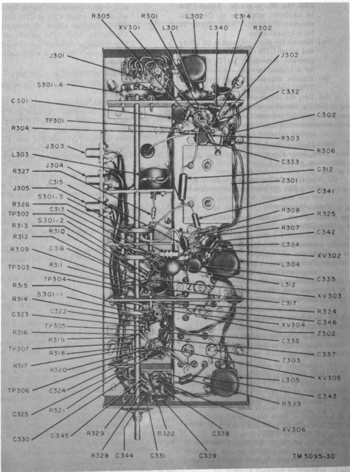
Figure 33. Frequency Meter FR-5jU, band-pass amplifier, location of parts, bottom view.
