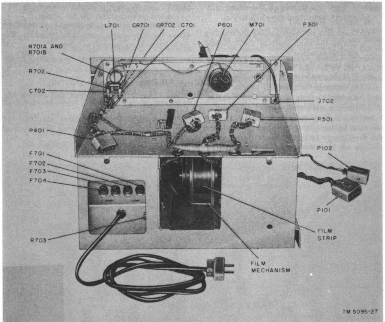
Figure 29. Frequency Meter FR-5/U, location of parts, rear view.
