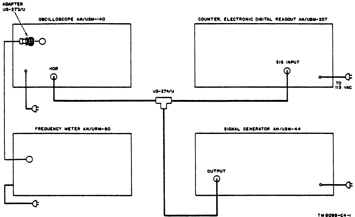
Figure 38.1. Crystal check.
