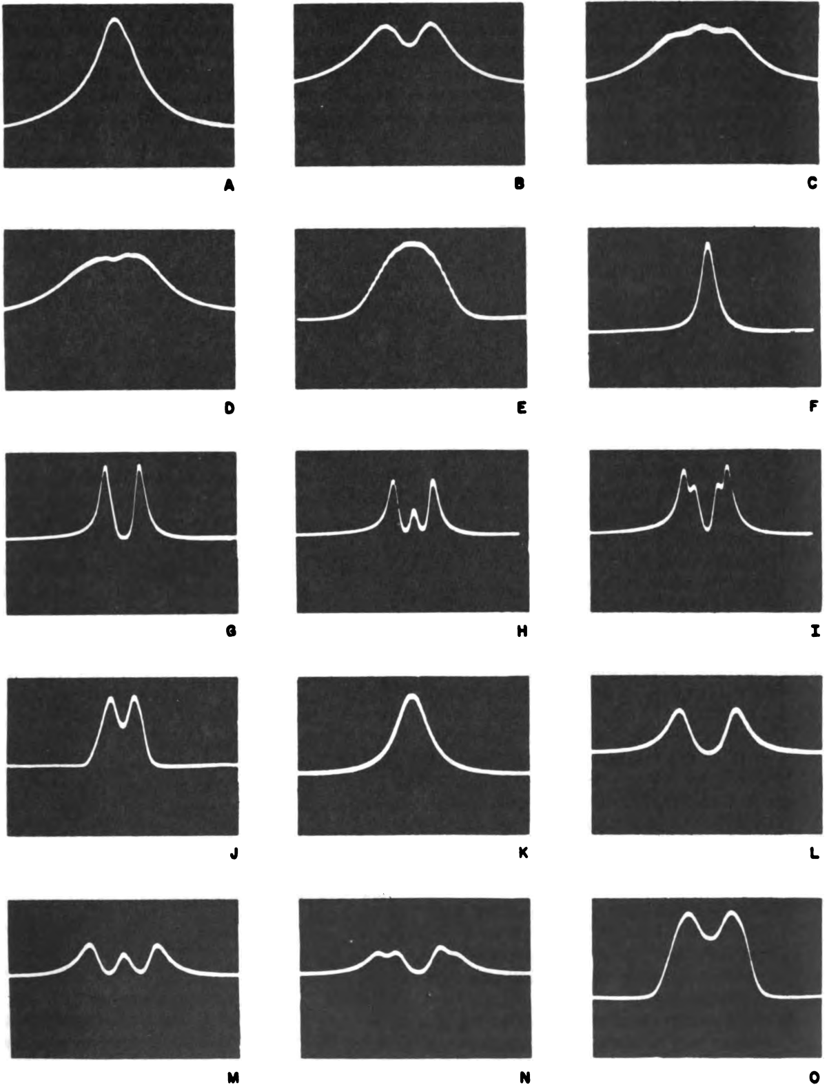
Figure 34. Frequency Meter FR-5/U, wave forms.
