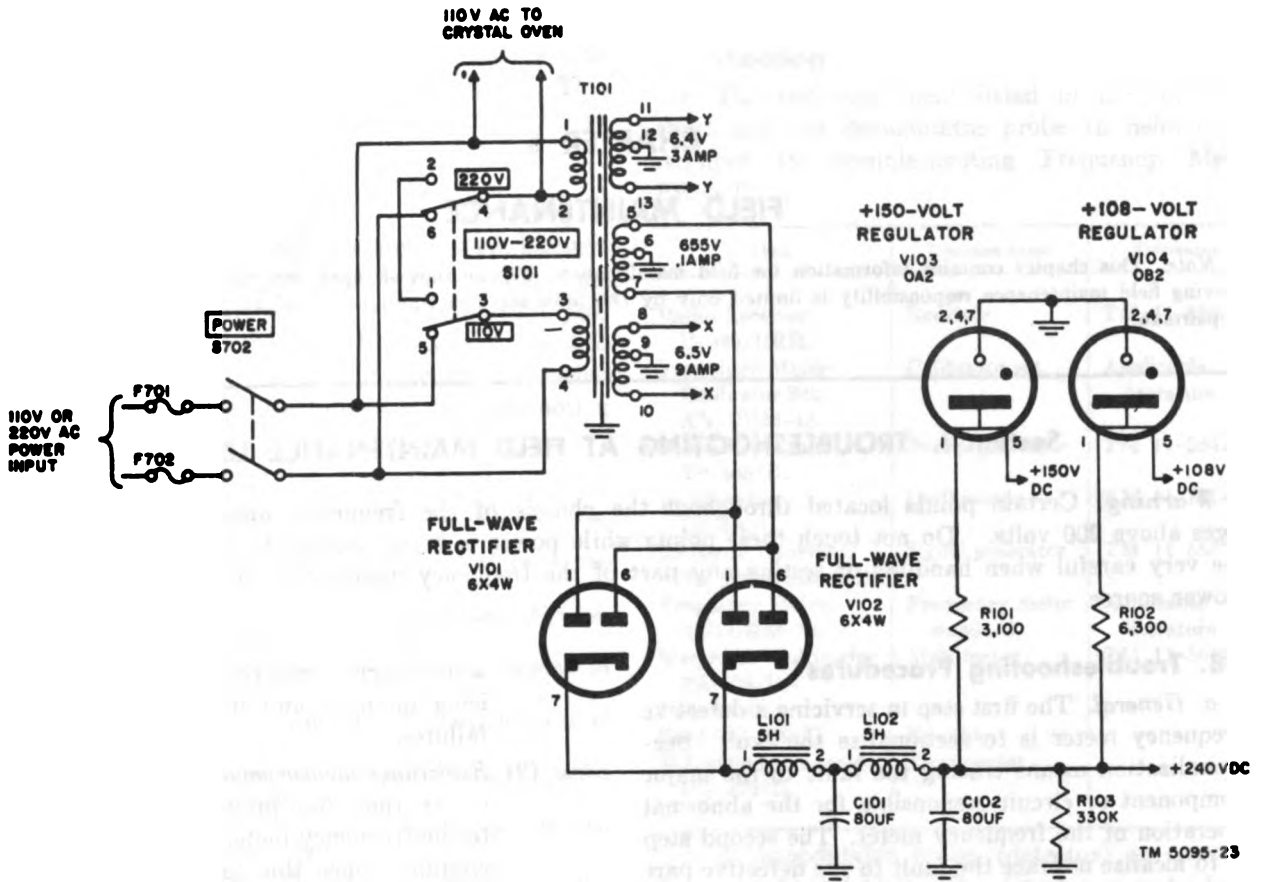
Figure 81. Power supply, simplified schematic diagram.
