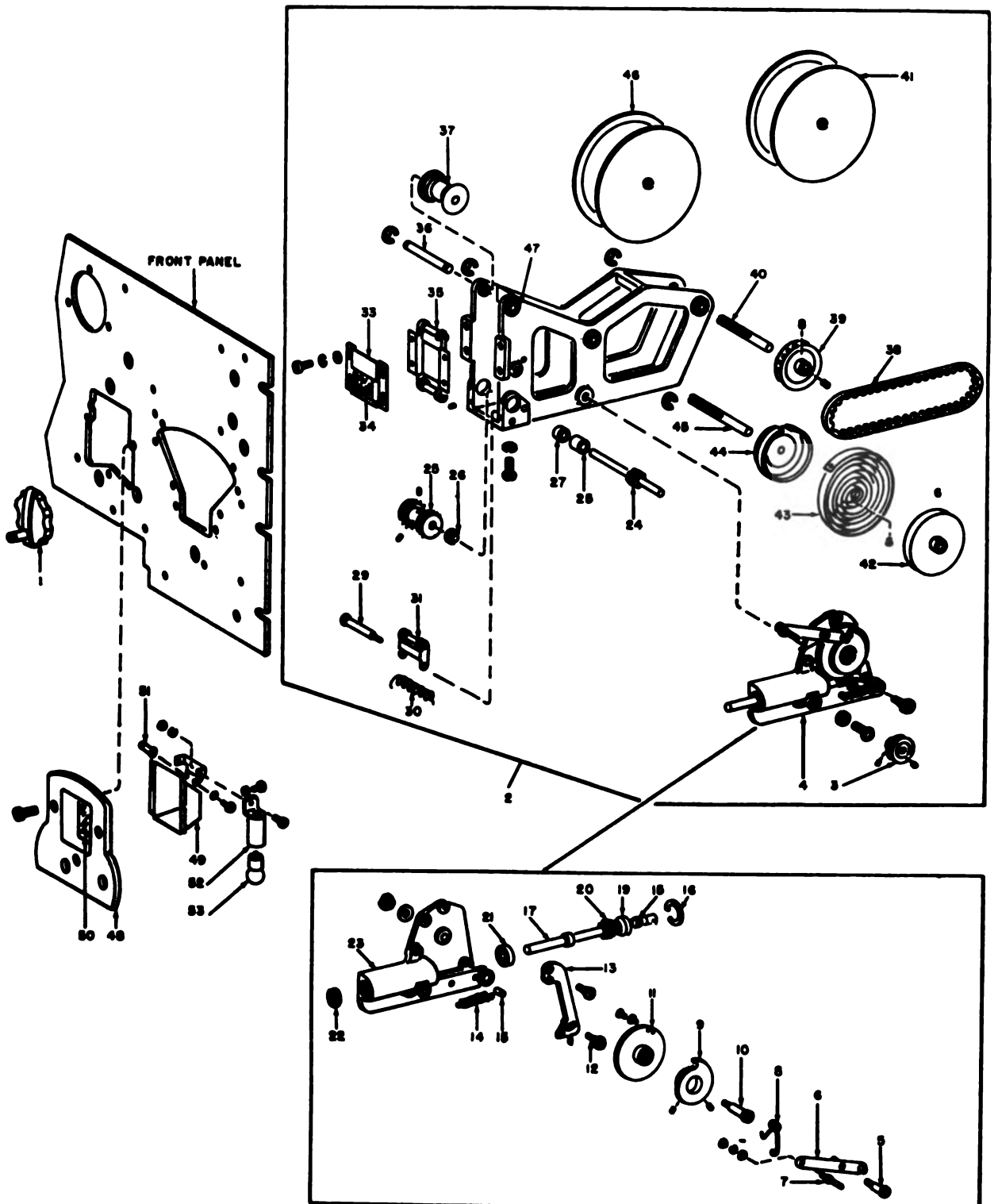
Figure 26. Film mechanism assembly, exploded view.
