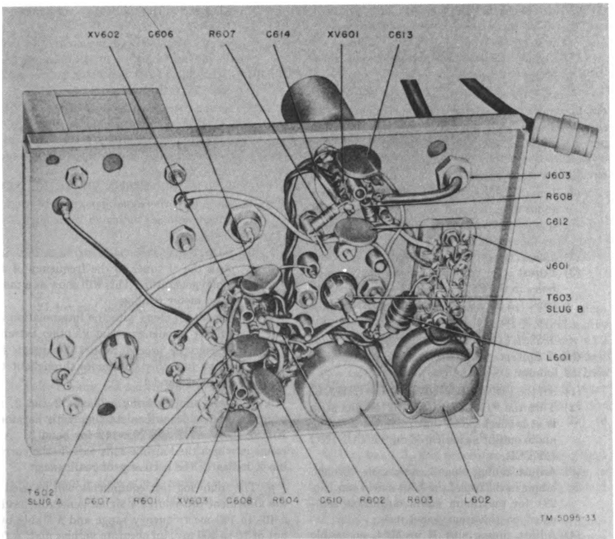
Figure 36. Frequency Meter FR-5/U, balanced modulator, location of parts, bottom view.
