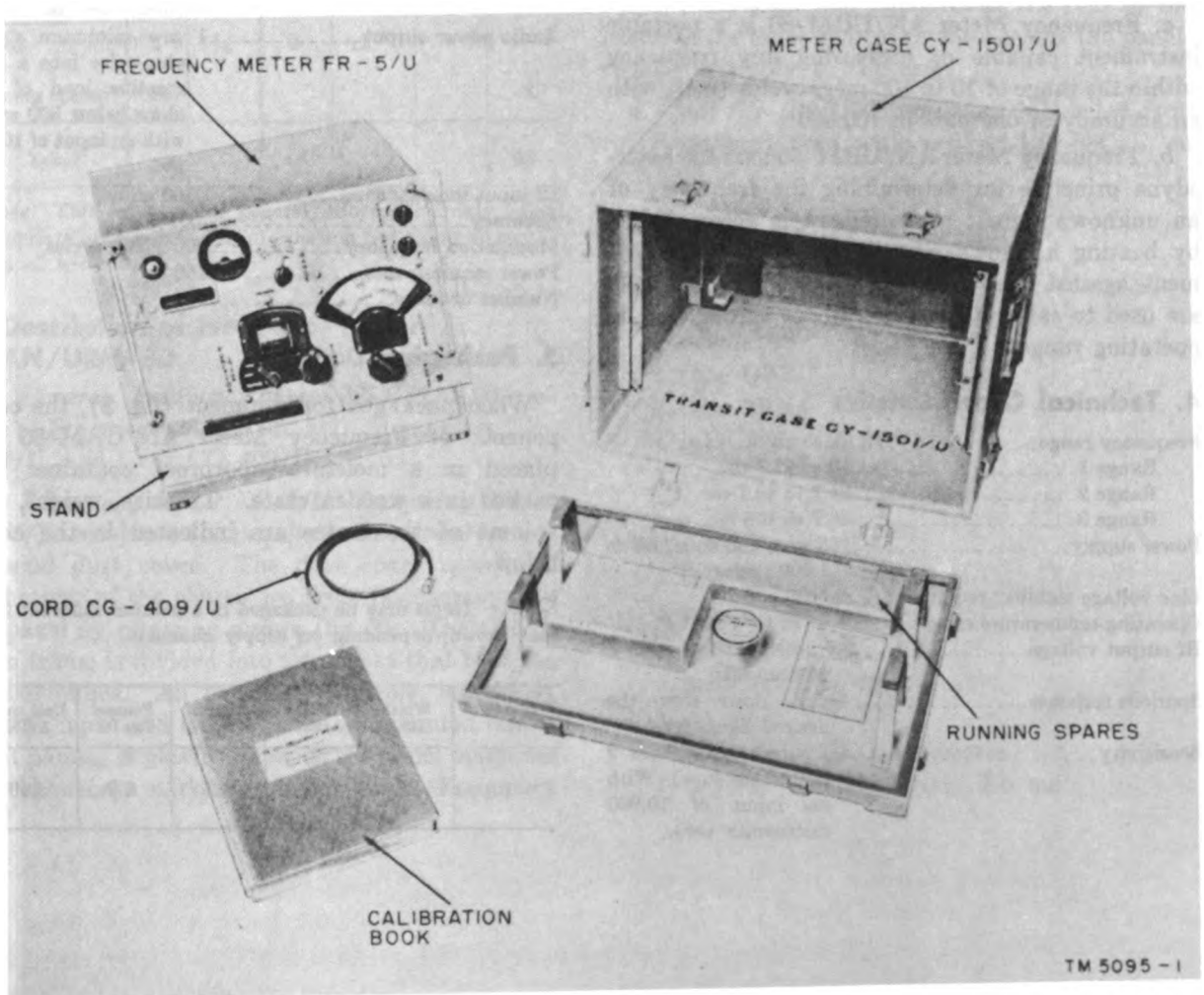
Figure 1. Frequency AN/URM-80.
