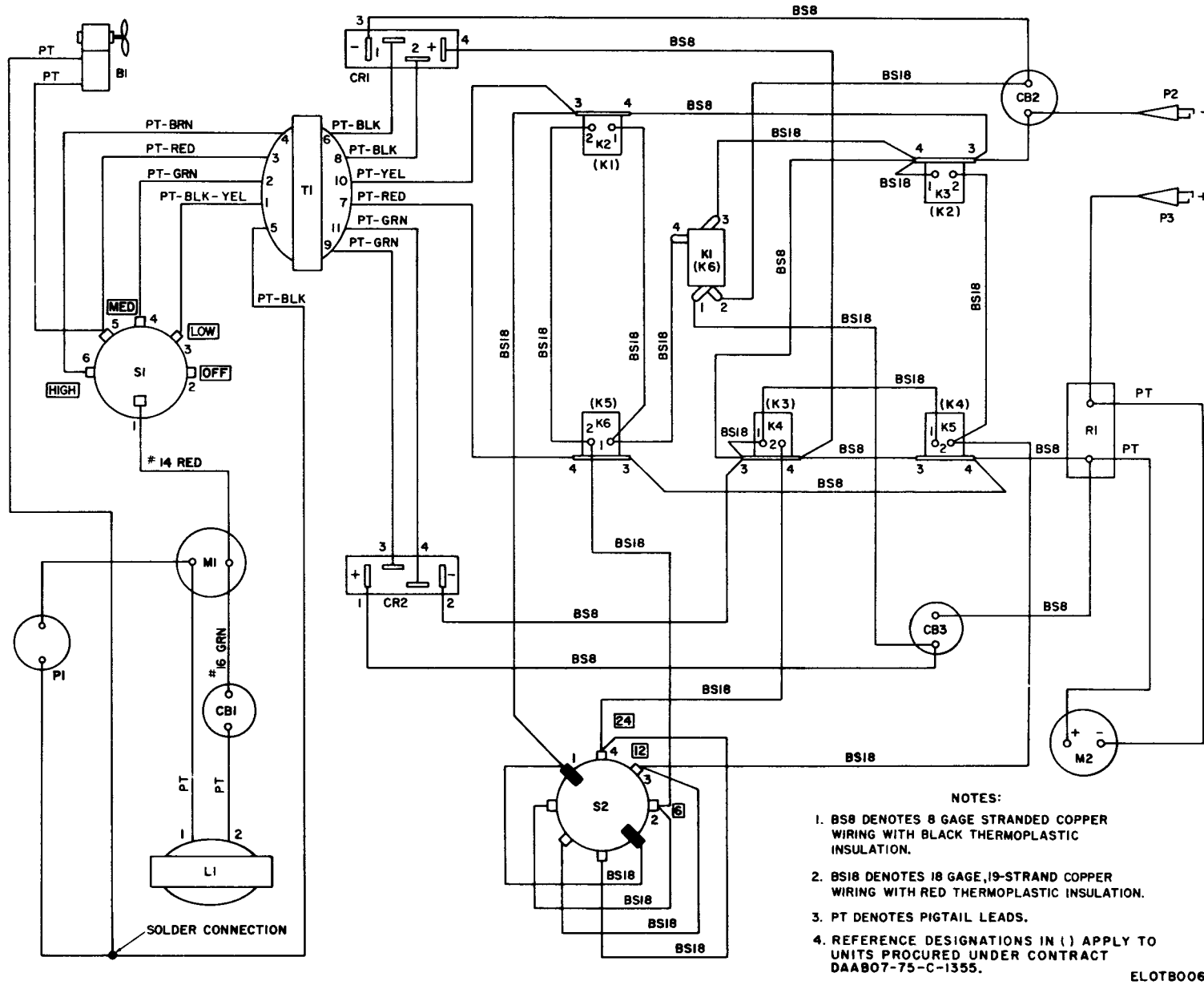
Figure 3-6. Charger, Battery PP-1660 JG, Wiring Diagram.
