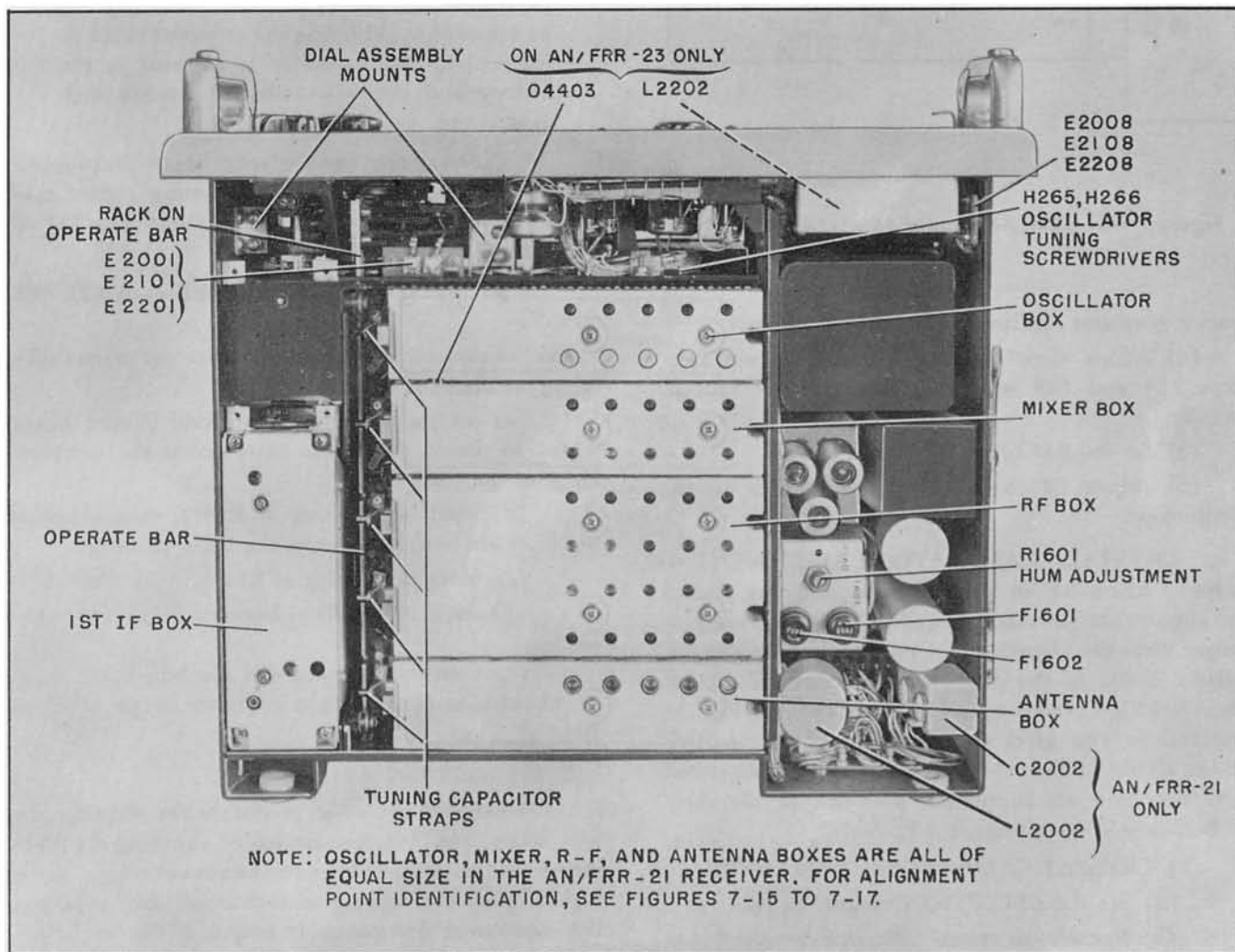
CHASSIS BOTTOM VIEW
