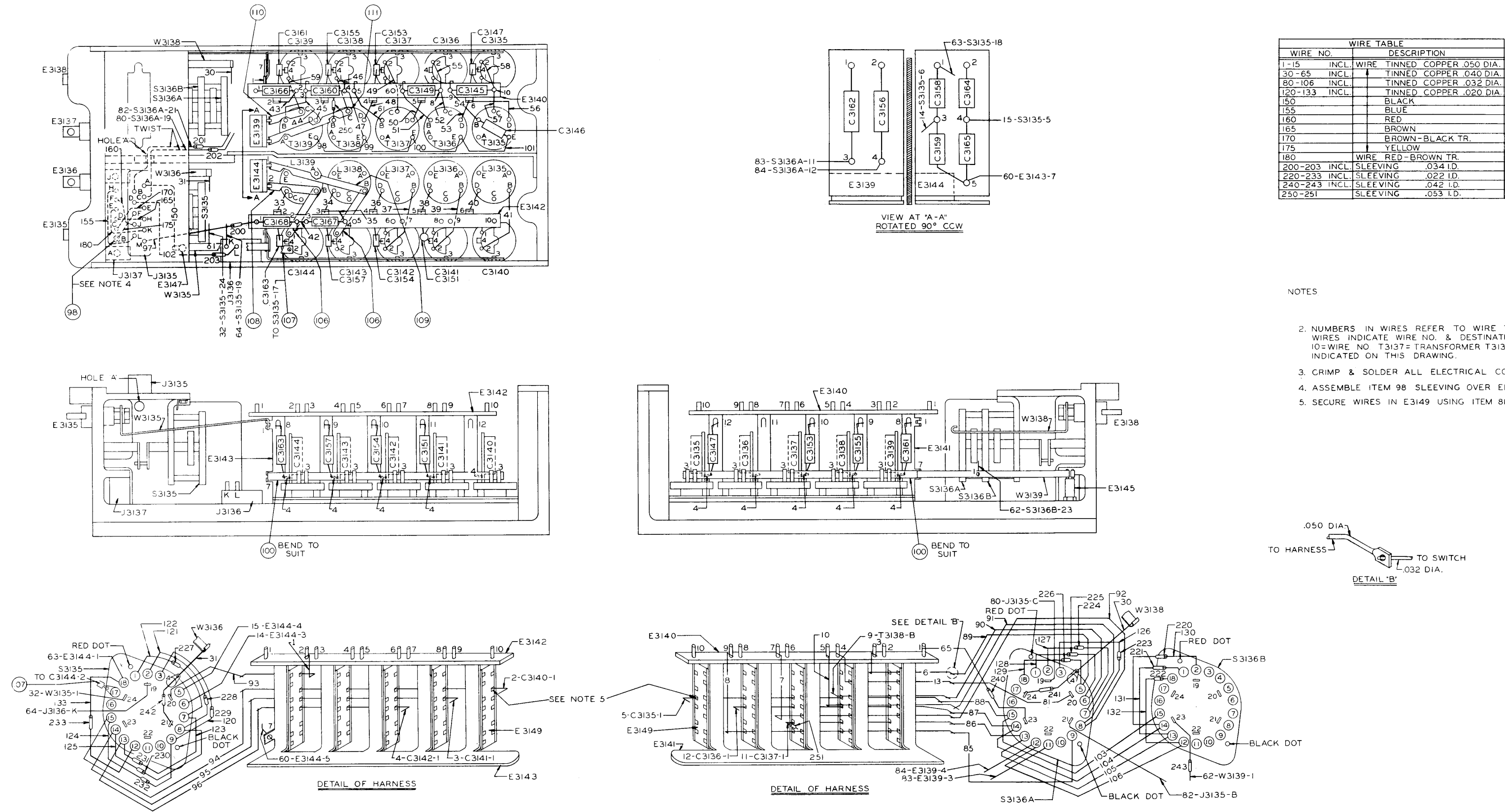
Figure 7-28. R-F Amplifier, Connection Diagram, AN/FRR-23
