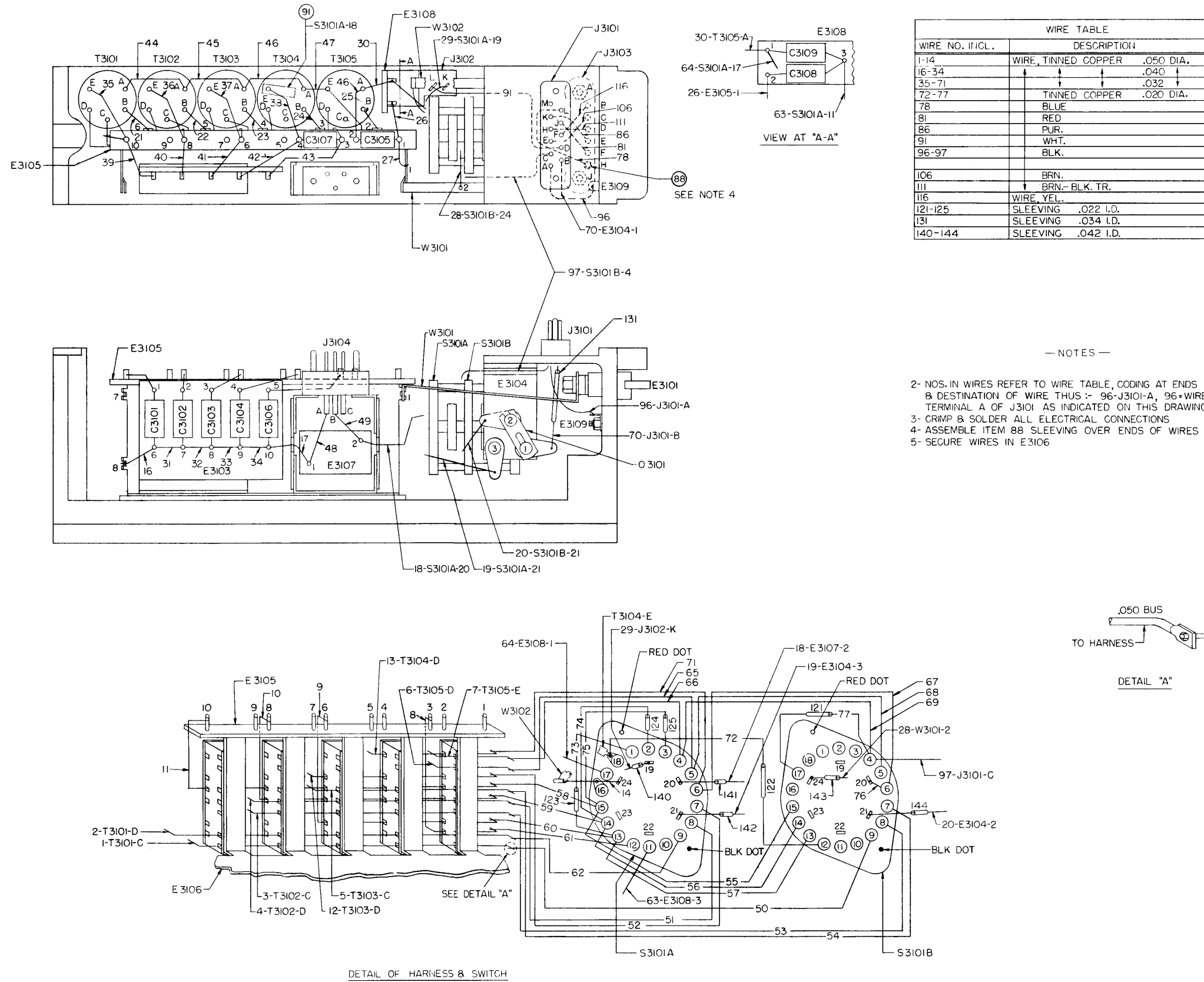
Figure 7-25. Antenna Box, Connection Diagram, AN/FRR-23
