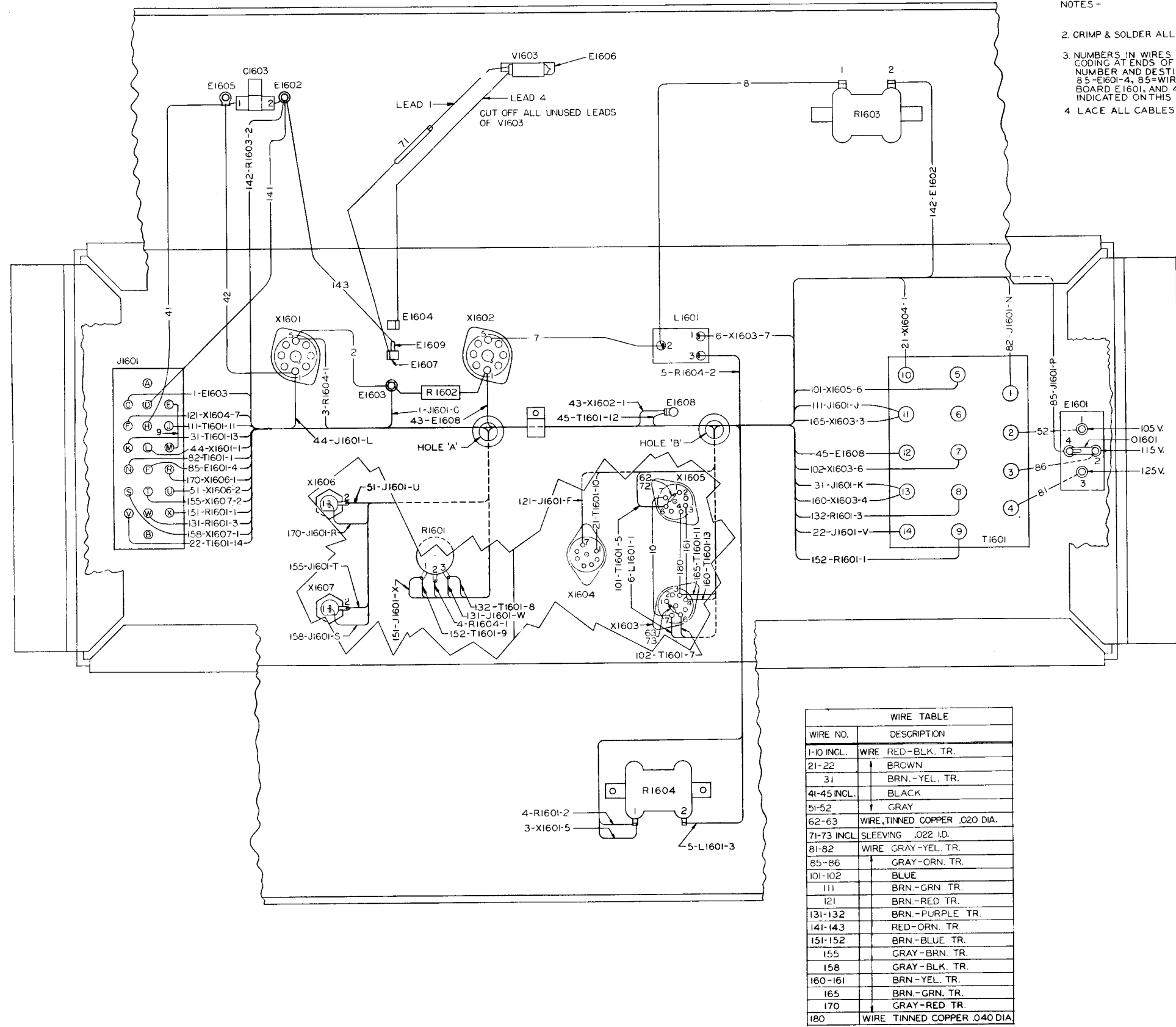
Figure 7-44. Power Supply, Connection Diagram
