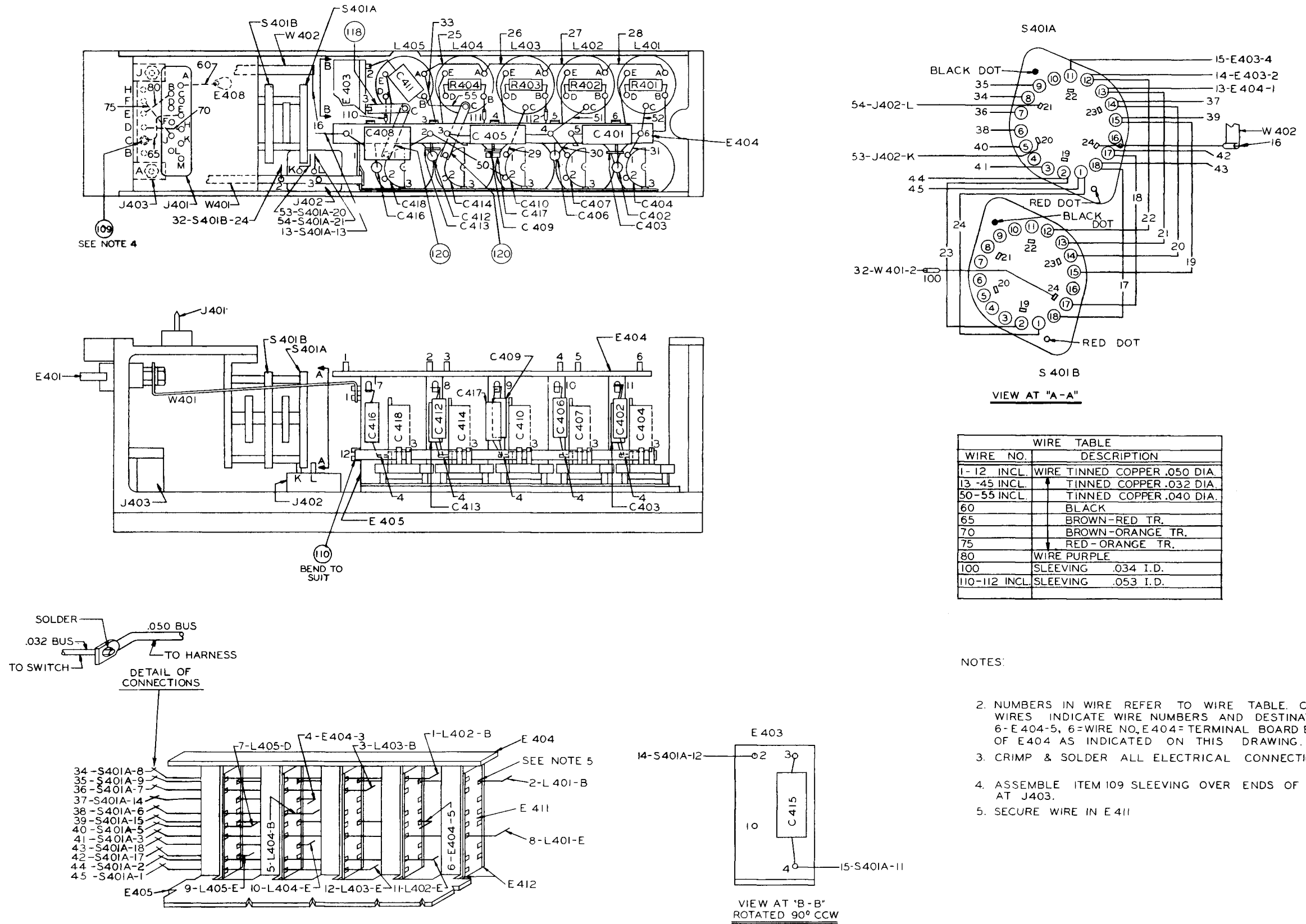
Figure 7-33. Oscillator, Connection Diagram, AN/FRR-22
