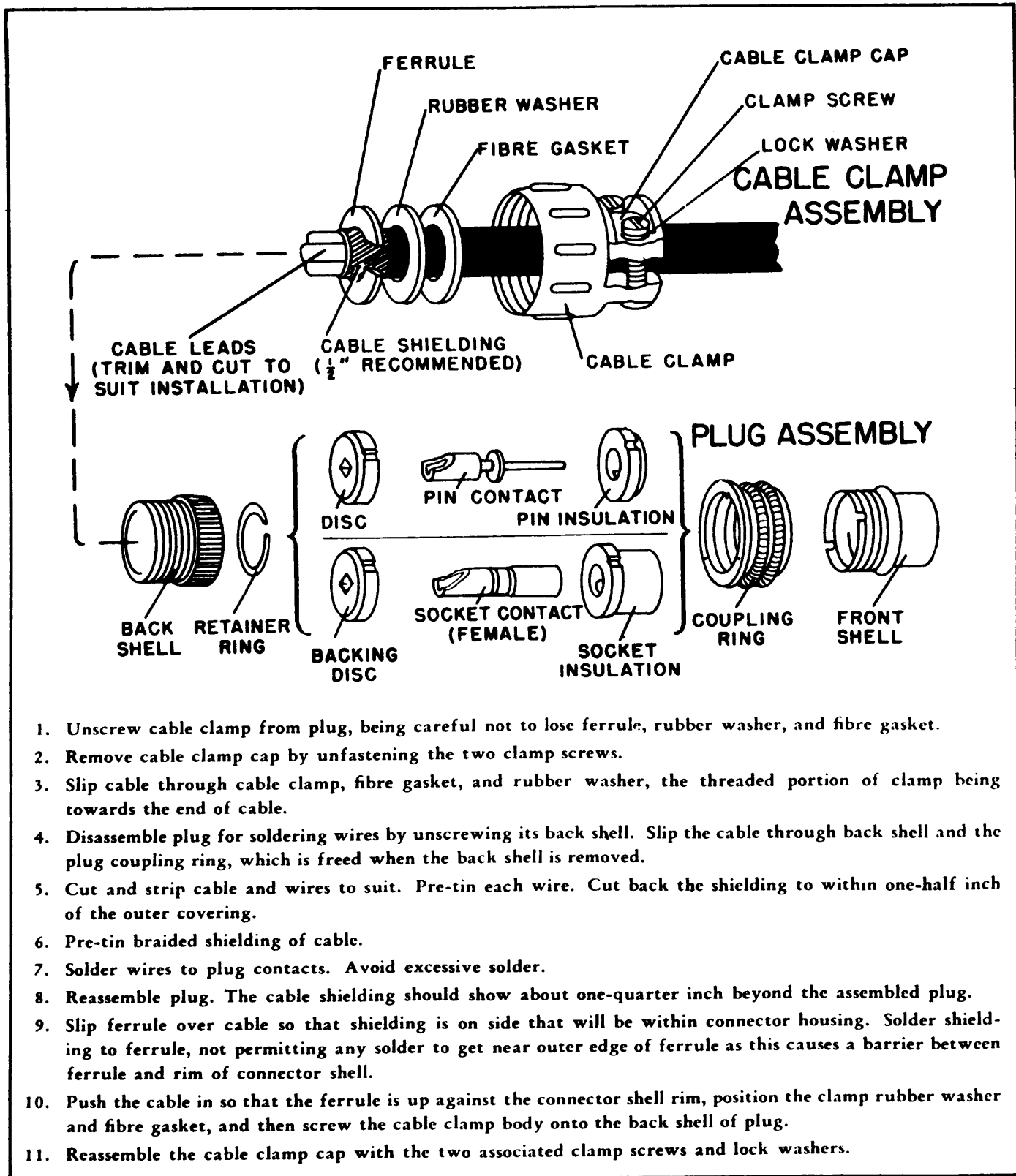
Figure 3-6. Cable Fabrication, AN-3106A Plugs
