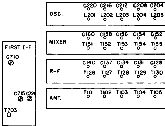
Figure 7-15. R-F Alignment Points, AN/FRR-21
