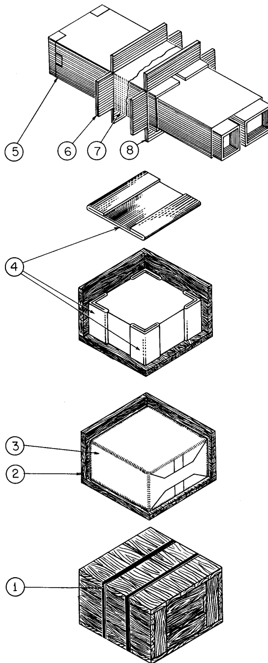
Figure 3-1. Unpacking
