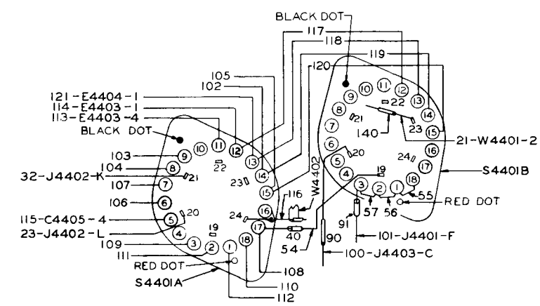
VIEW AT "A-A" USE IN CONJUNCTION WITH DETAIL OF HARNESS
