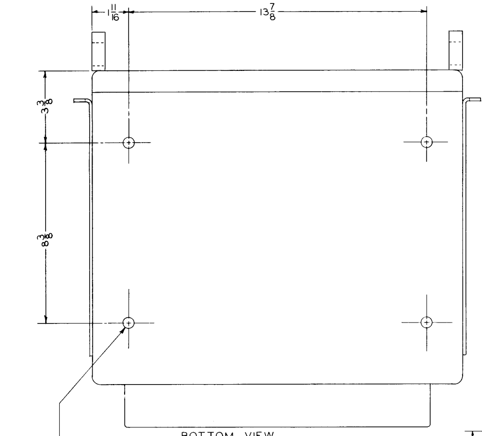
RACK OR BASE MOUNTING ASSEMBLY
