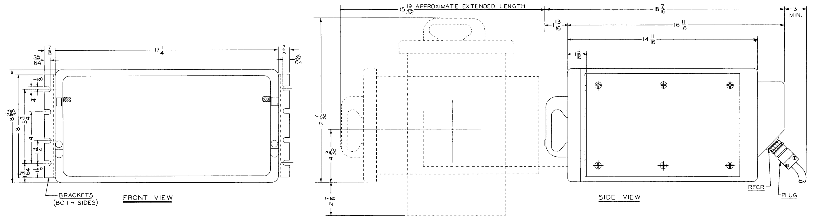
RACK OR BASE MOUNTING ASSEMBLY
