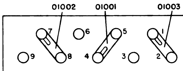
(B) LINK POSITIONS IN COMPANION RECEIVER
