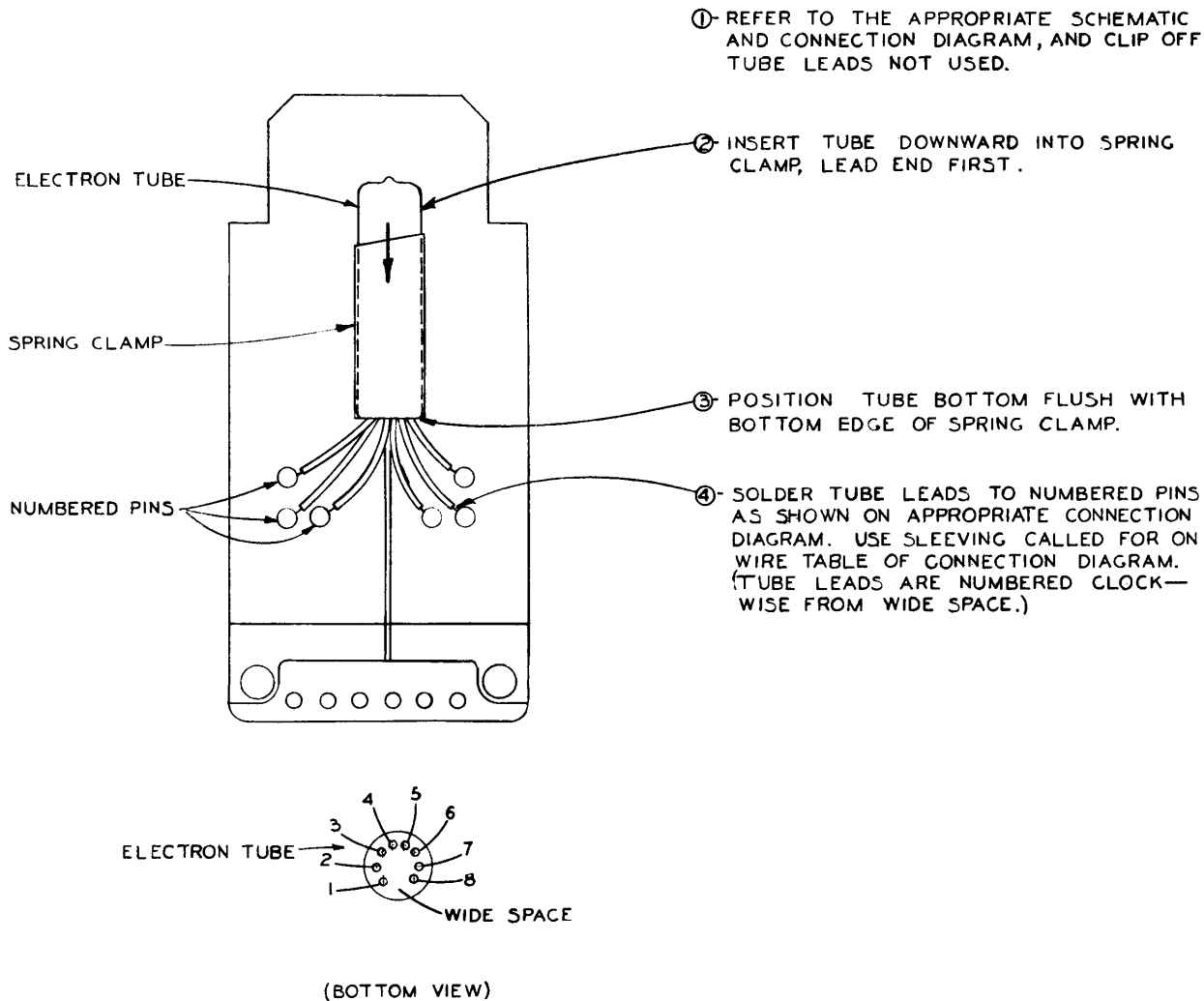
Figure 7-7. Eight-Pin Electron Tube Replacement Plug-in Board
