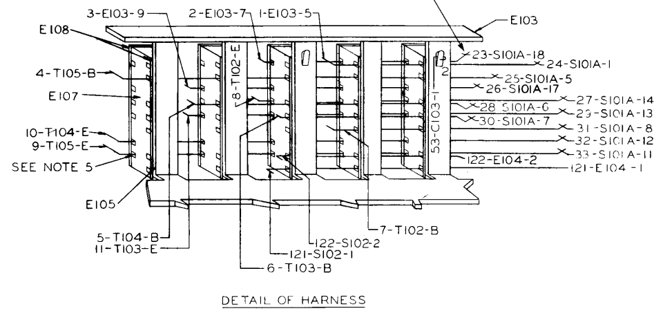
DETAIL OF HARNESS
