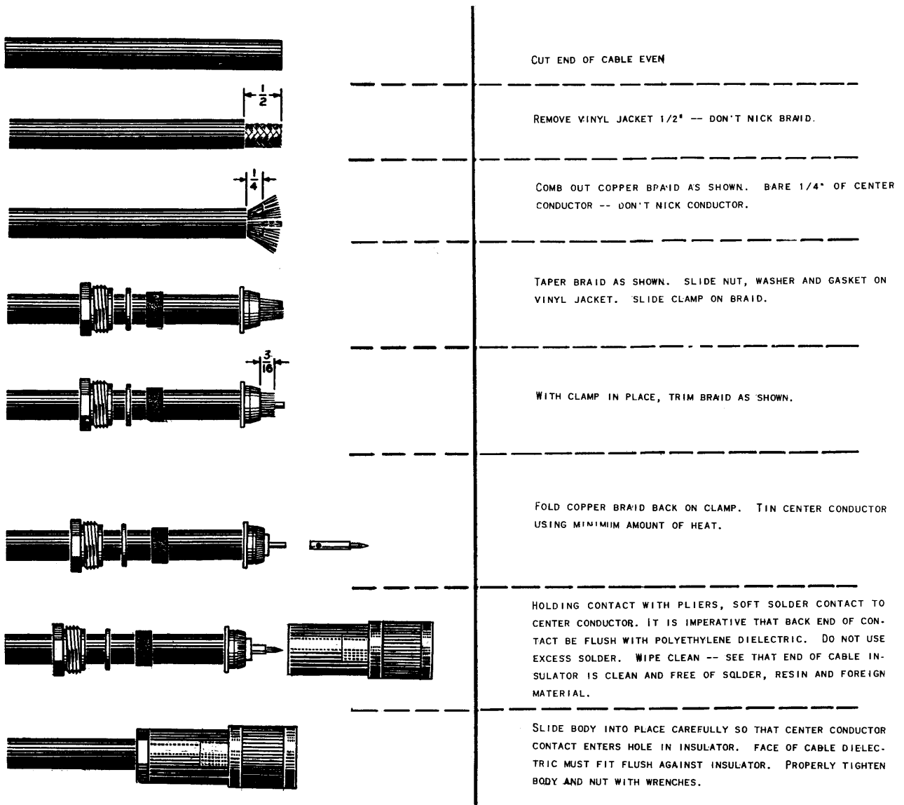
Figure 3-5. Cable Fabrication, UG-21B/U Plug
