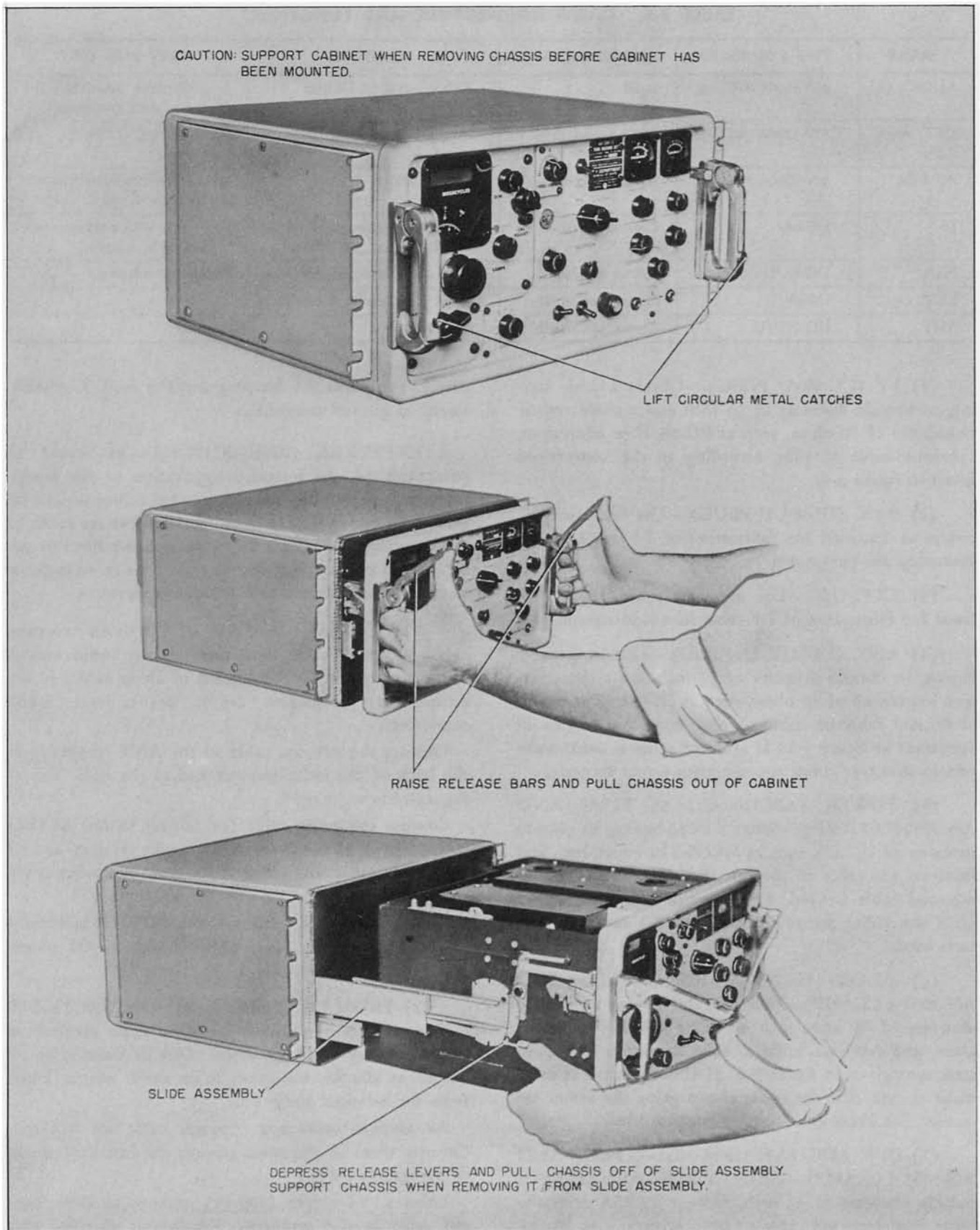
Figure 3-2. Removal of Chassis from Cabinet
