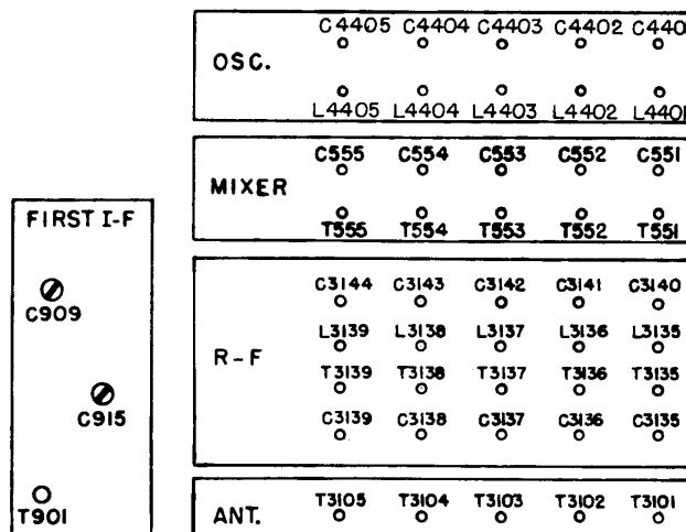
Figure 7-17. R-F Alignment Points, AN/FRR-23
