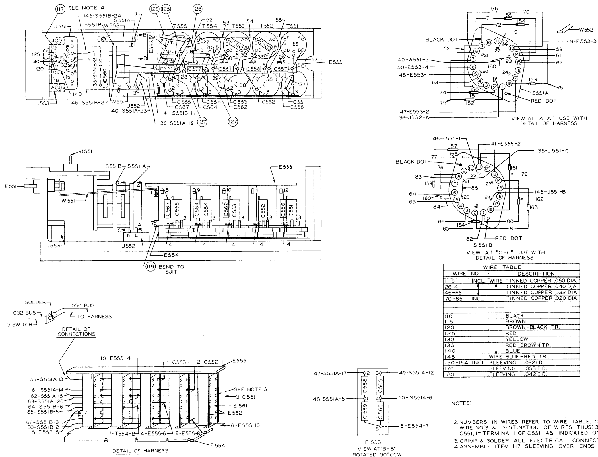
Figure 7-31. Mixer, Connection Diagram, AN/FRR-23
