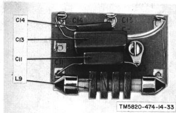
Figure 33. Transmitter terminal board TB2.
