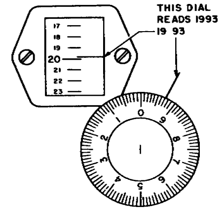
Figure 15 Typical transmitter dial settings
