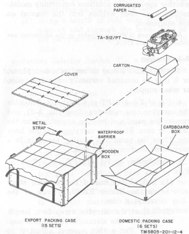
Figure 2-1. Telephone Set TA-312/PT, packaging diagram.
