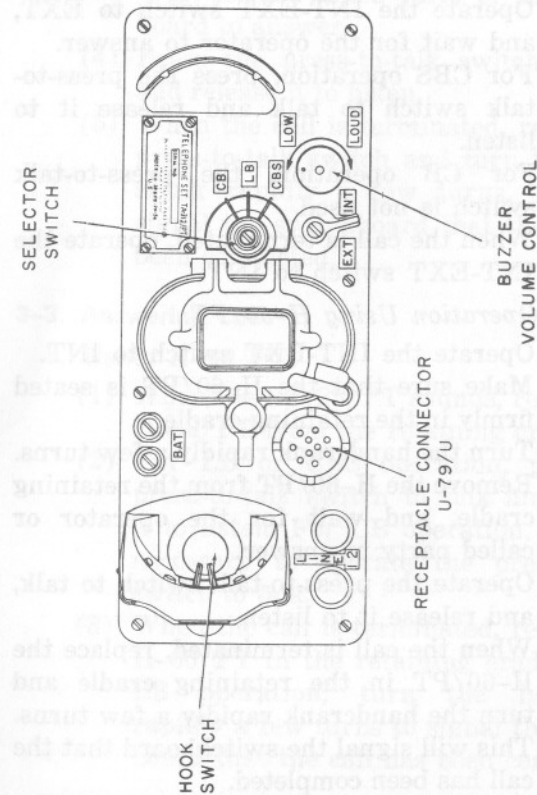
Figure 3-1. Telephone Set TA-312/PT, controls and indicators.
