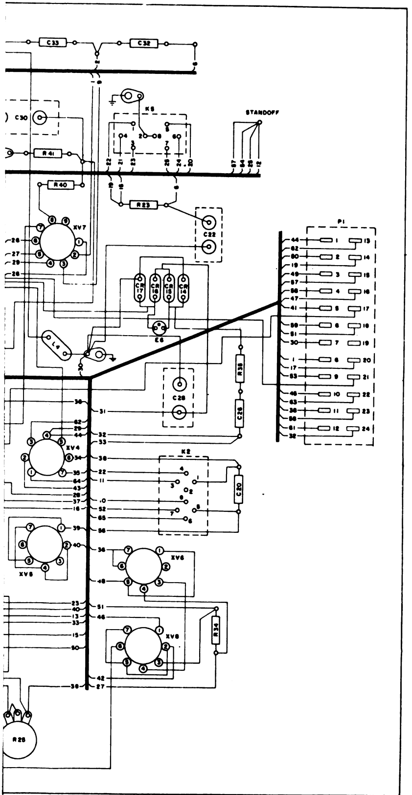
level chassis, wiring diagram.
