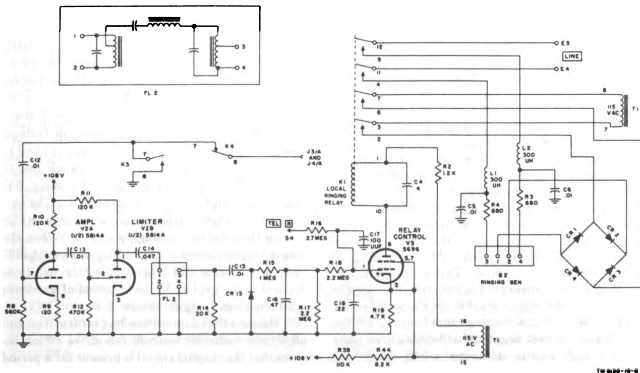
Figure 10. Local telephone ringing circuit.
