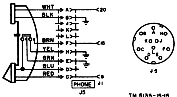
Figure 15. Handset H-33/PT circuit.
