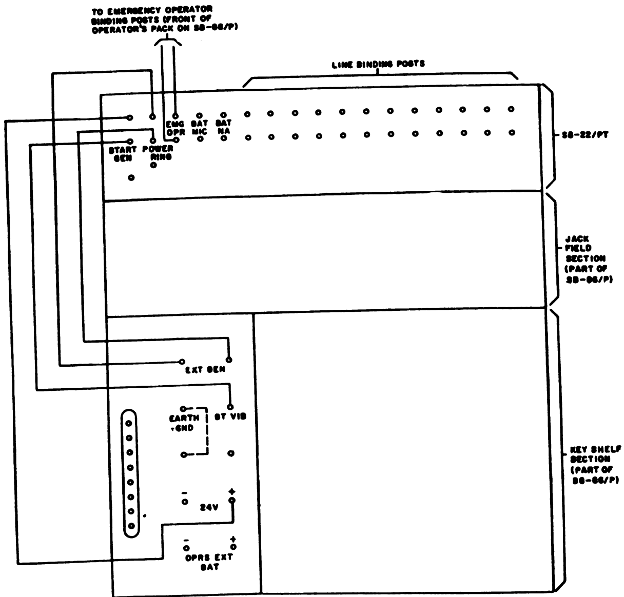
Figure 2.2. Simplified cording diagram, showing connections between SB-86/P and SB-22/PT for push-to-talk radio circuits.
