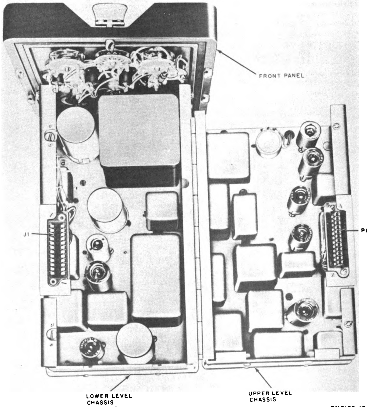
Figure 4. Control unit, upper level chassis swung open.
