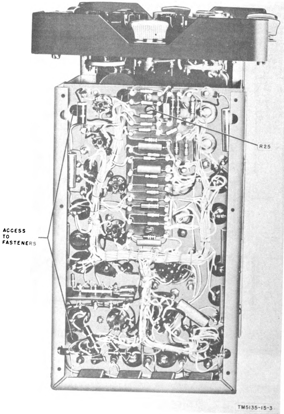
Figure 3. Control unit, case removed, top view.
