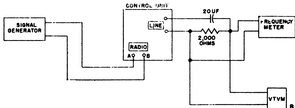
Figure 24. Test equipment connections for final tests.
