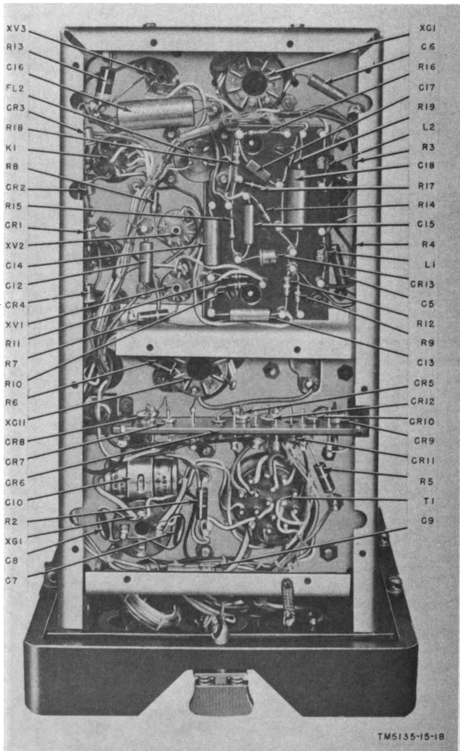
Figure 23. Lower level chassis, bottom view, component location.
