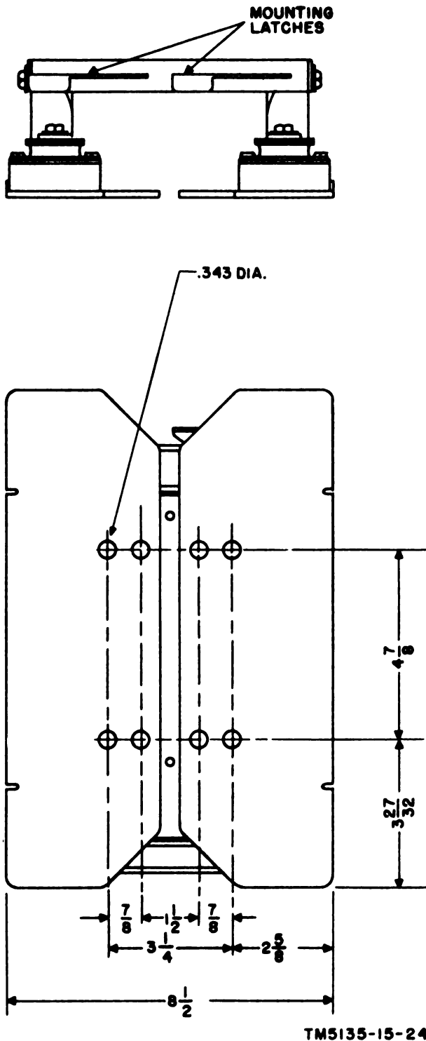
Figure 6. Mounting MT-791/U, mounting hole locations.
