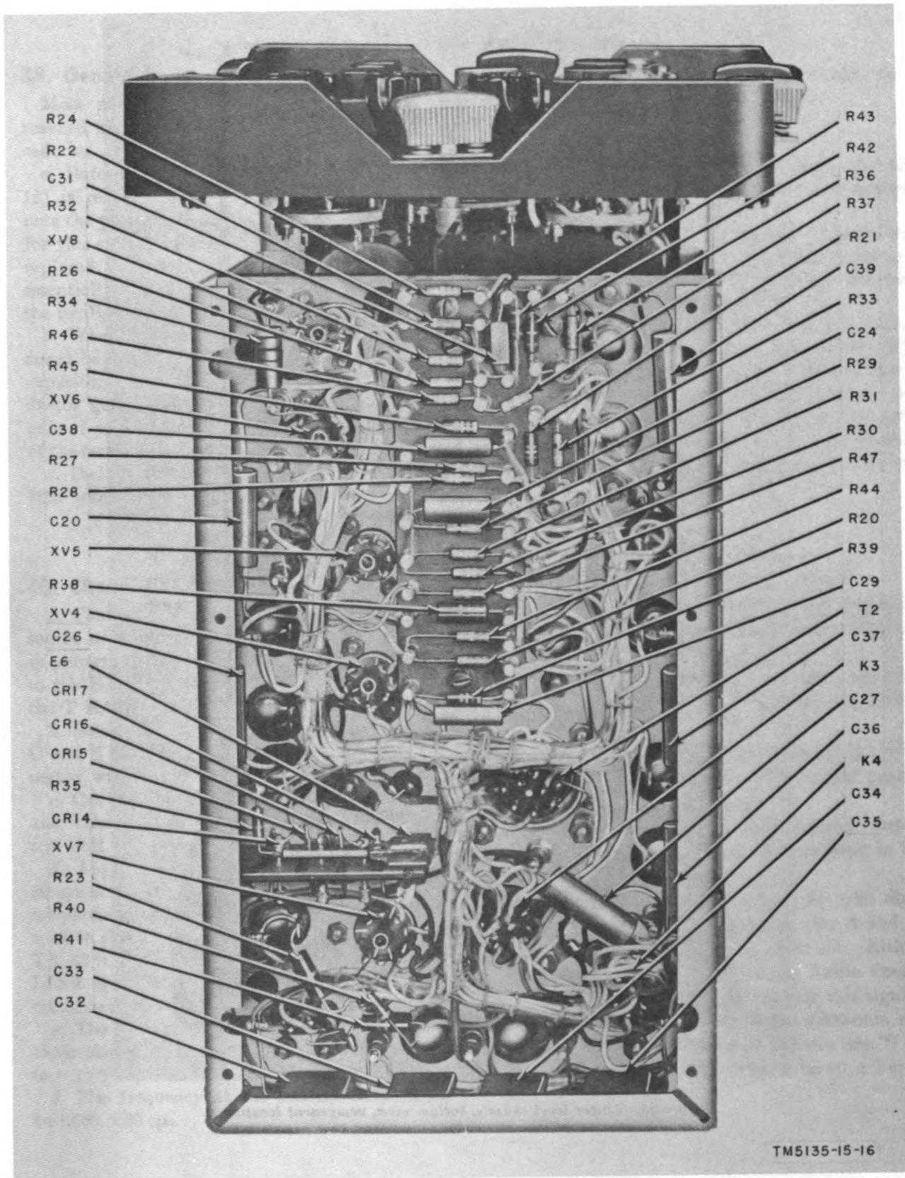
Figure 22. Upper level chassis, top view, component location.
