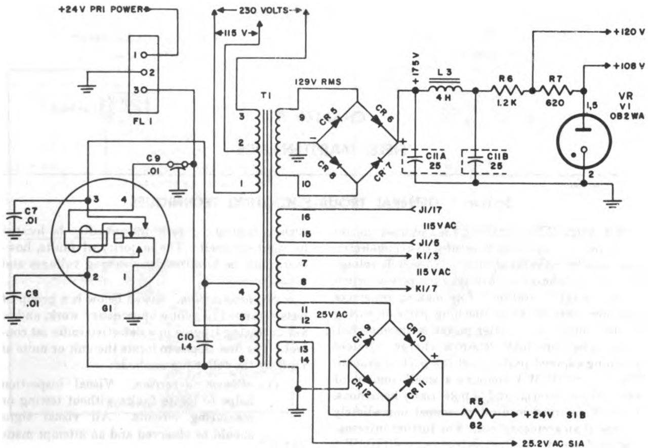
Figure 17. Power supply circuit.
