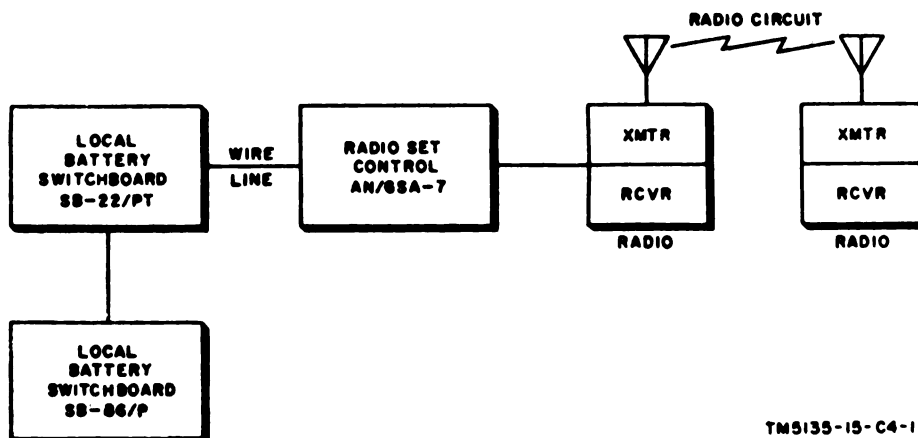
Figure 2.1. System application of Radio Set Control AN/GSA-7.
