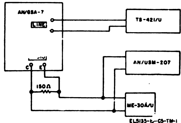
Fig. 24.1 Output level test, 1600 cycles.
