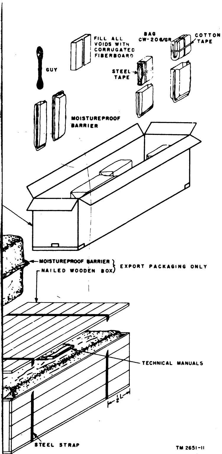
Antenna Group AN/GRA-12.
