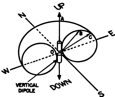
C. CROSS-SECTION WHEN ANTENNA IS VERTICAL
