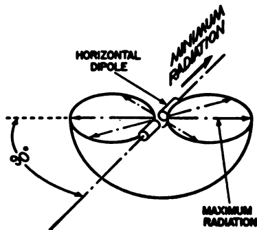
D. CROSS-SECTION WHEN ANTENNA IS HORIZONTAL
