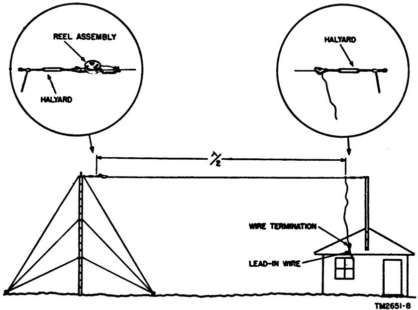
Figure 7. L-type antenna.
