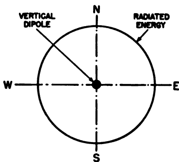
B. HORIZONTAL CROSS-SECTION SHOWING HORIZONTAL DIRECTIVITY OF VERTICAL DIPOLE
