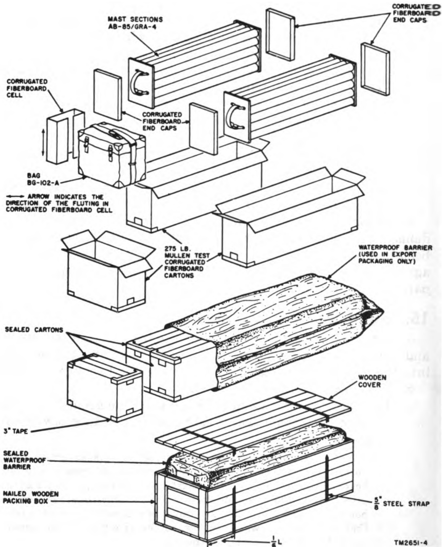
Figure 11. Packaging of Antenna Group AN/GRA-4.
