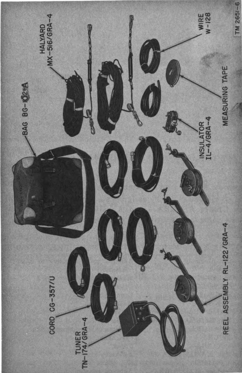
Figure 4. Antenna AS-244/GRA-4, components.
