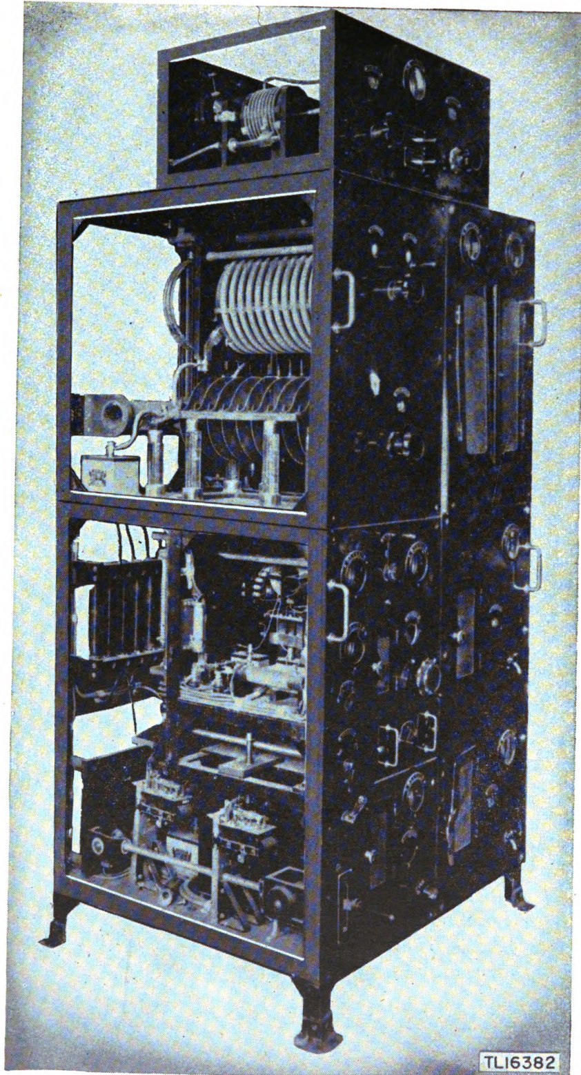
Model 95 Mark 4 Improvement 1 transmitter.
