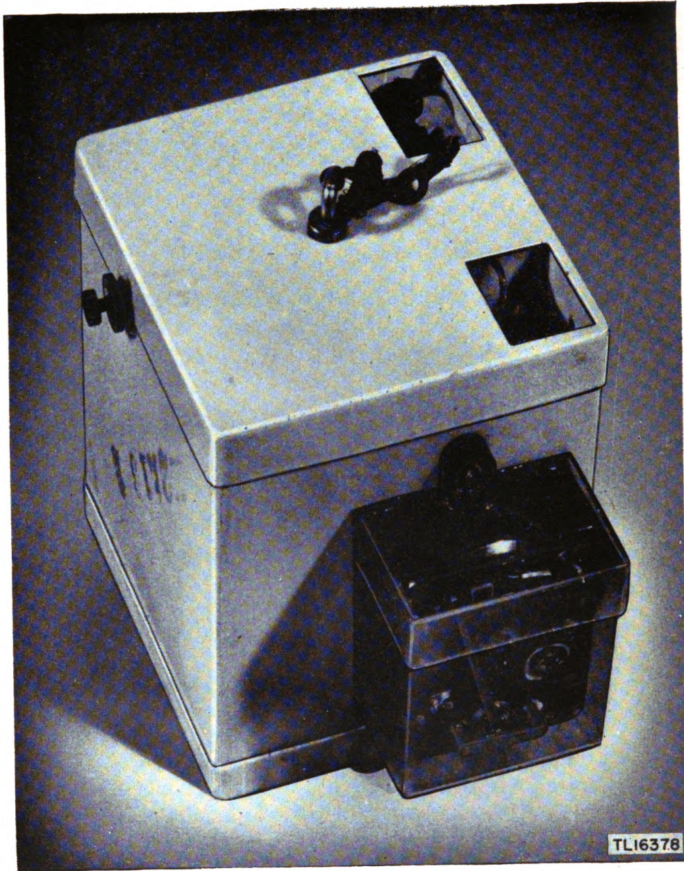
Radiosonde, showing barometer.
