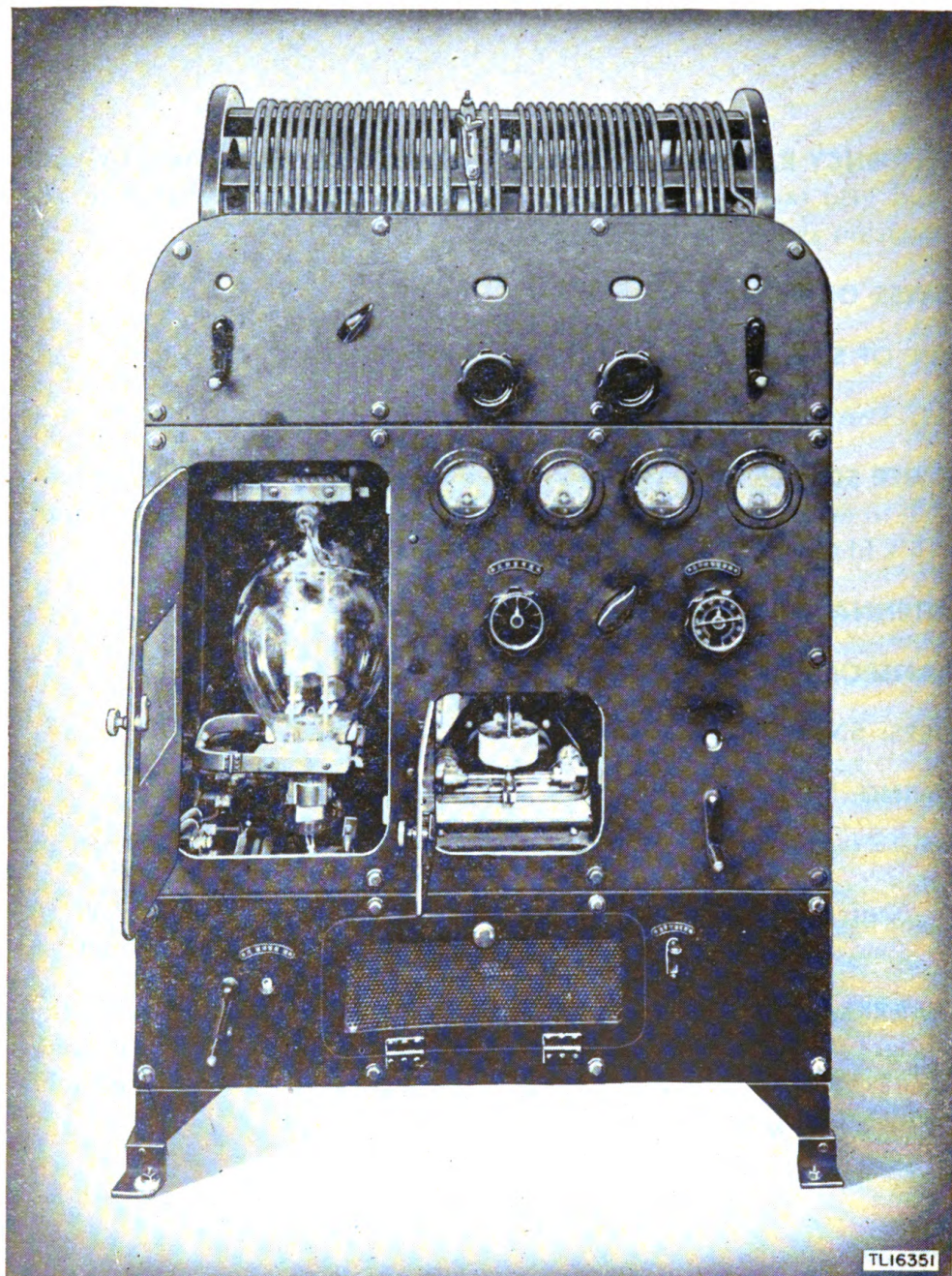
Model 92 Mark 3 Improvement 1 transmitter.
