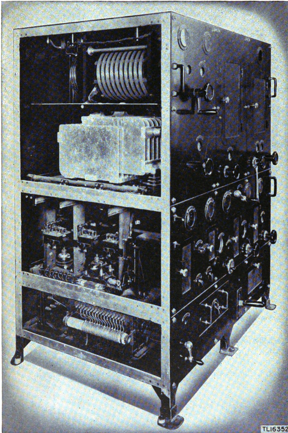
Model 95 transmitter.
