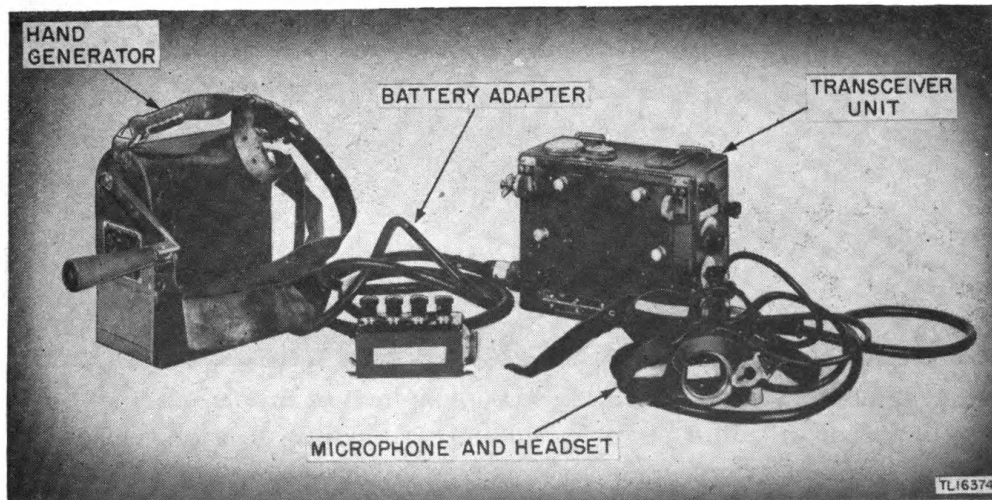
Model 97 Light Wireless Set, equipment interconnected.
