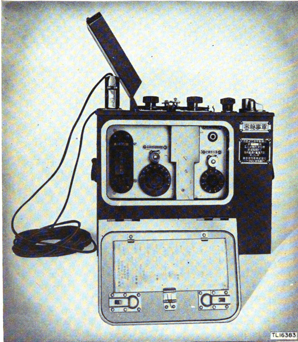
Mark 53 Type C Receiver.
