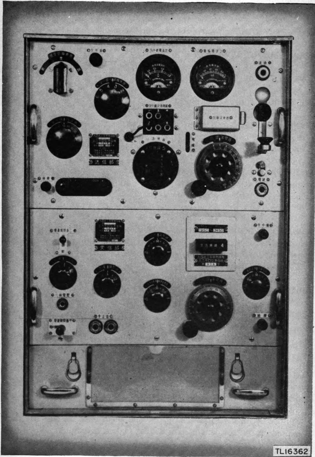
Model 94 Mark 3A Wireless Set: Mark 36 Type D Transmitter, Mark 36 Type D Receiver.
