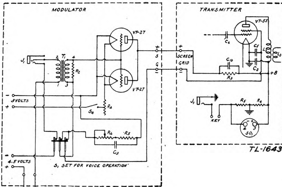
FIGURE 25.—Radio sets SCR-178 and SCR-179 (using BC-187 and BC-188), functional diagram, voice operation.
