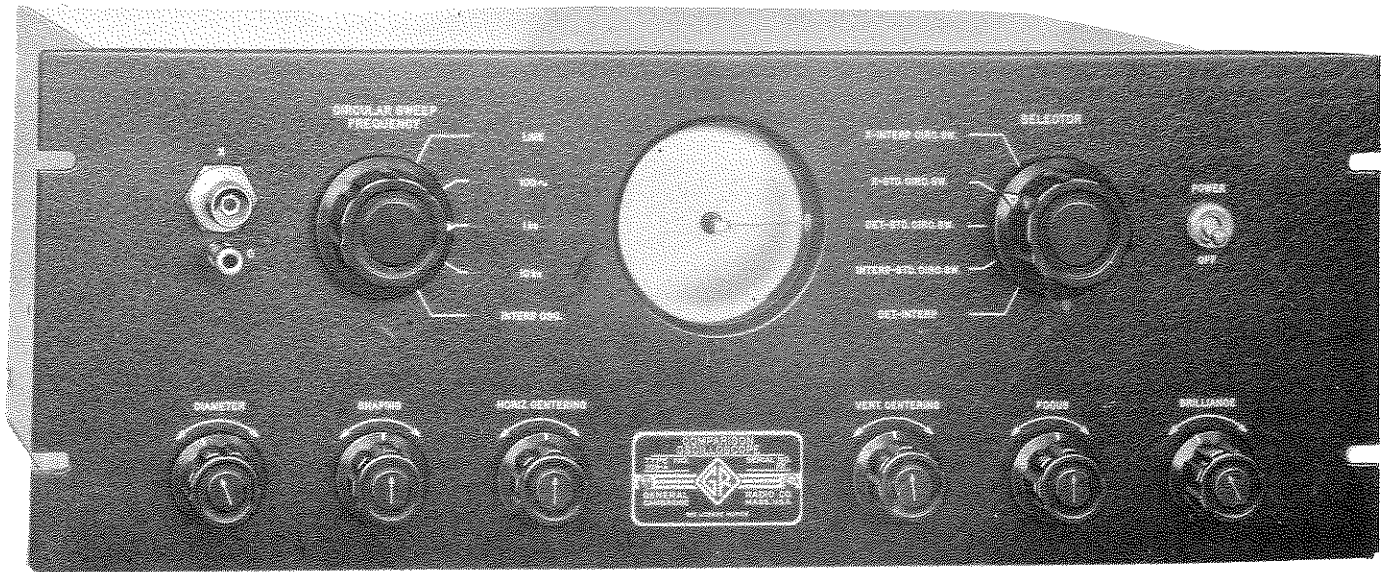
Figure 7. Panel View of the Type 1109-B Comparison Oscilloscope Showing All Controls.
