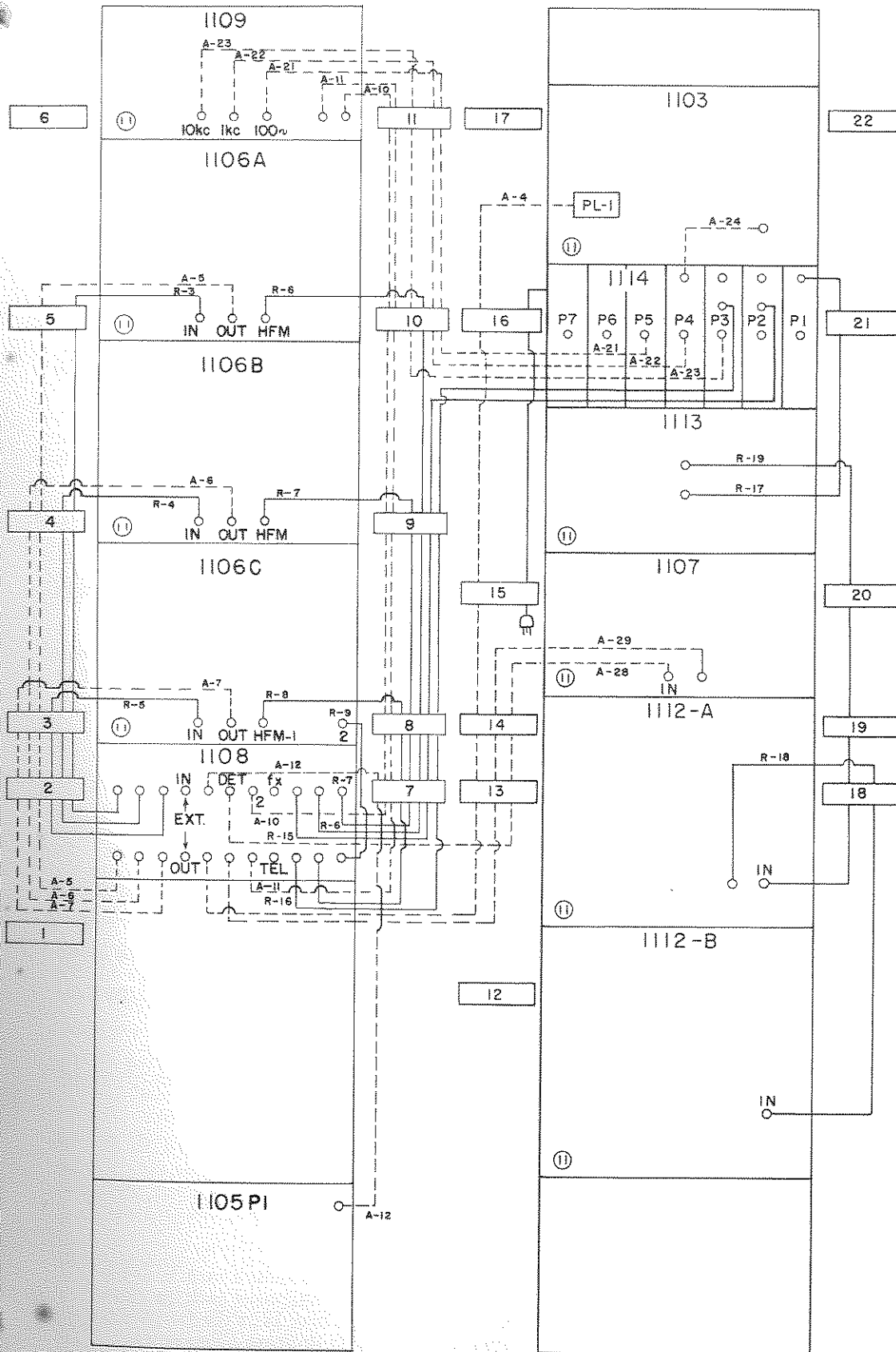
Figure 2. A rear view outline sketch of the complete Type 1120-A Frequency Standard and Type 1105-B Frequency Measuring Equipment showing the location and arrangement of the interconnecting cables.
