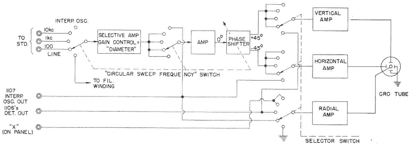
Figure 8. Functional Block Diagram of the Type 1109-B Comparison Oscilloscope.
