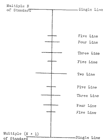
Figure 13. Division of a Standard-Frequency Interval by Multiple-Line Oscilloscope Patterns.
