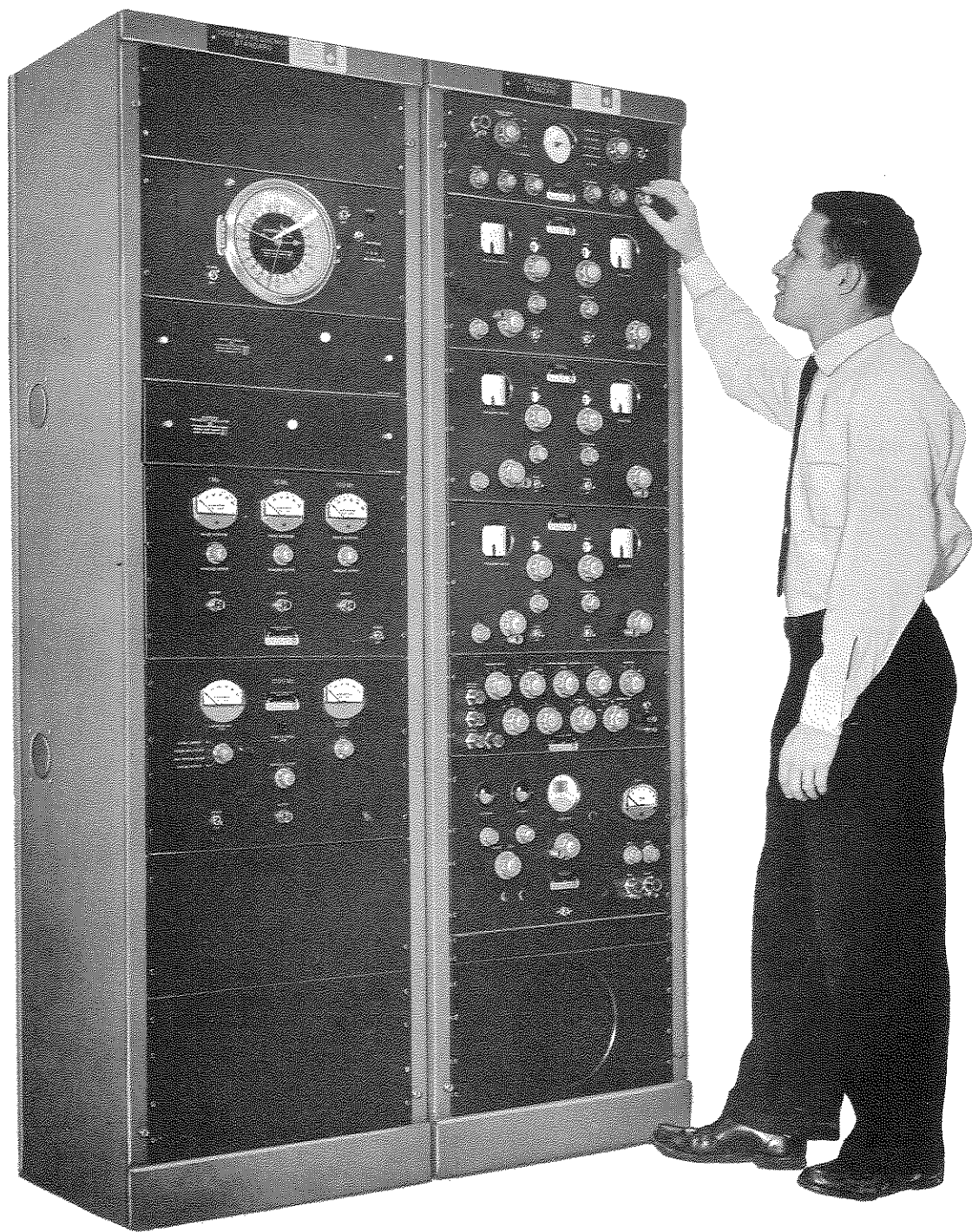
Figure 1. Type 1105-B Frequency Measuring Equipment (right) with Type 1120-AH Primary Frequency Standard.
