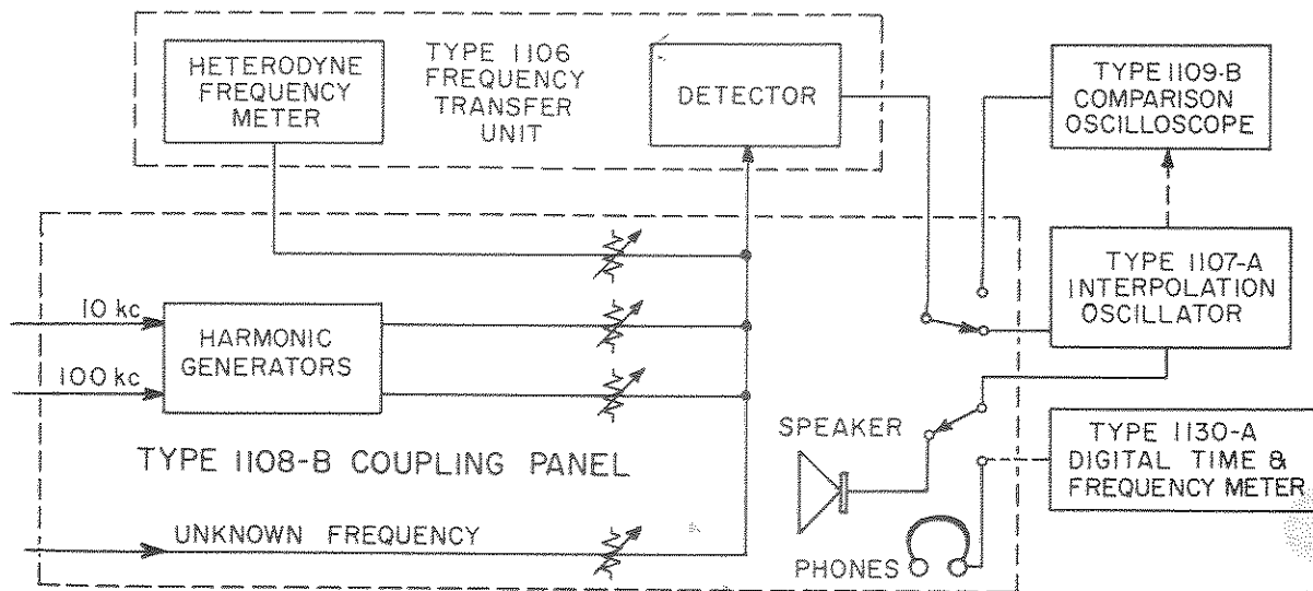
Figure 4. Block Diagram of the Type 1108-B Coupling Panel and associated equipment.
