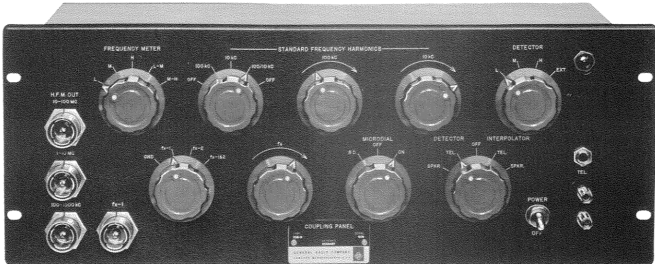
Figure 3. Panel View of the Type 1108-B Coupling Panel Showing All Controls.
