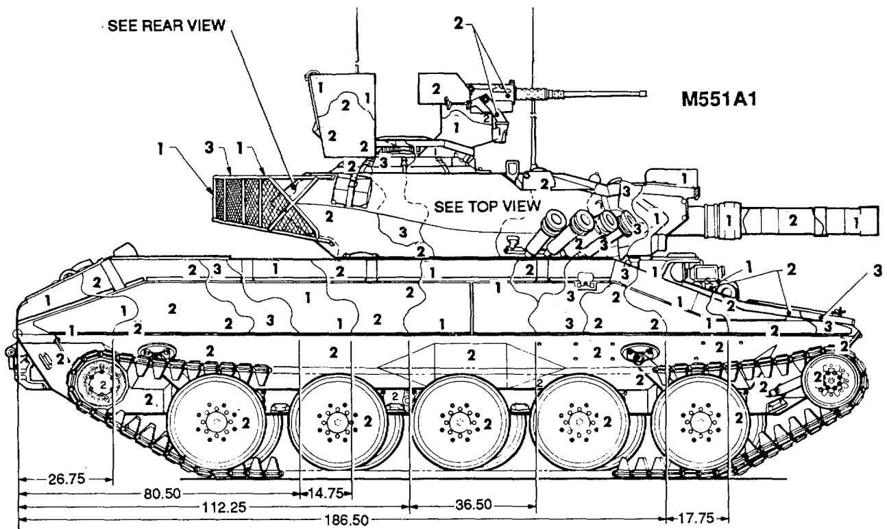
Figure 112. Armored, reconnaissance/airborne vehicles full tracked, M551A1. (1 of 2)
