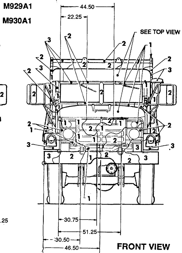
Figure 70. Truck, dump: 5-ton, M929A1 and M930A1. (2 of 2)
