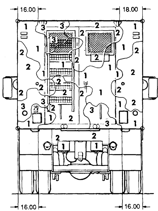
Figure 65. Truck, van, expansible: 5-ton, M820A2. (1 of 2)
