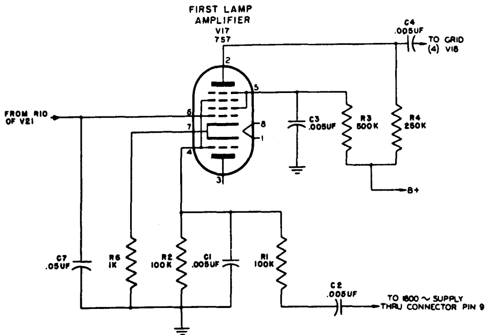
Figure 68. First lamp amplifier, exciter lamp supply.
