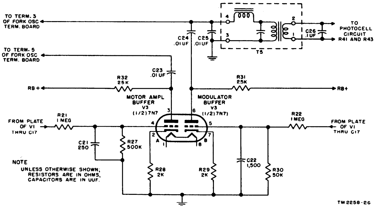
Figure 37. Output buffers, unsealed fork oscillator unit.
