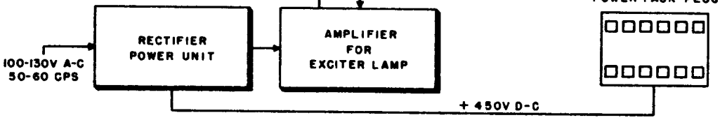
Figure 31. Facsimile Transceiver TT-1(*)/TXC-1, transmitting block diagram.
