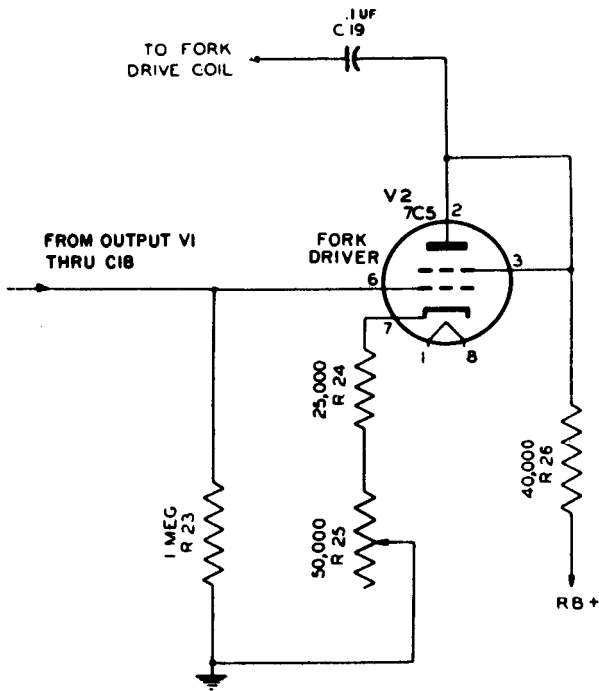
Figure 36. Fork driver, unsealed fork oscillator unit.
