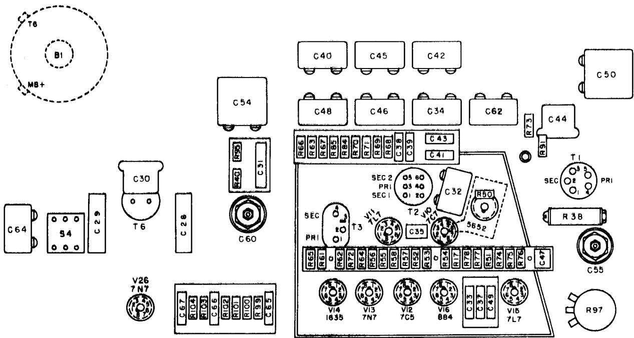
Facsimile Transceiver TT-1D/TXC-1, bottom view, parts identification.
