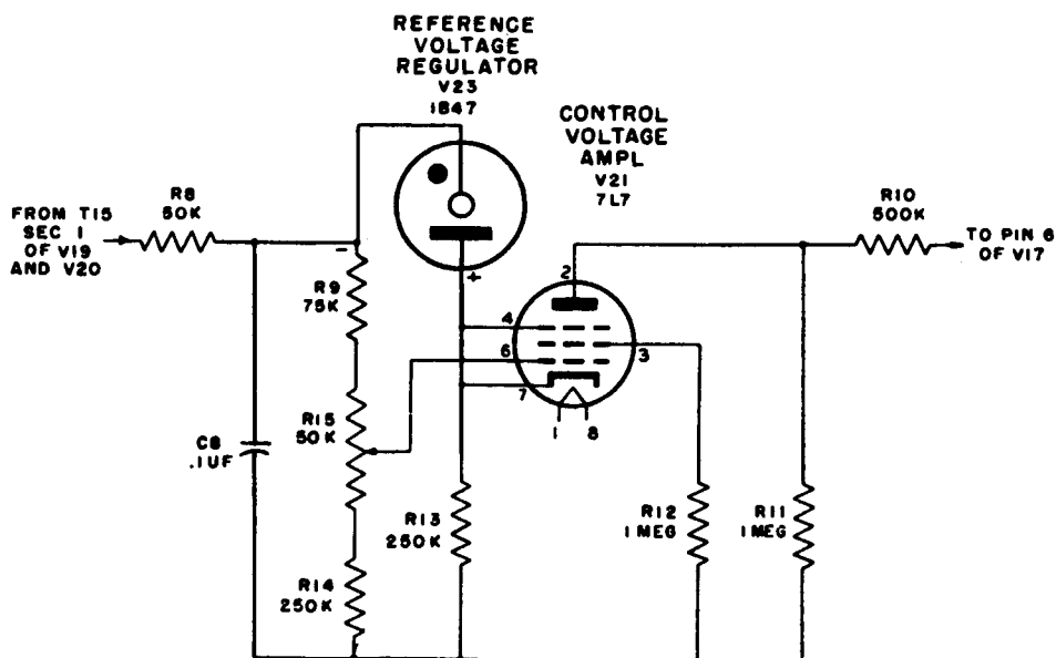
Figure 71. Control voltage amplifier, exciter lamp power supply, rectifier power unit PP-86/TXC-1.
