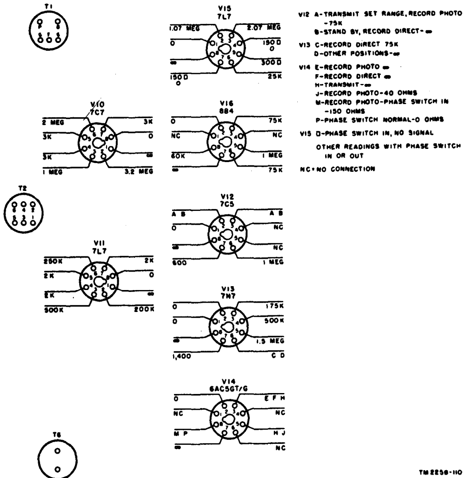
Figure 86. Resistance measurement chart, stages V10 through V16, Facsimile Transceivers TT-1/TXC-1 and TT-1A/TXC-1.
