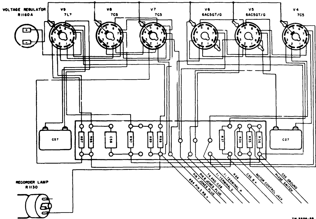
Figure 178. Facsimile Transceivers TT-1/TXC-1 and TT-1A/TXC-1, regulator panel wiring diagram.
