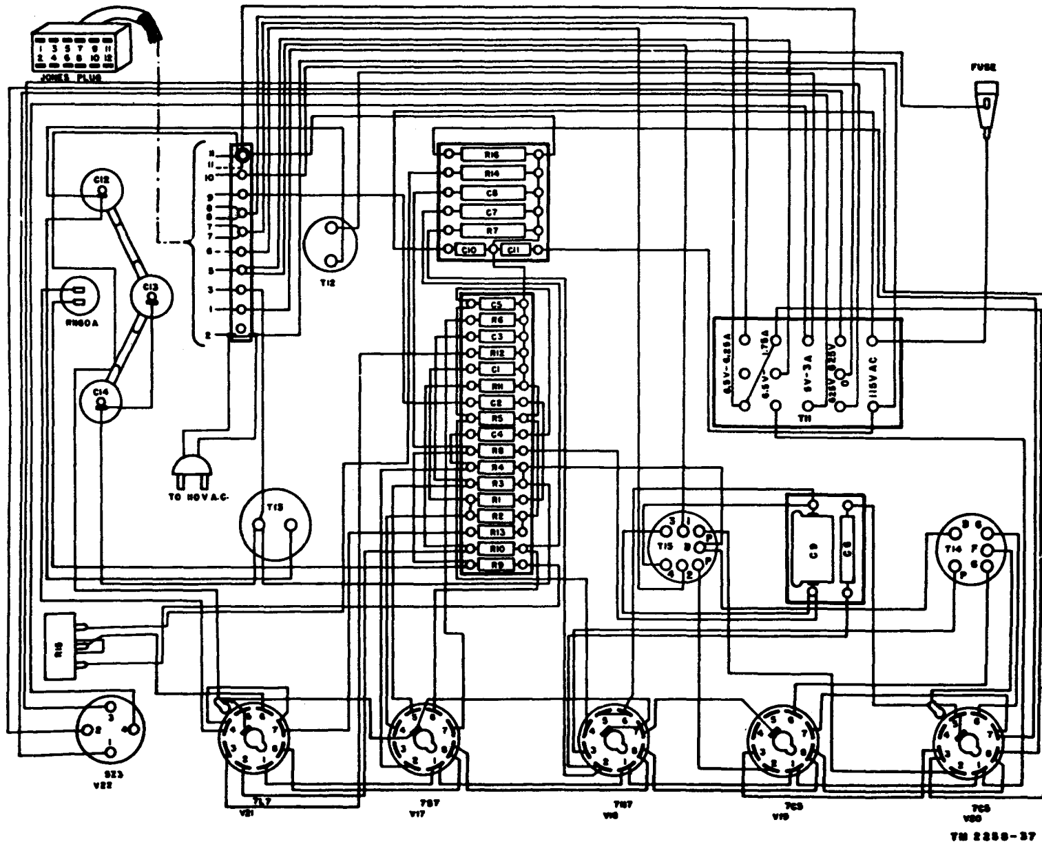
Figure 176. Rectifier Power Unit PP-88/TXC-1, wiring diagram.
