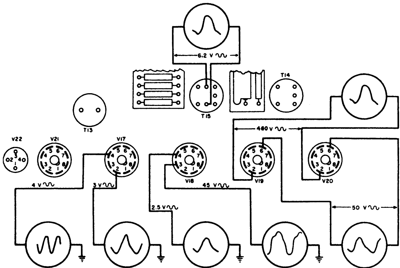
Figure 79. Signal-tracing chart, multivibrator stage, Facsimile Transceivers TT-1D/TXC-1, TT-1E/TXC-1 and TT-1/TXC-1.
