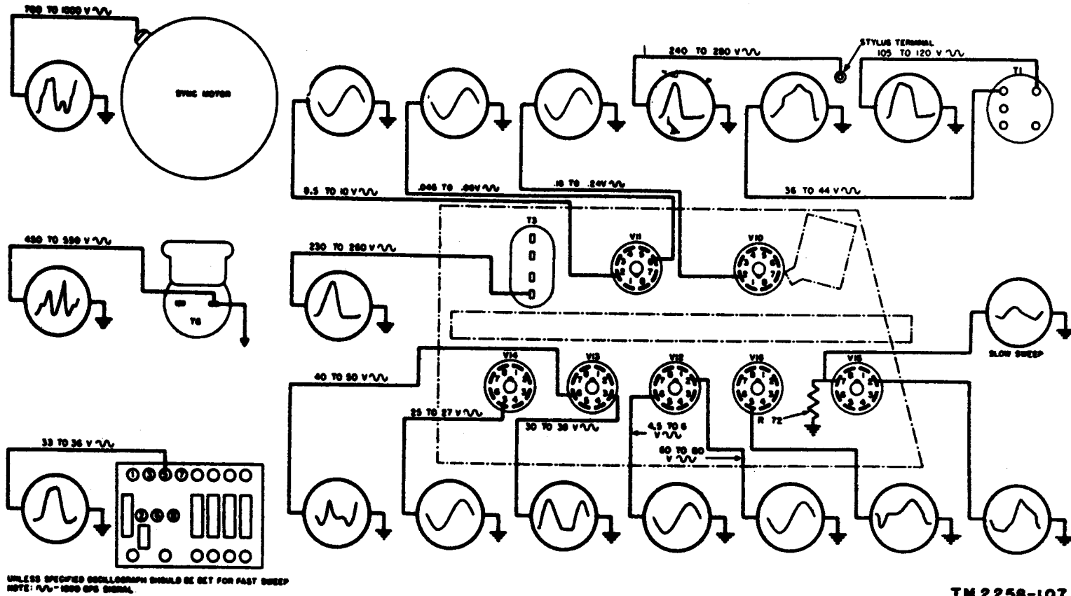
Figure 77. Signal-tracing chart, Facsimile Transceiver TT-1A/TXC-1.
