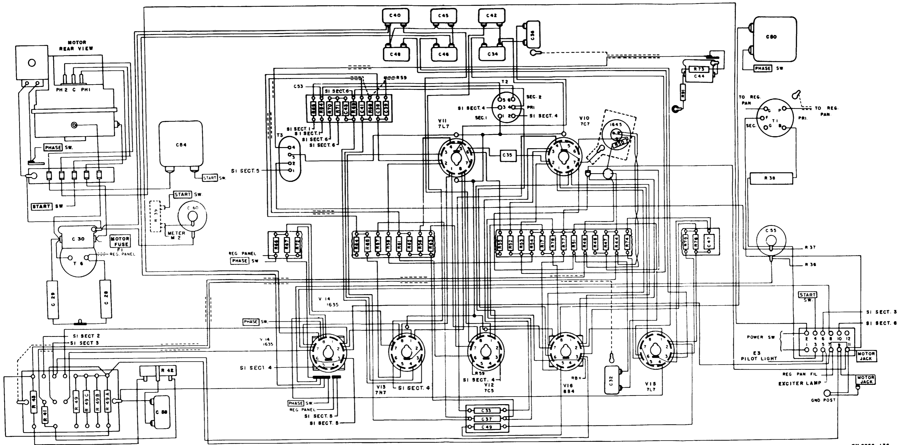
Figure 185. Facsimile Transceiver TT-1B/TXC-1, chassis wiring diagram.
