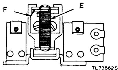
Figure 109. Start magnet.
