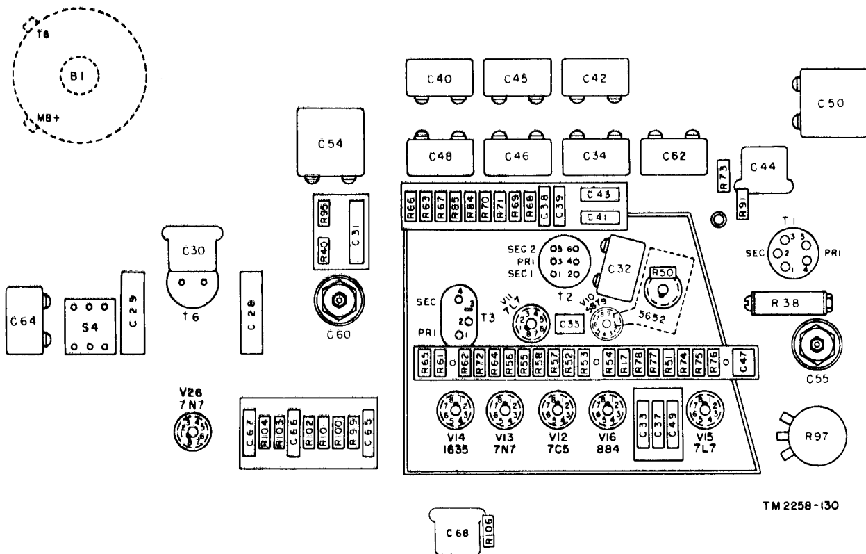
Figure 132. Facsimile Transceiver TT-1E/TXC-1, bottom view, parts identification.
