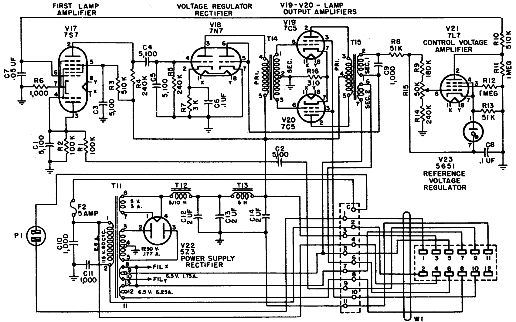
Figure 160. Rectifier Power Unit PP-86A/TXC-1, furnished on Order No. 6457-Phila-51, schematic diagram.
