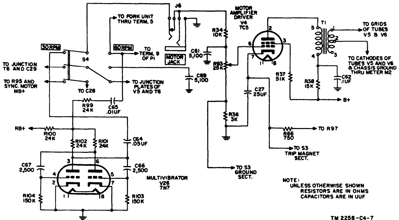
Figure 43. Multivibrator and motor amplifier driver Facsimile Transceiver TT-1F/TXC-1.
