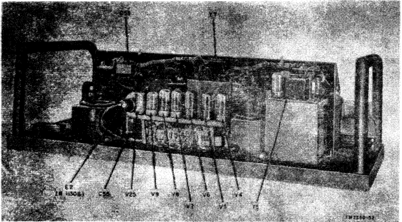
Figure 130. Facsimile Transceiver 11-10/1A0-1, rear view, parts identification.
