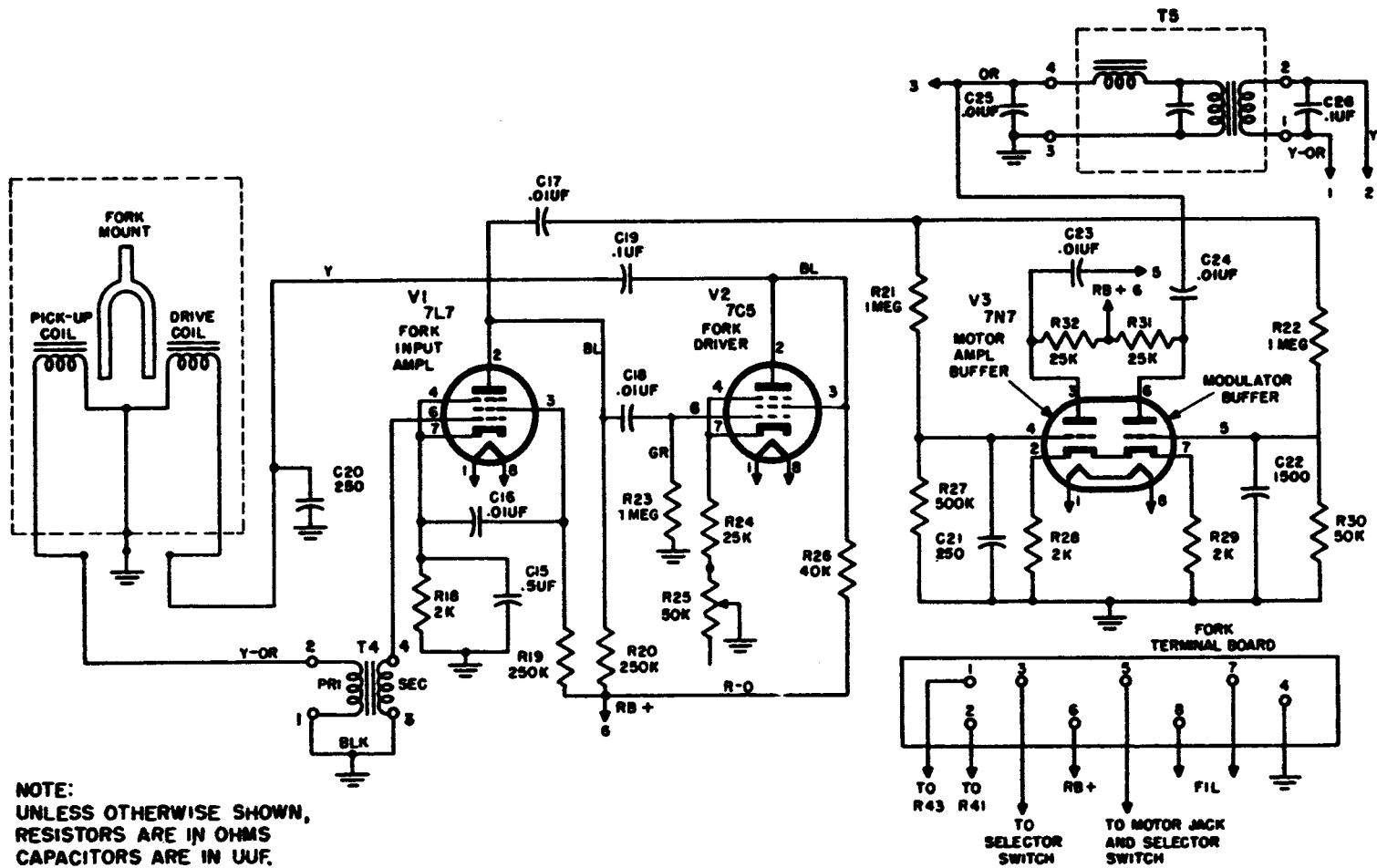
Figure 167. Unsealed fork oscillator unit, schematic diagram.
