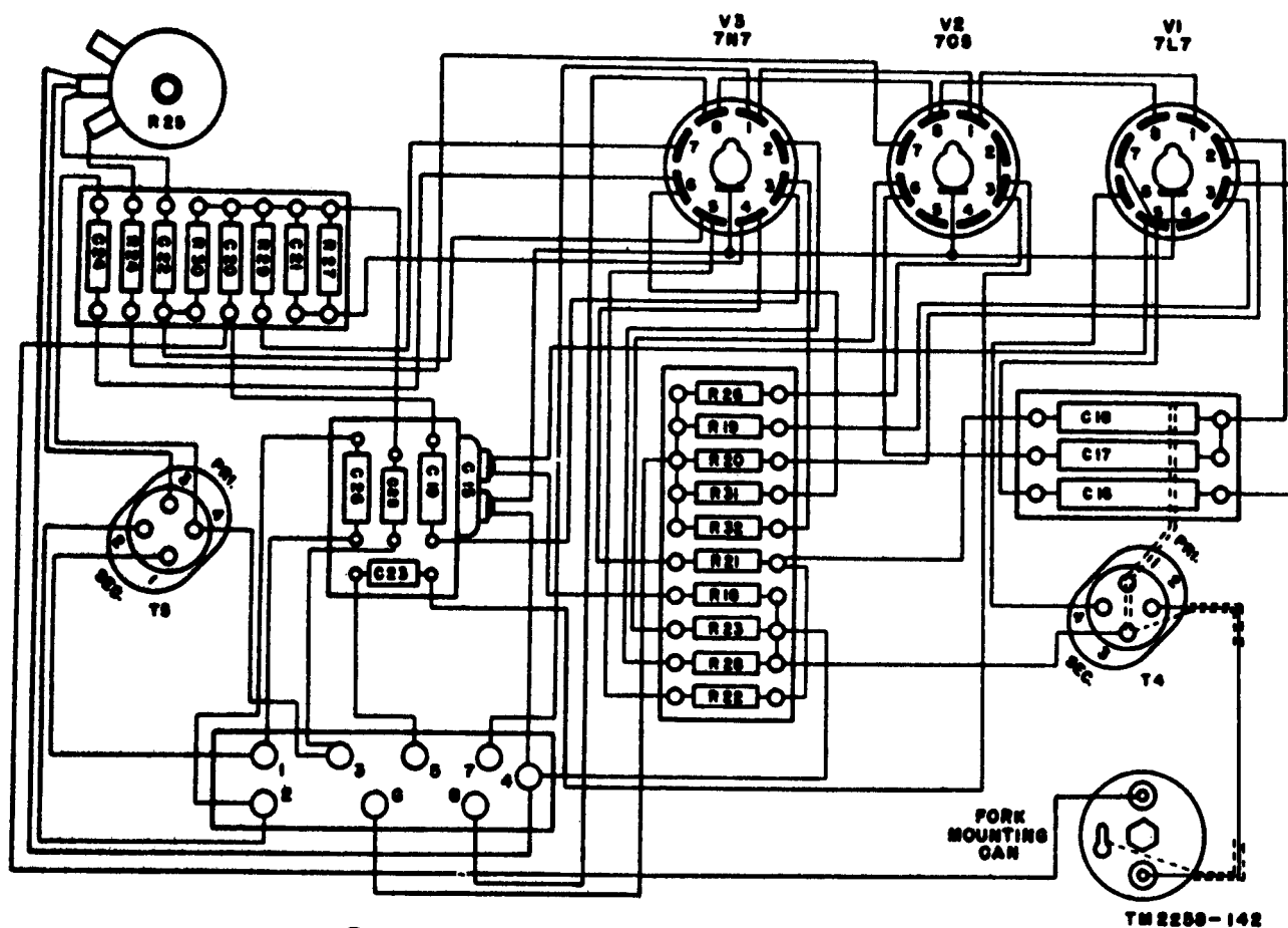
Figure 178. Unsealed fork oscillator unit, wiring diagram.
