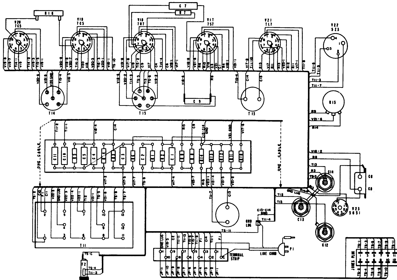
Figure 176. Rectifier Power Unit PP-86A/TXC-1, furnished on Order No. 6437-Phila-51, wiring diagram.
