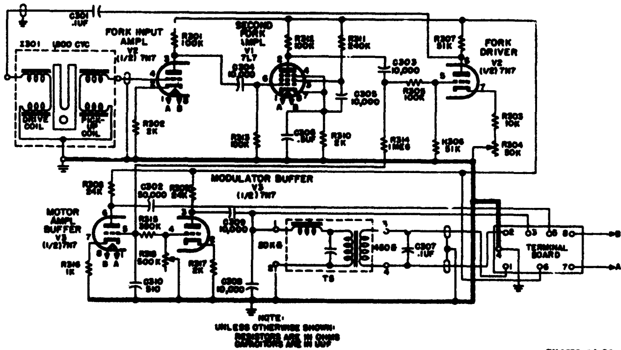
Figure 174. Sealed fork oscillator unit, schematic diagram.
