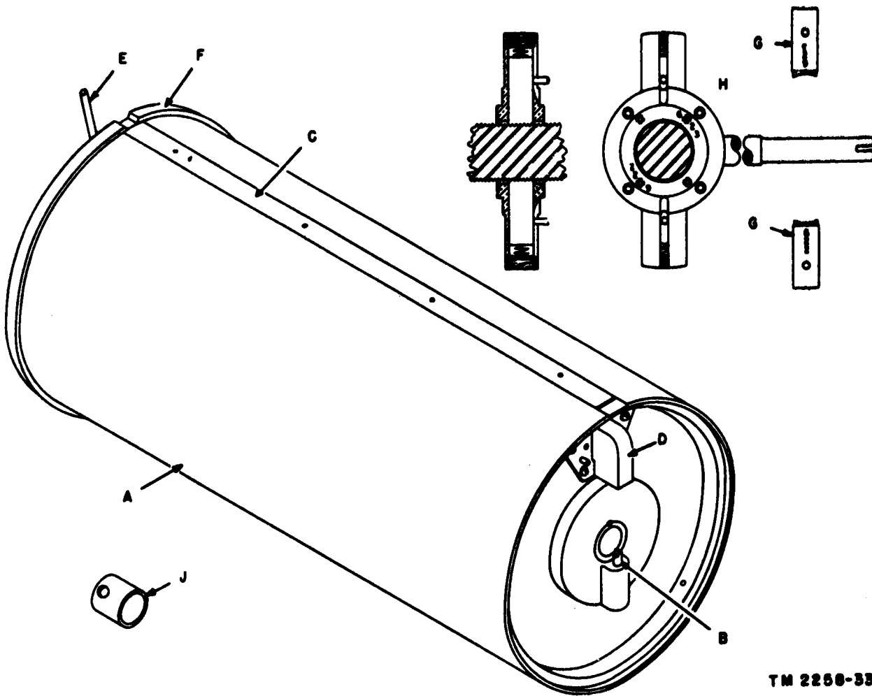
Figure 117. Drum assembly, Facsimile Transceivers TT-1/TXC-1, TT-1A/TXC-1, and TT-1B/TXC-1.
