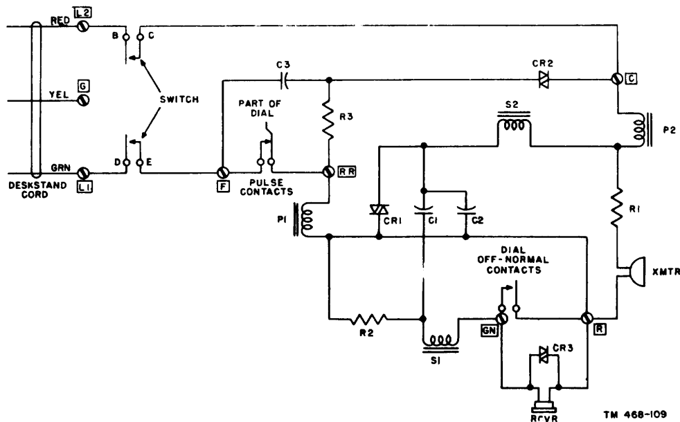
Figure 66. Dialing circuit, schematic.
