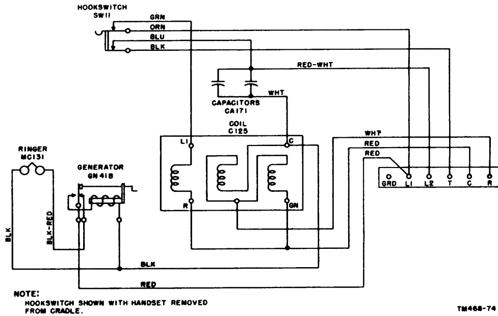
Figure 100. Telephone TA-168/U (manual operation), wiring diagram.
