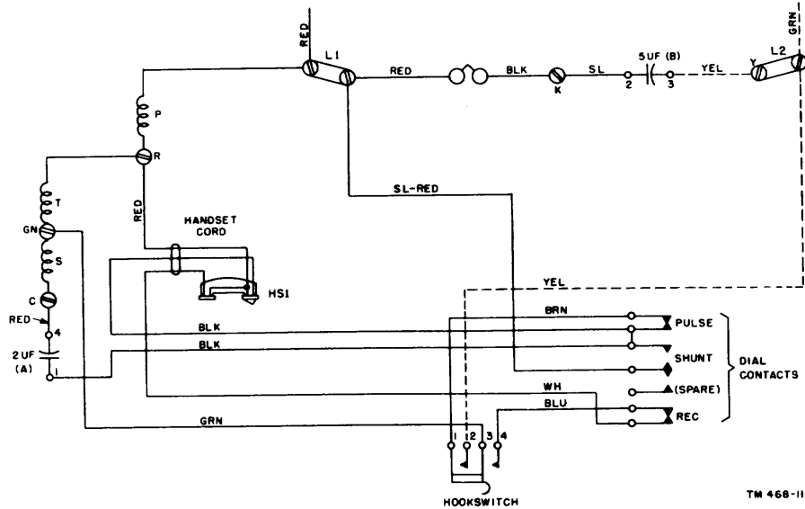
Figure 72. Telephone TP-6-A, with dial, schematic diagram.
