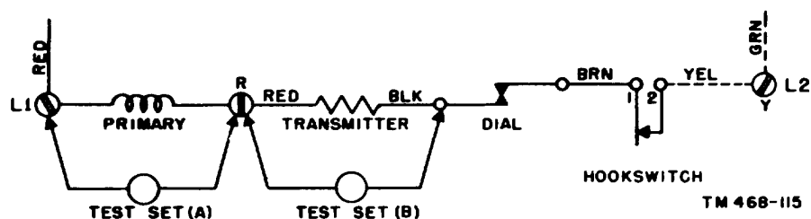
Figure 76. Telephone TP-A, tea for short-circuited primary winding and transmitter, wiring diagram.
