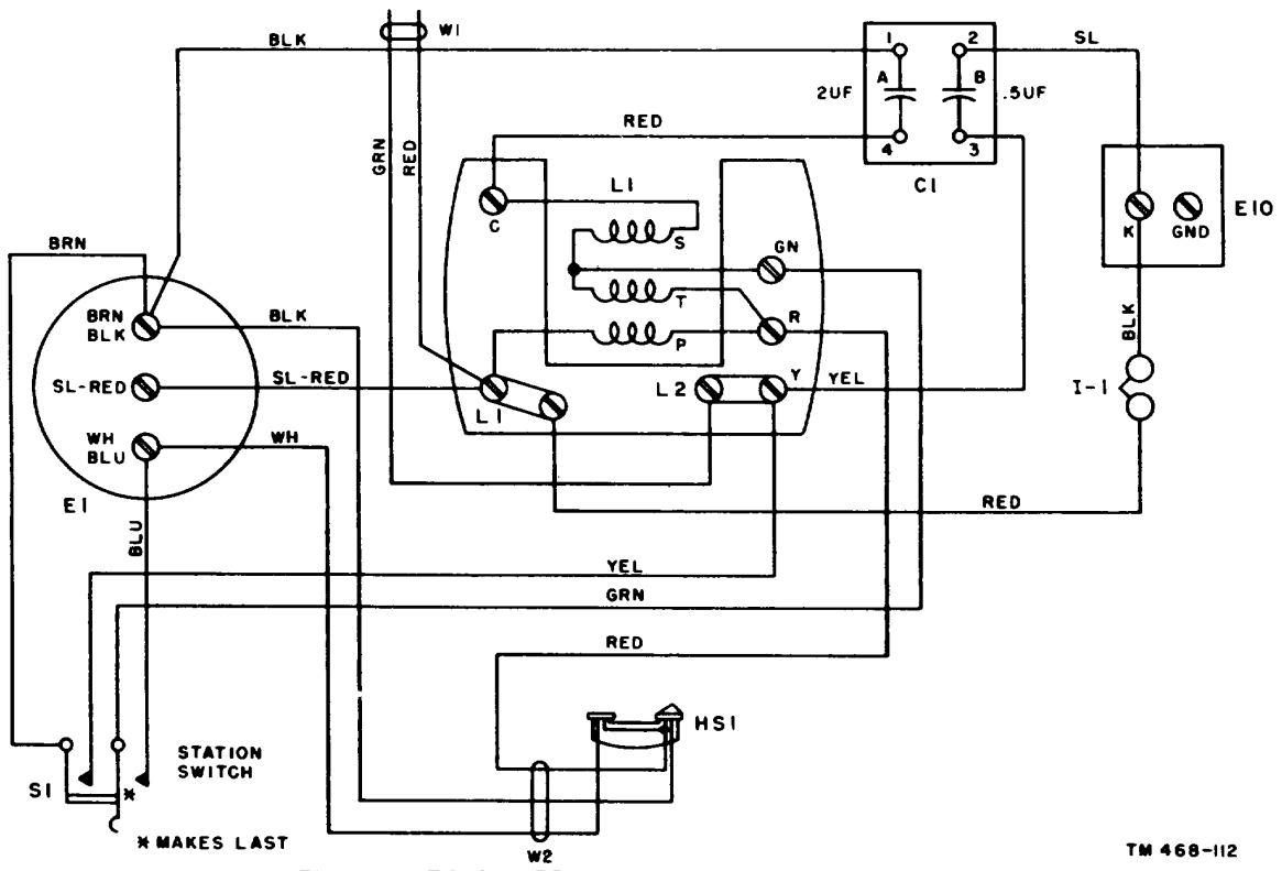
Figure 73. Telephone TP-6-A, manual operation, wiring diagram.
