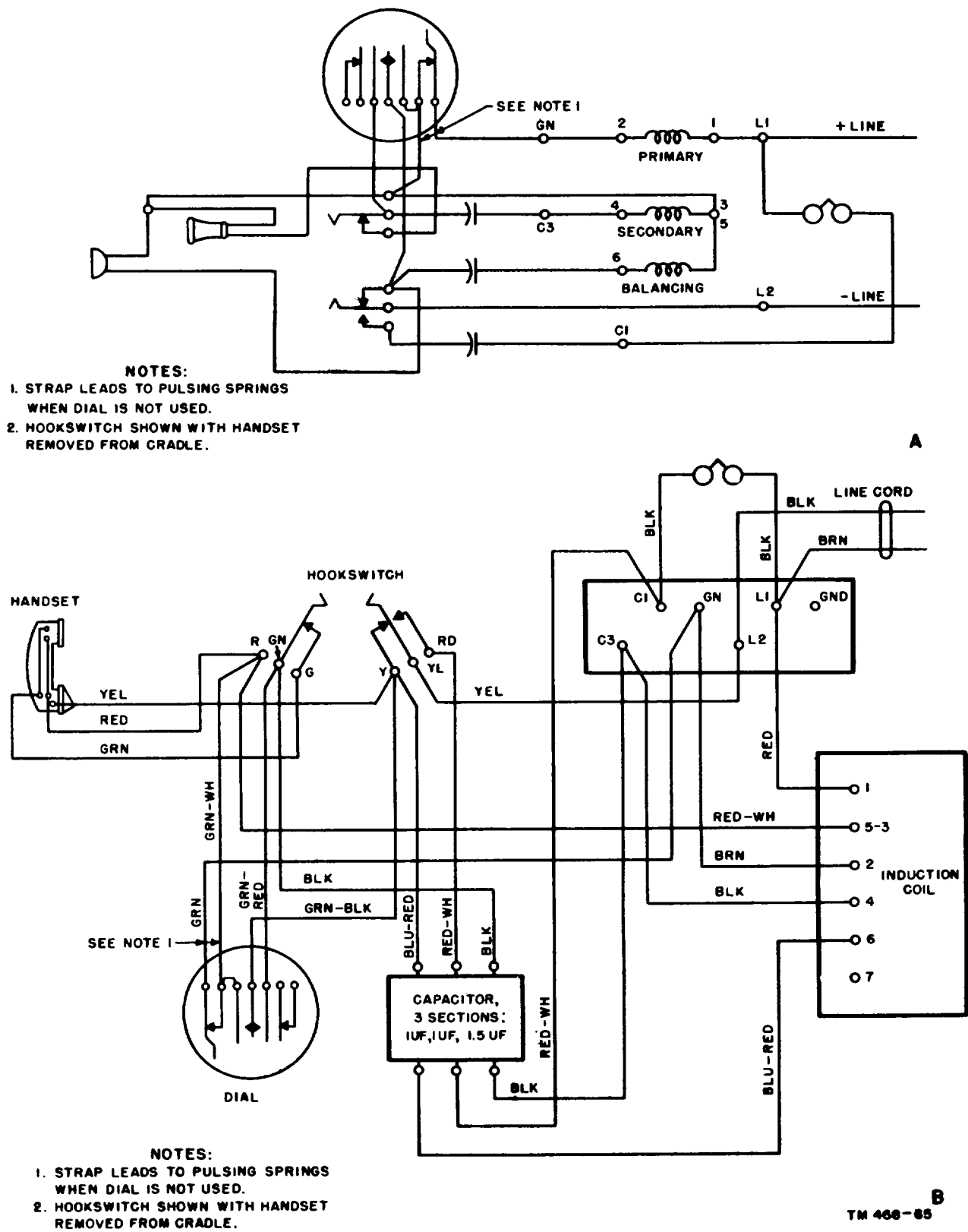
Figure 92. Telephone TA-LOS/FTC (Kellogg 9 BAX). schematic (A) and wiring (B) diagrams.
