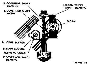
Figure 71. Lubrication points for Dial TA-45/GT.
