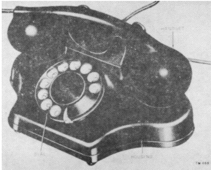
Figure 6. Telephone TA-102/FTC (Kellogg No. 925BAX), arranged for dial operation.
