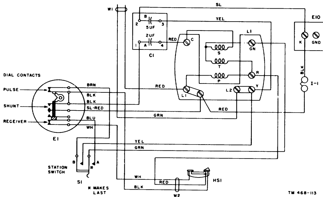
Figure 73. Telephone TP-6-A, manual operation, wiring diagram.
