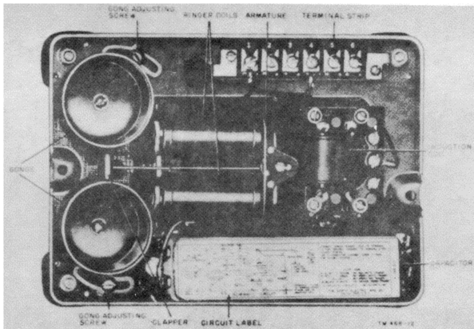
Figure 11. Telephone TP-6 (North Elec Mfg No. H-600SL and No. 3H6SL), with base plate open, showing locations of parts
