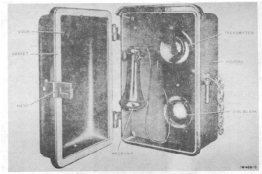
Figure 20. Telephone TA-105/FTC, guard and fire telephone.
