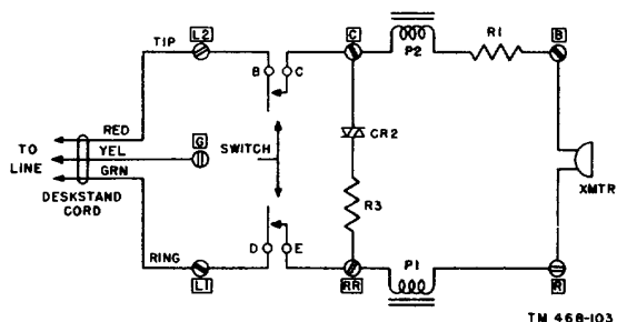
Figure 60. Transmitter circuit, manual, schematic.
