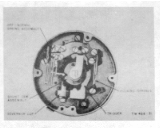
Figure 31. Dial TA-45/IGT (Telephonic), rear view, showing location of parts.
