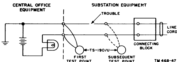
Figure 81. Method of testing for a line open.
