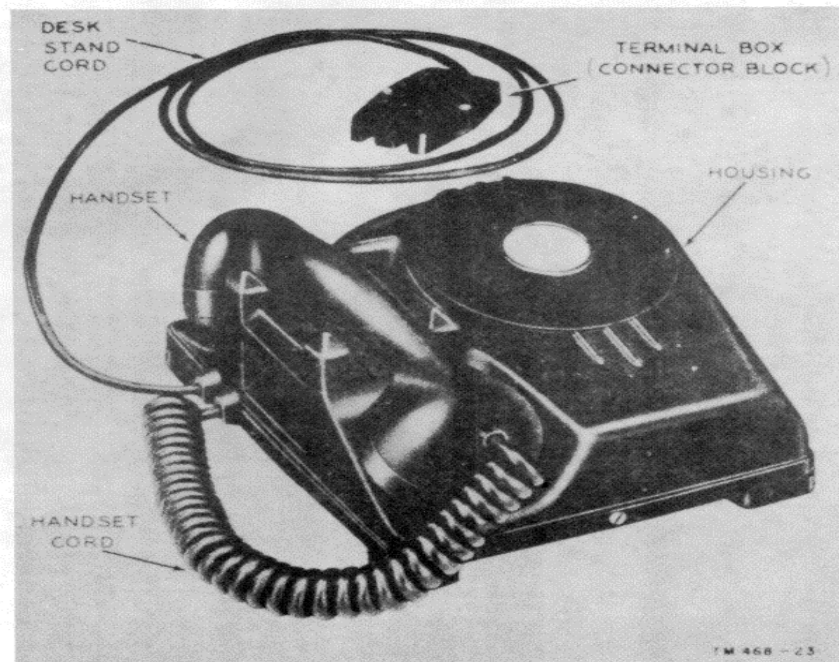
Figure 22. Telephone TA-166/U, arranged for manual operation.
