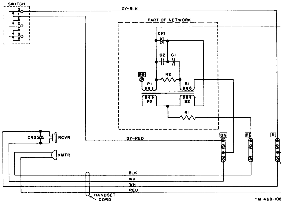
Figure 65. Receiver circuit, manual, wiring.
