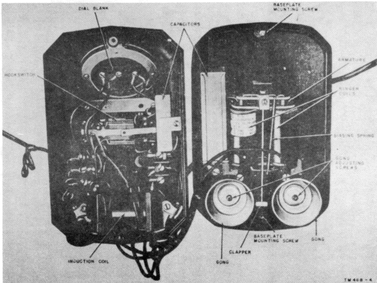
Figure 5. Telephone TA-101/FTC (Auto Elec No. 40), with base plate open
