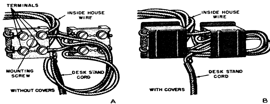
Figure 48. WECO 11-type connecting block.
