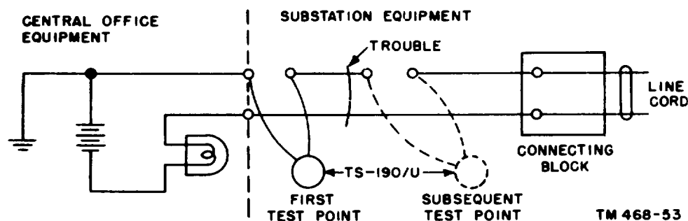
Figure 82. Testing for a line short.
