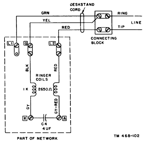
Figure 59. Ringer circuit, wiring.
