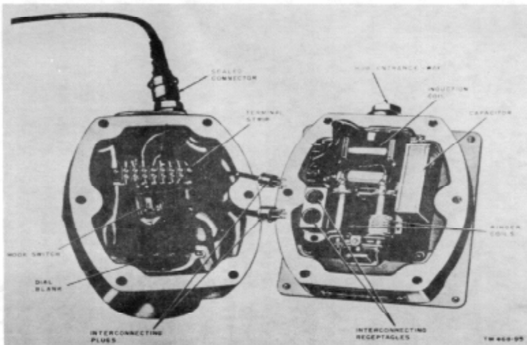
Figure 43. Telephone Set TA-212/U, with cover open, showing location of parts.
