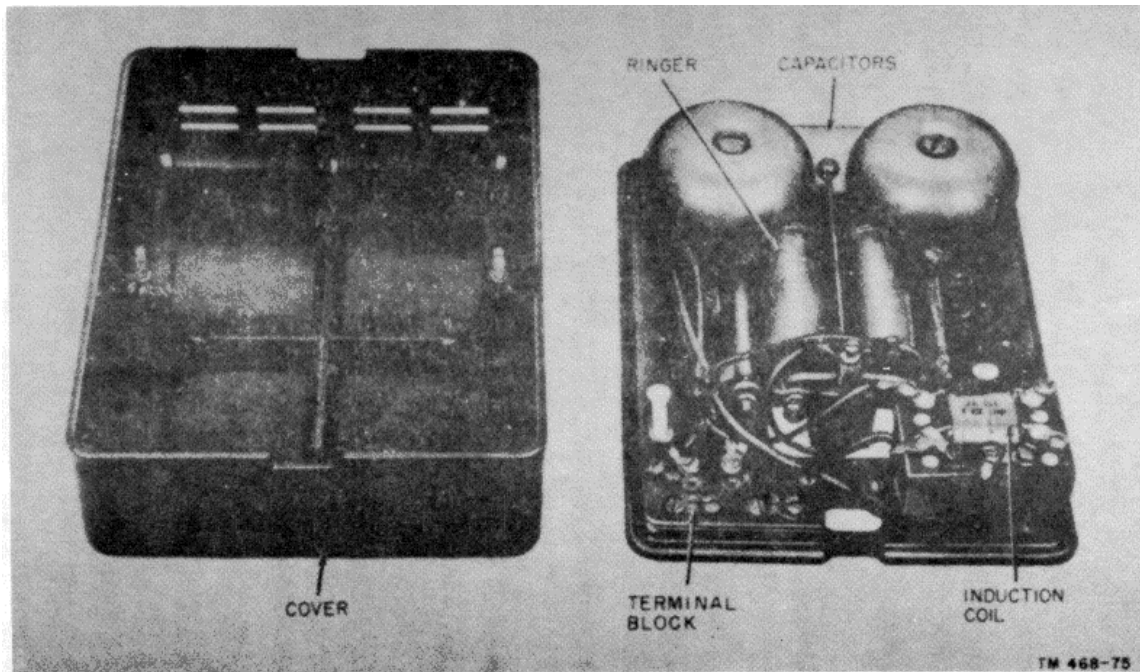
Figure 46. Bell box, WECO. No. 684A, showing location of parts.
