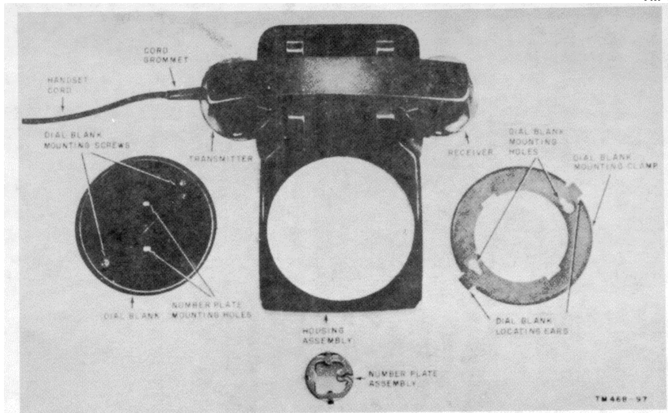
Figure 34. Telephone Set TA-236/FT, housing assembly
