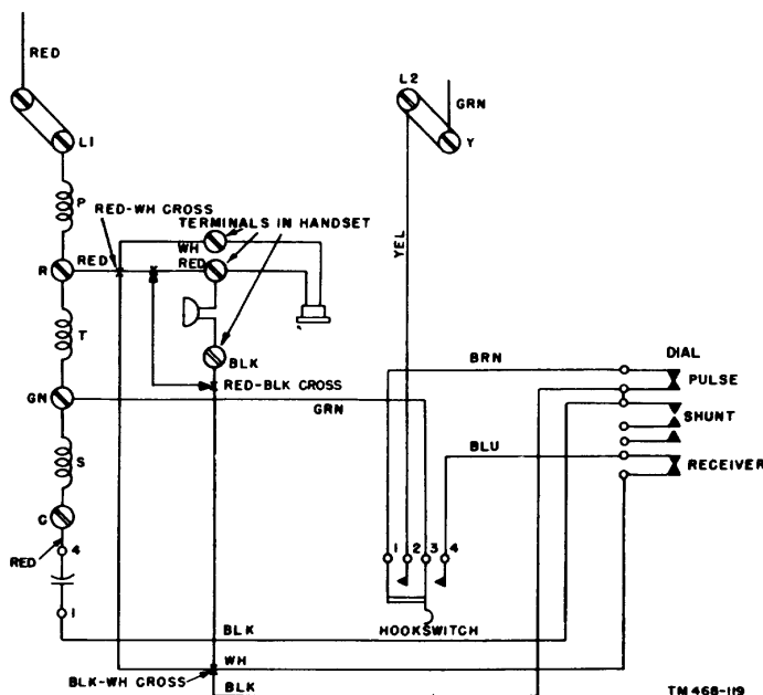
Figure 80. Telephone TP-A, schematic diagram showing crossed leads.
