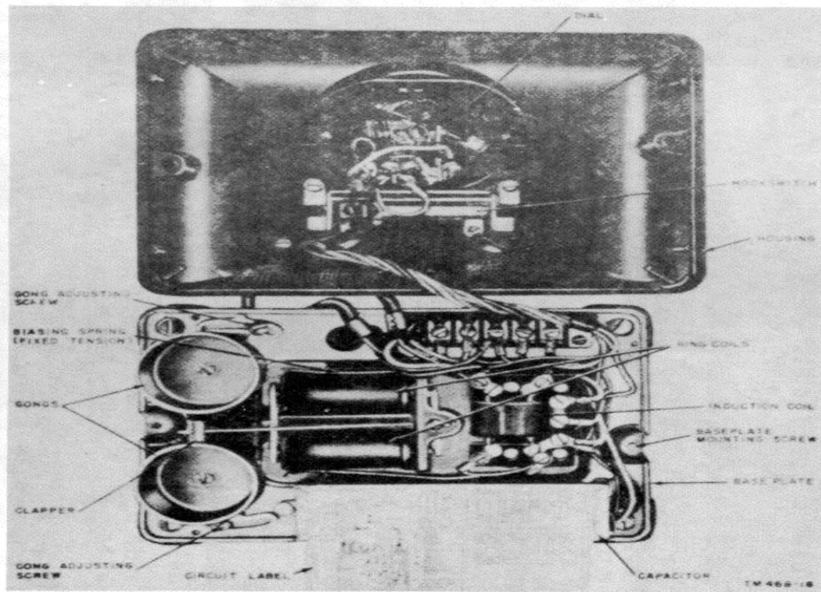
Figure 19. Telephone Set TA-107/FTC, with base plate open.
