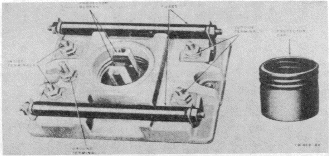
Figure 52. WECo. No. 98A protector, for inside installation.
