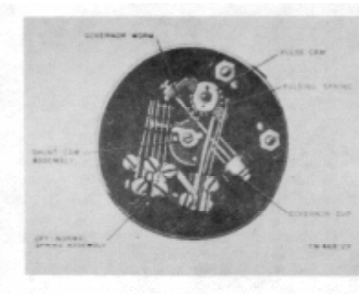
Figure 30. Dial TA-45(*)/GT (Auto Elec), rear view.
