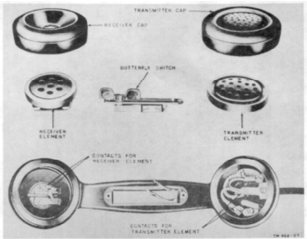
Figure 27. Handed TS-12-F, exploded view.
