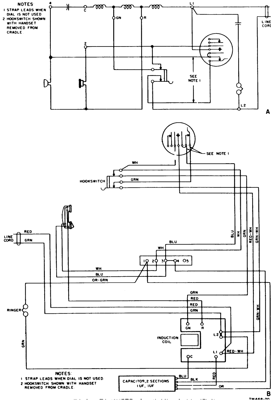
Figure 96. Telephone TA-107/FTC, schematic (A) and wiring (B) diagrams.
