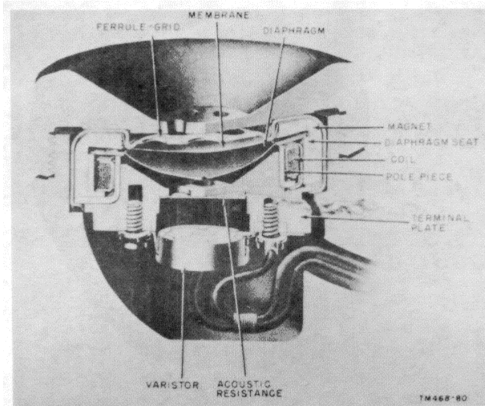
Figure 38. Receiver unit for Telephone Set TA-236/FT, sectional view.
