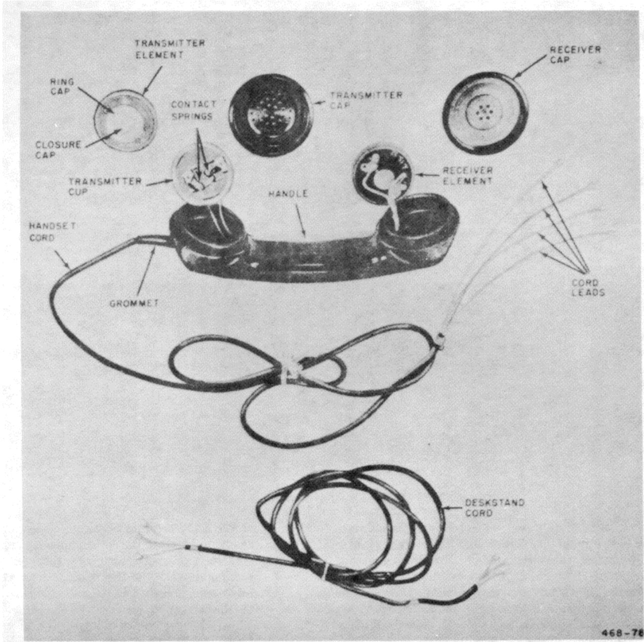
Figure 36. Handset for Telephone Set TA-236/FT, partially disassembled.
