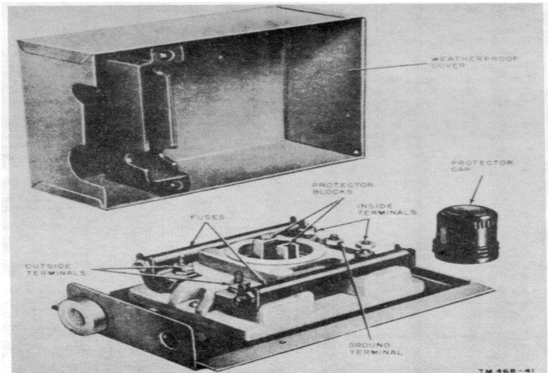
Figure 53. Protector AREA (WECo. No. 1093A), for outside installation.
