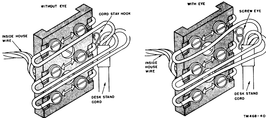
Figure 49. WECO 12-type connecting block.
