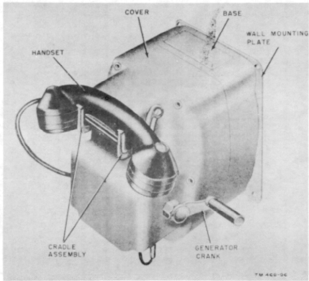
Figure 44. Telephone Set TA-213/U, less Battery Box CY-1149.
