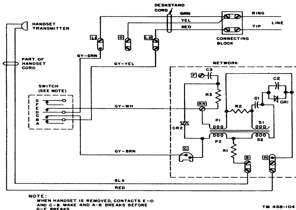
Figure 61. Transmitter circuit, manual, wiring.
