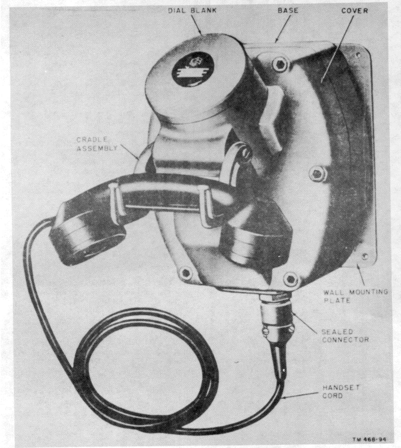
Figure 42. Telephone Set TA-212/ U, explosionproof wall-type telephone for common-battery use.
