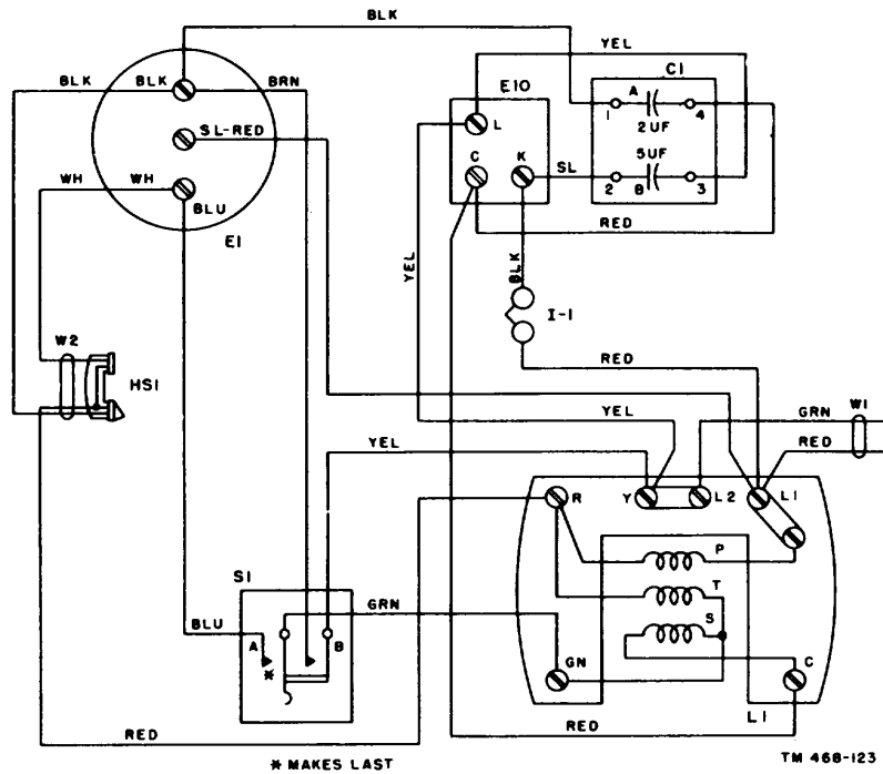
Figure 100. Telephone TA-168/U (manual operation), wiring diagram.
