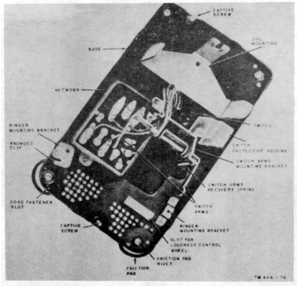
Figure 35. Telephone Set TA-236/FT, base plate assembly
