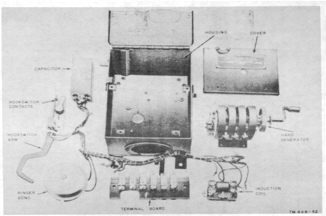
Figure 25. Component of Telephone Box EE-91.
