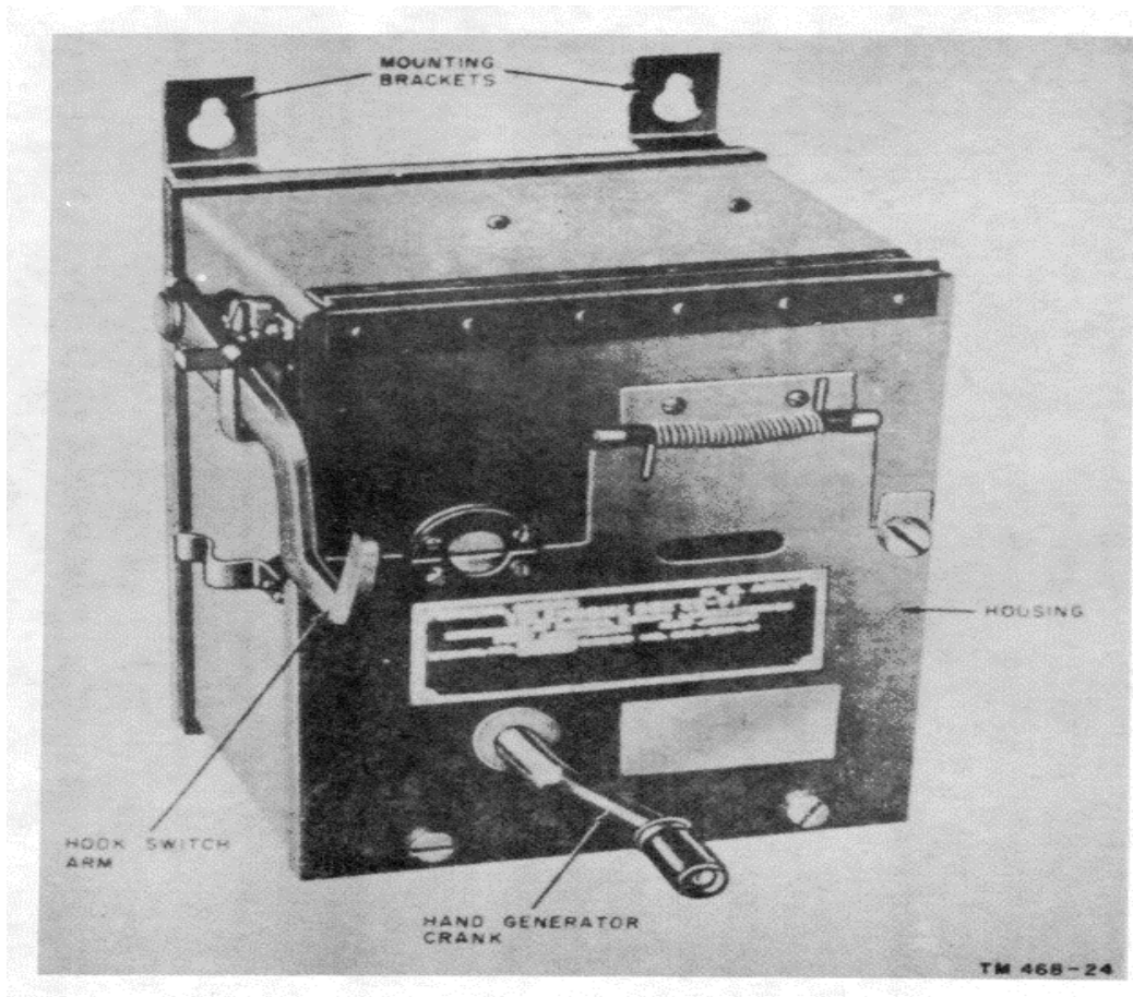
Figure 24. Telephone Box EE-91, common-battery telephone.
