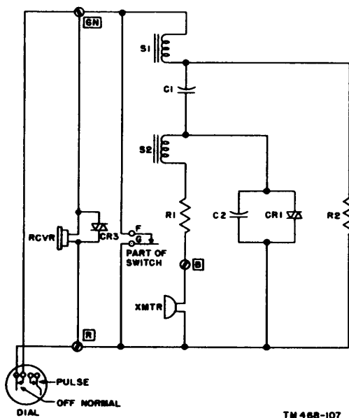
Figure 64. Receiver circuit, dial, schematic.
