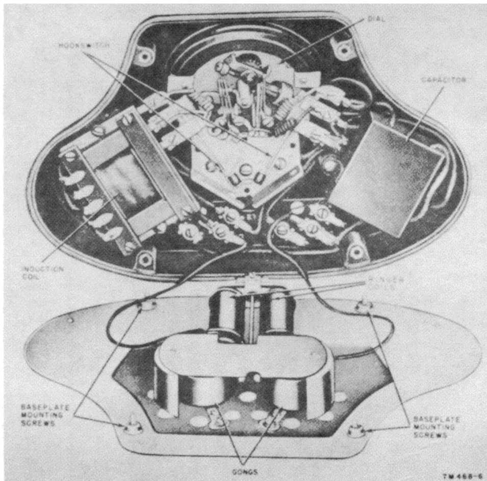
Figure 6. Telephone TA-102/FTC (Kellogg No. 925BAX), arranged for dial operation.
