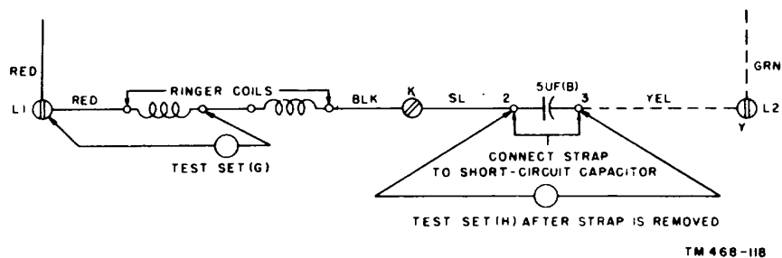
Figure 79. Telephone TP-6-A, tests for short-circuited ringer coil and capacitor B.
