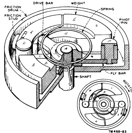
Figure 56. Dial speed governor.
