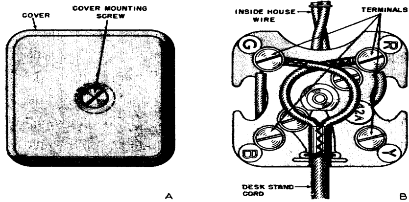
Figure 47. WECO 42-type connecting block.
