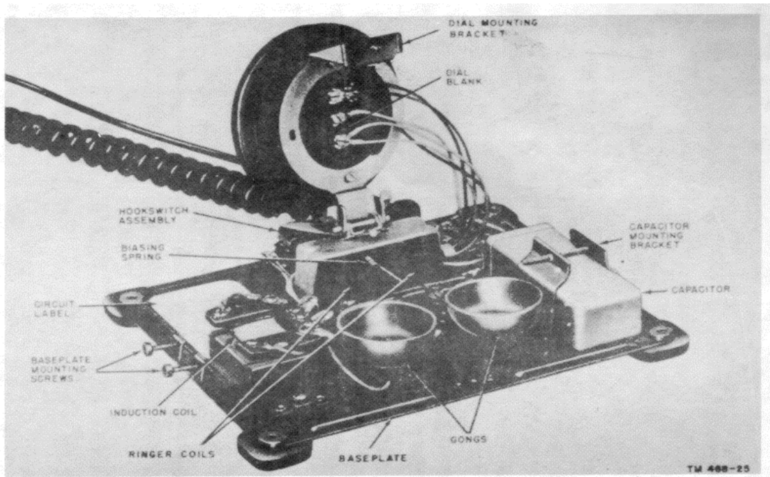
Figure 23. Telephone TA-1661U, with base plate open, showing location of parts.
