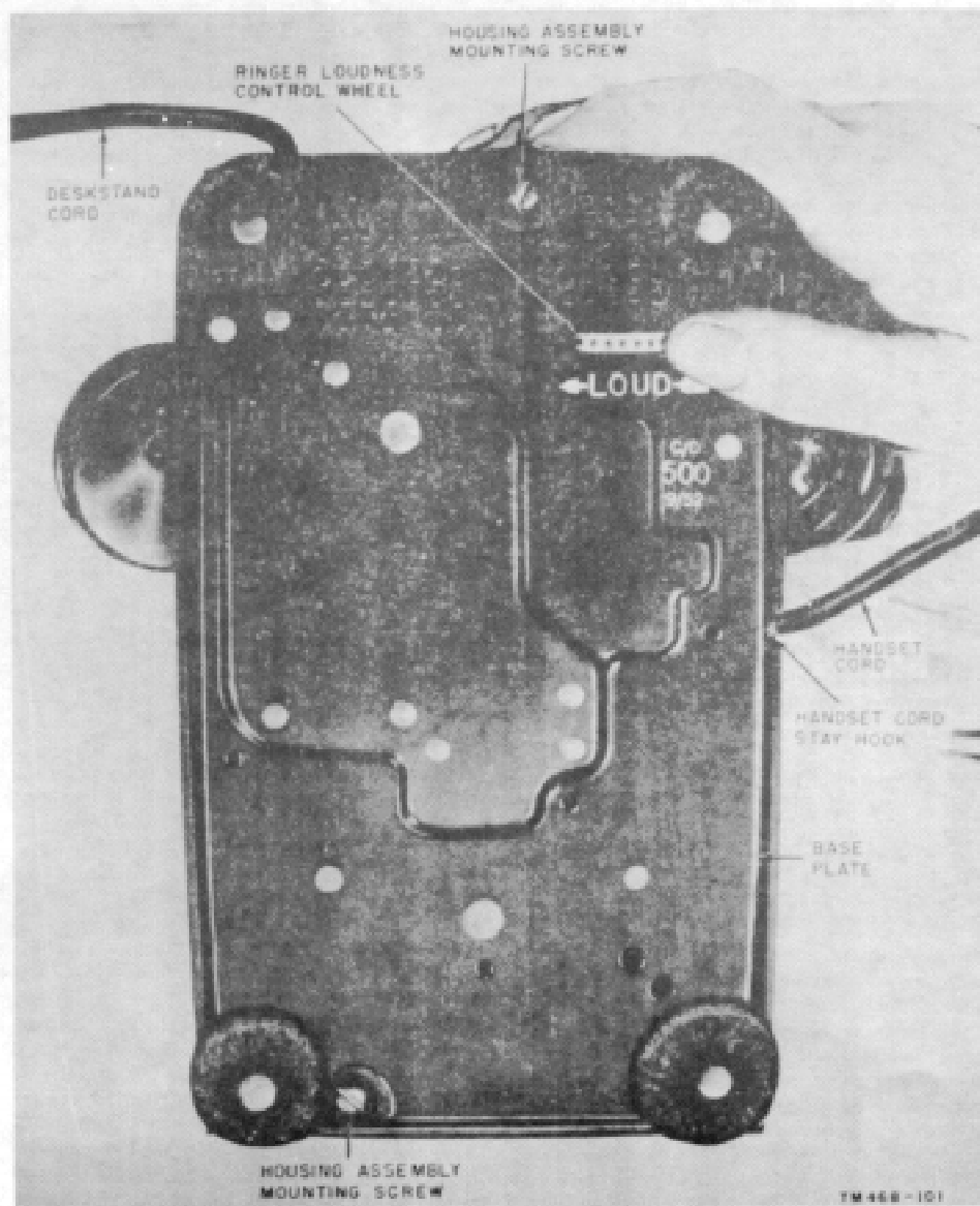
Figure 58. Adjusting the ringer loudness control.
