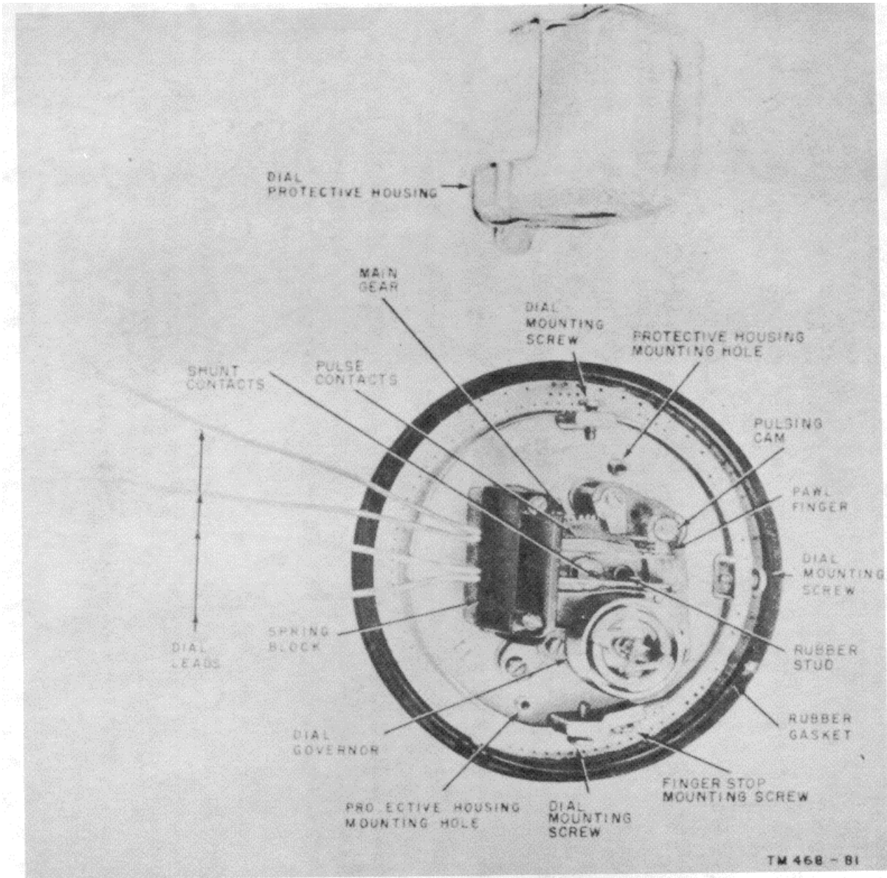
Figure 41. Dial for Telephone Set TA-236/FT, showing mechanism and housing.
