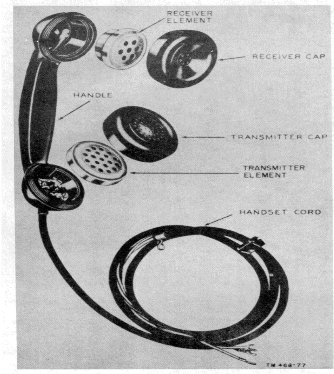
Figure 28. TP-6 or TP-6-A handset, exploded view.
