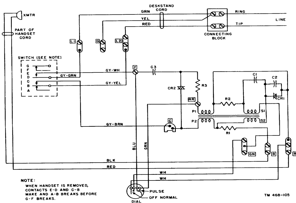
Figure 62. Transmitter circuit, dial, wiring.
