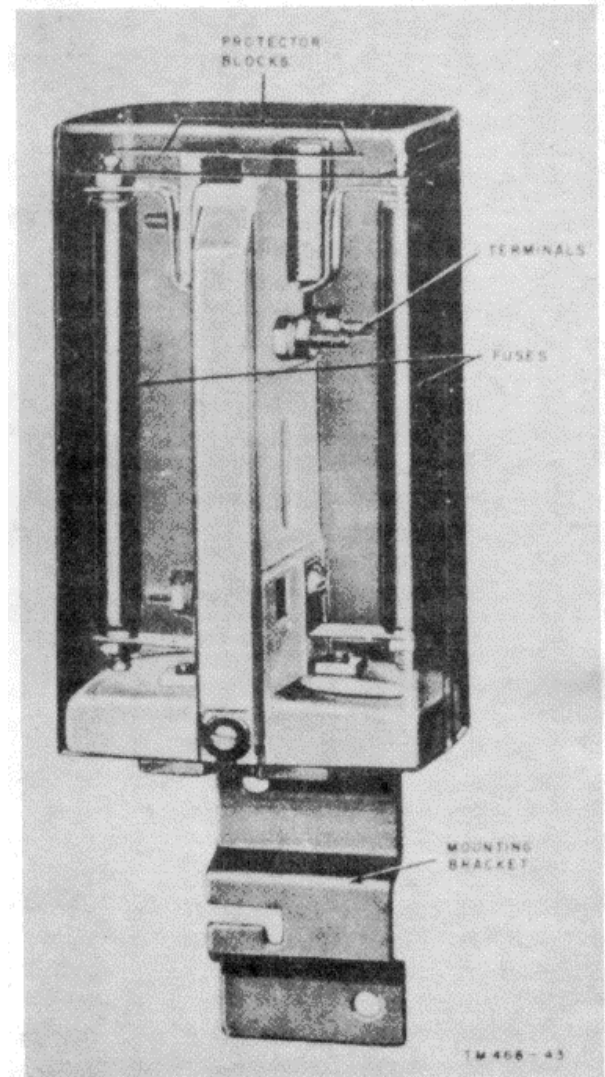
Figure 50. Protector AR-8 (Reliable Electric Co. No. 1000).
