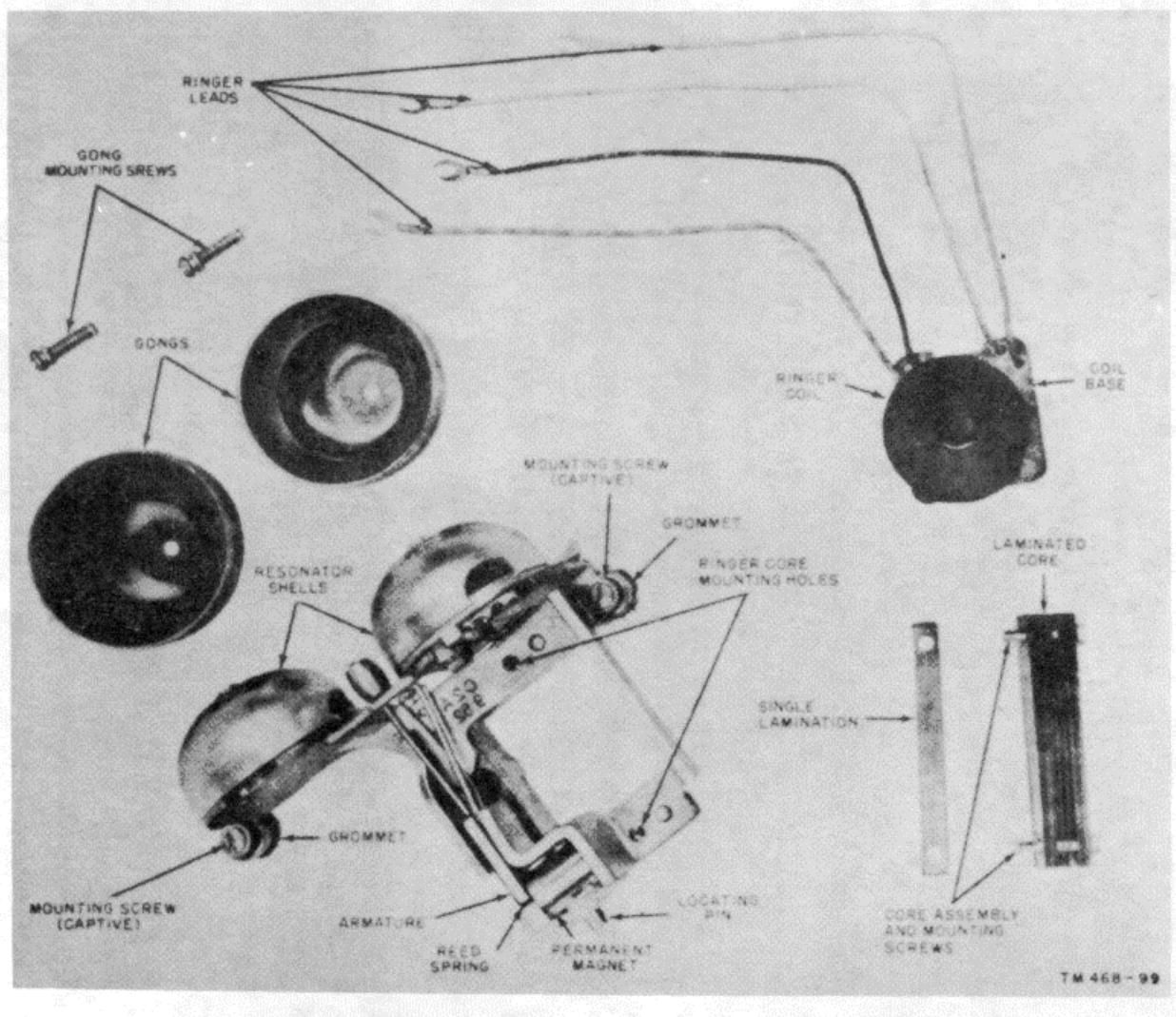
Figure 40. Ringer for Telephone Set TA-236/FT, exploded view.
