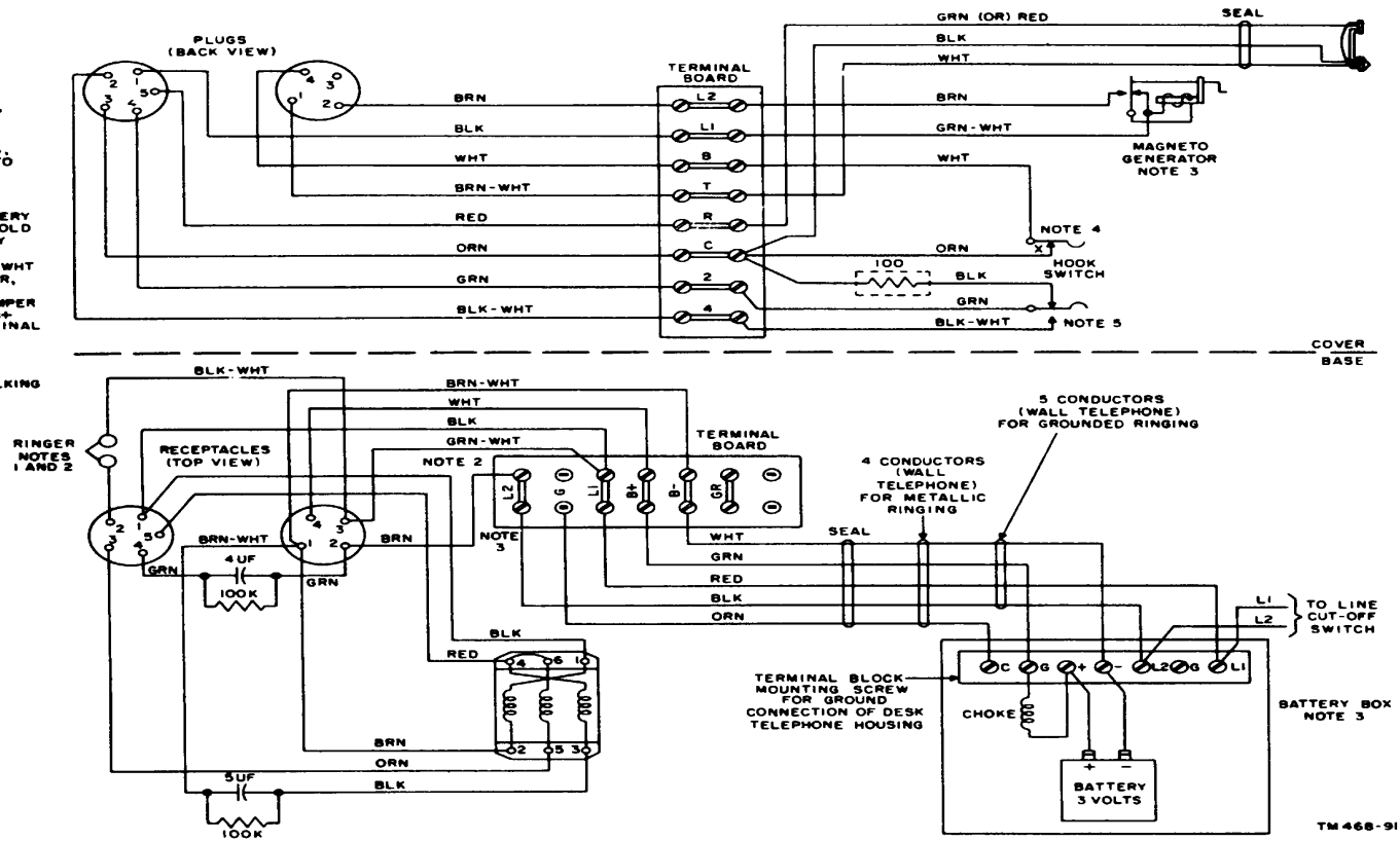
Figure 103. Telephone TA-213/U, wiring diagram.
