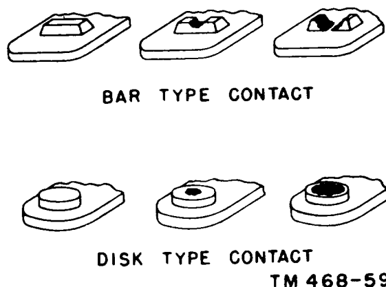
Figure 86. Progressive stages of contact pitting (bar and disk-type contacts).
