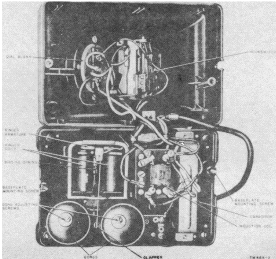
Figure 3. Telephone TP-6, with base plate open
