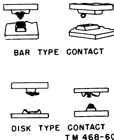
Figure 87. Build-ups and pits on contacts (bar and disk-type contracts)
