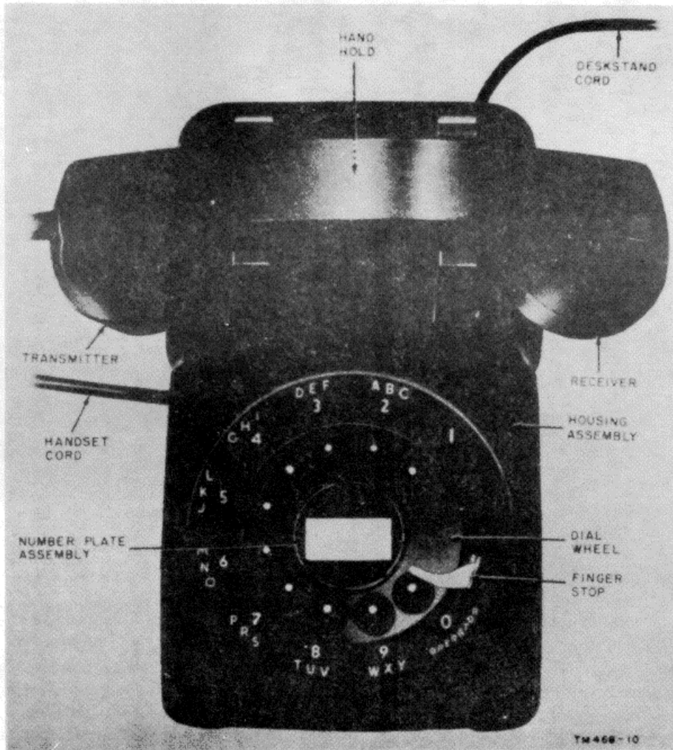
Figure 33. Telephone Set TA-236IFT, arranged for dial operation.
