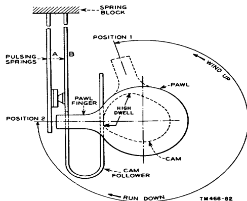
Figure 55. Dial pulsing mechanism.
