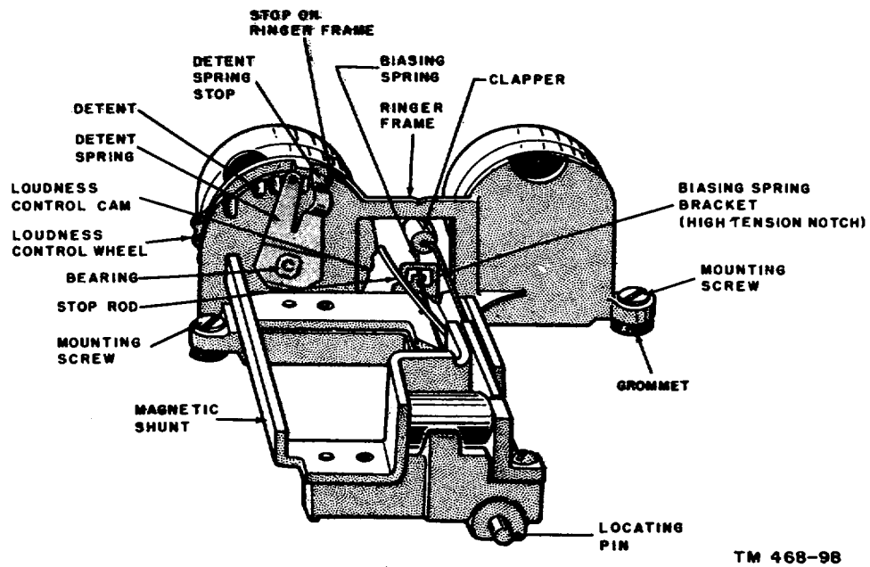
Figure 39. Ringer frame and permanently attached elements.
