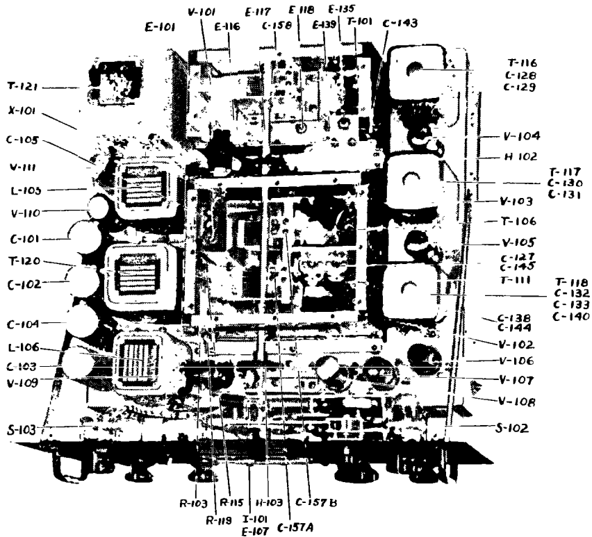
FIG. 2.13 TOP VIEW RADIO RECEIVER CHASSIS
