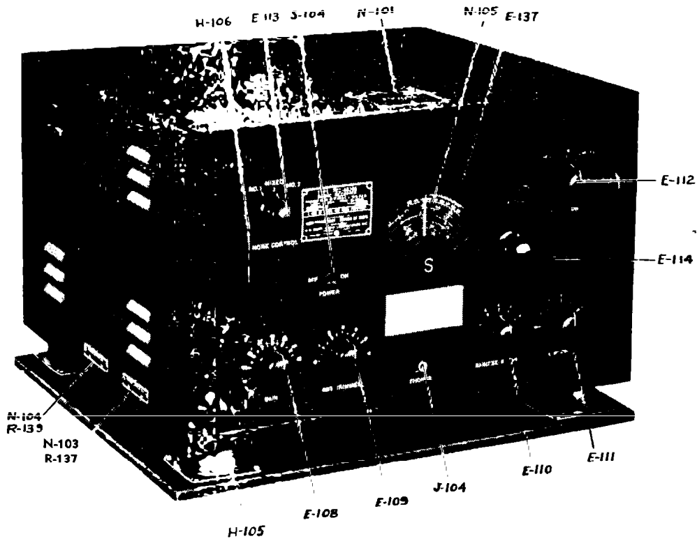
FIG. 1 LEFT FRONT OBLIQUE VIEW, RADIO RECEIVER
