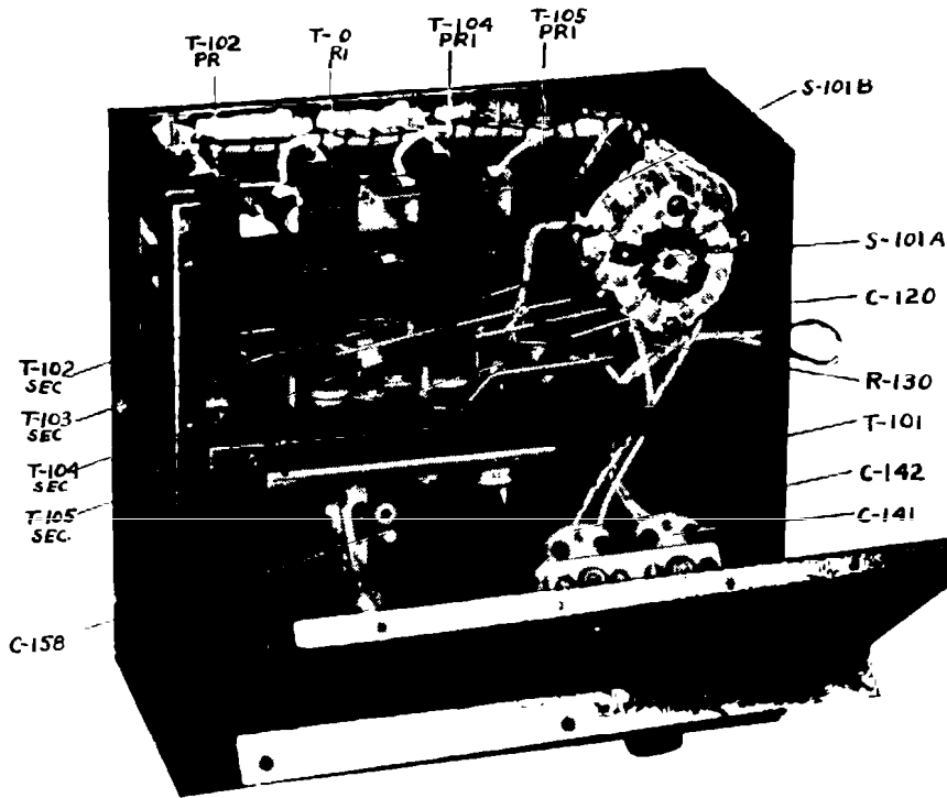
FIG. 2.18 LEFT OBLIQUE INVERTED VIEW, ANTENNA COMPARTMENT
