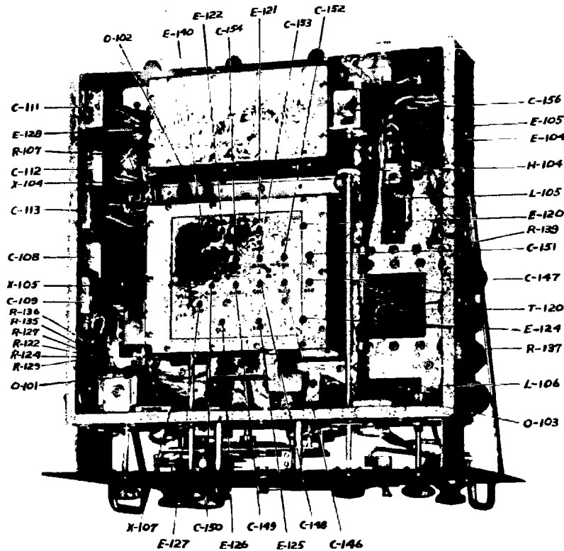
FIG. 2.111 LEFT BOTTOM OBLIQUE VIEW, RADIO RECEIVER CHASSIS
