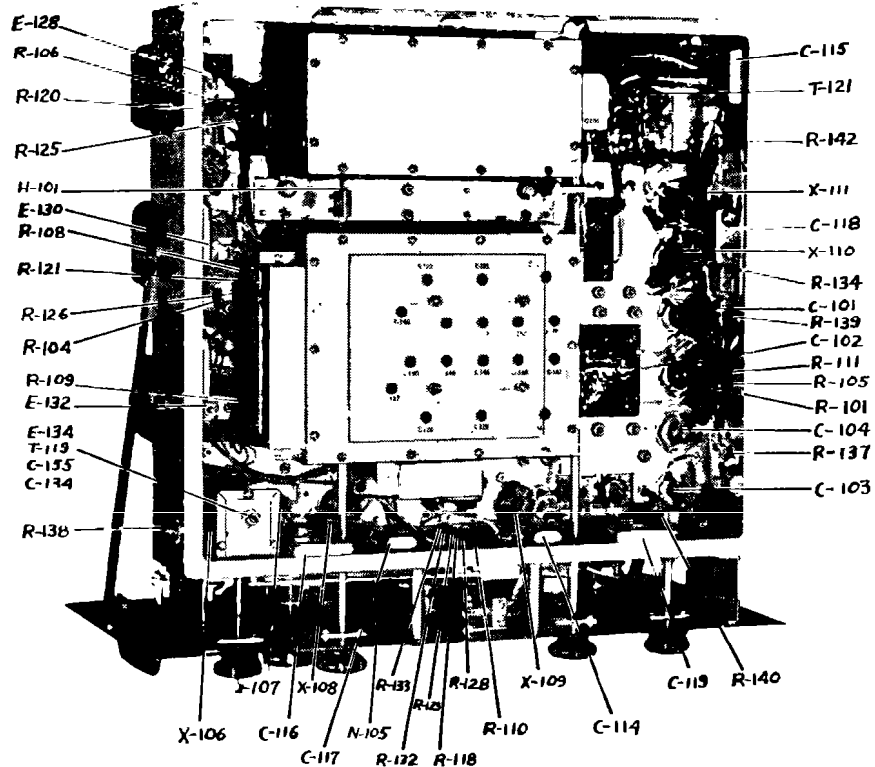
FIG. 2.15 RIGHT BOTTOM OBLIQUE VIEW, RADIO RECEIVER CHASSIS
