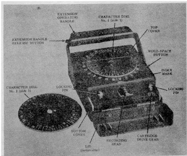
Figure 1-2. CO/B-8 Coder.
