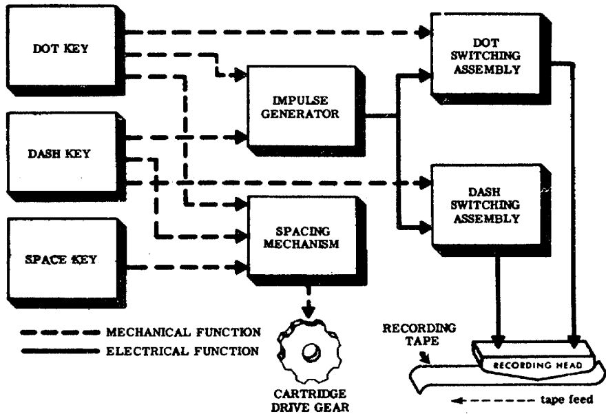
Figure 3-5. CO-3B Coder functional block diagram.
