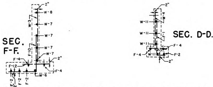
FIGURE 9.—Standard short and midrange multitarget butts with integral target pit and storeroom, material tabulation.
