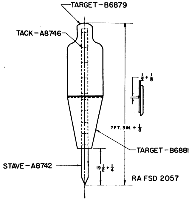
FIGURE 62.—Target M, M1913, complete.
