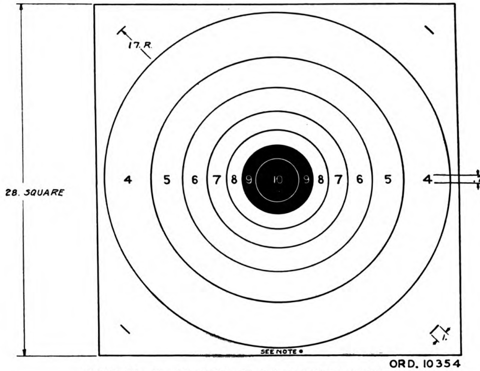
FIGURE 66.—Target, pistol, 25-yard (standard American).
