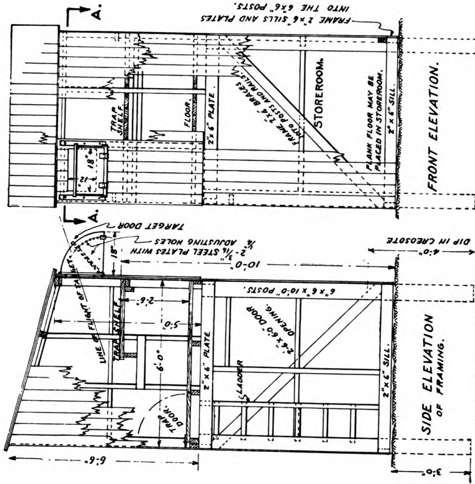
FIGURE 46.—Skeet range, details of structures required.
