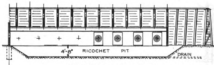
SECTION ON C-C
