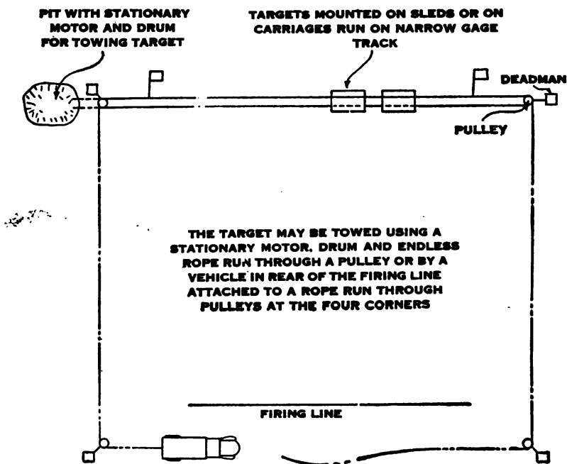
FIGURE 35.—Range for caliber .30 moving field target.
