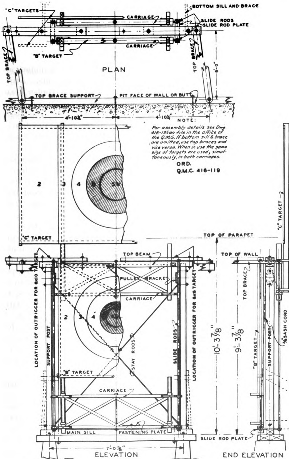
FIGURE 56.—Standard combination sliding target frame support, assembly.
