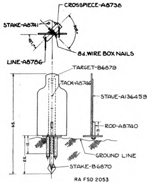
FIGURE 54.—Target, bobbing, M1913.
