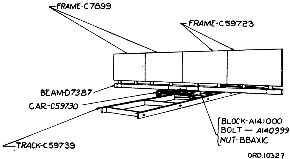
FIGURE 83.—Target, rolling, machine-gun, complete.
