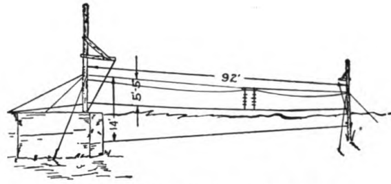
FIGURE 21.—Horizontal target.
