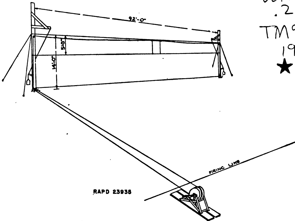
FIGURE 21.—Horizontal target.
