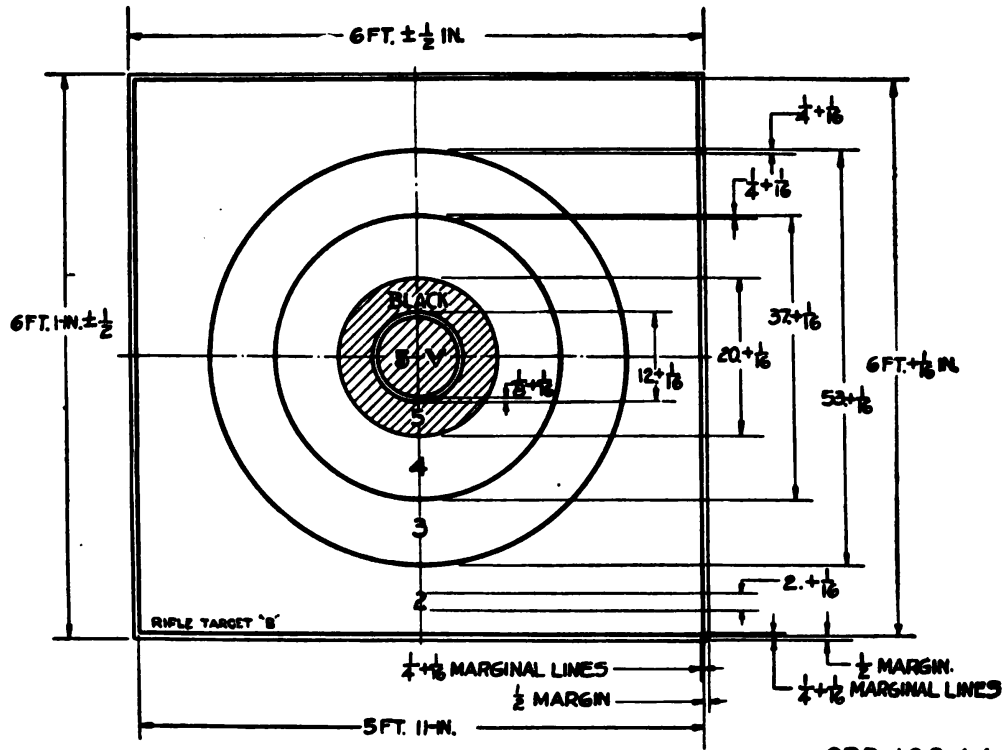
FIGURE 70.—Target, rifle, B.
