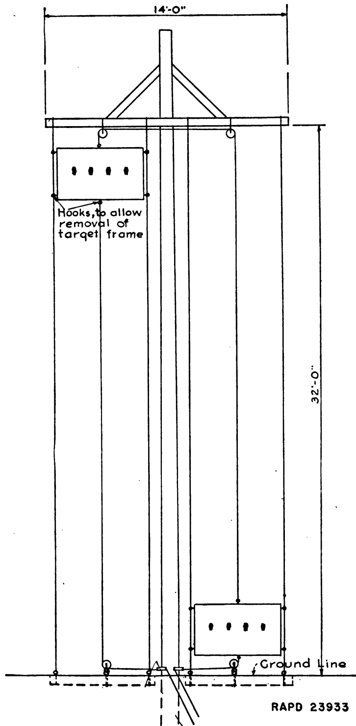
FIGURE 23½.—Parachute target.
