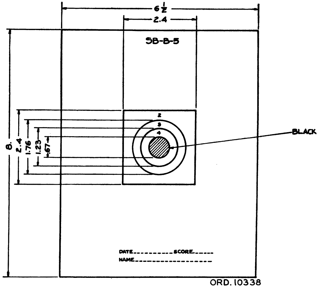
FIGURE 78.—Target, rifle, SB-B-5.
